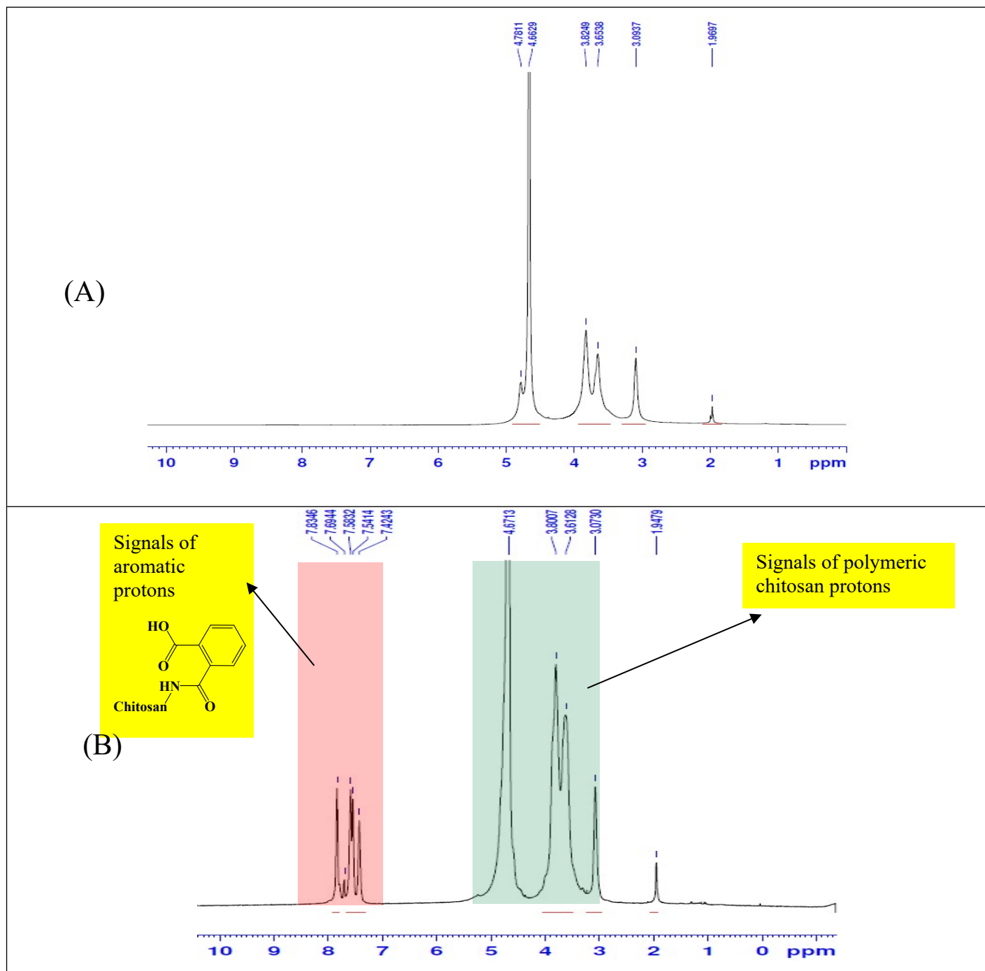
Figure S5 ^1\text{H} NMR spectrums of (A) chitosan, (B) chitosan phthalate.
