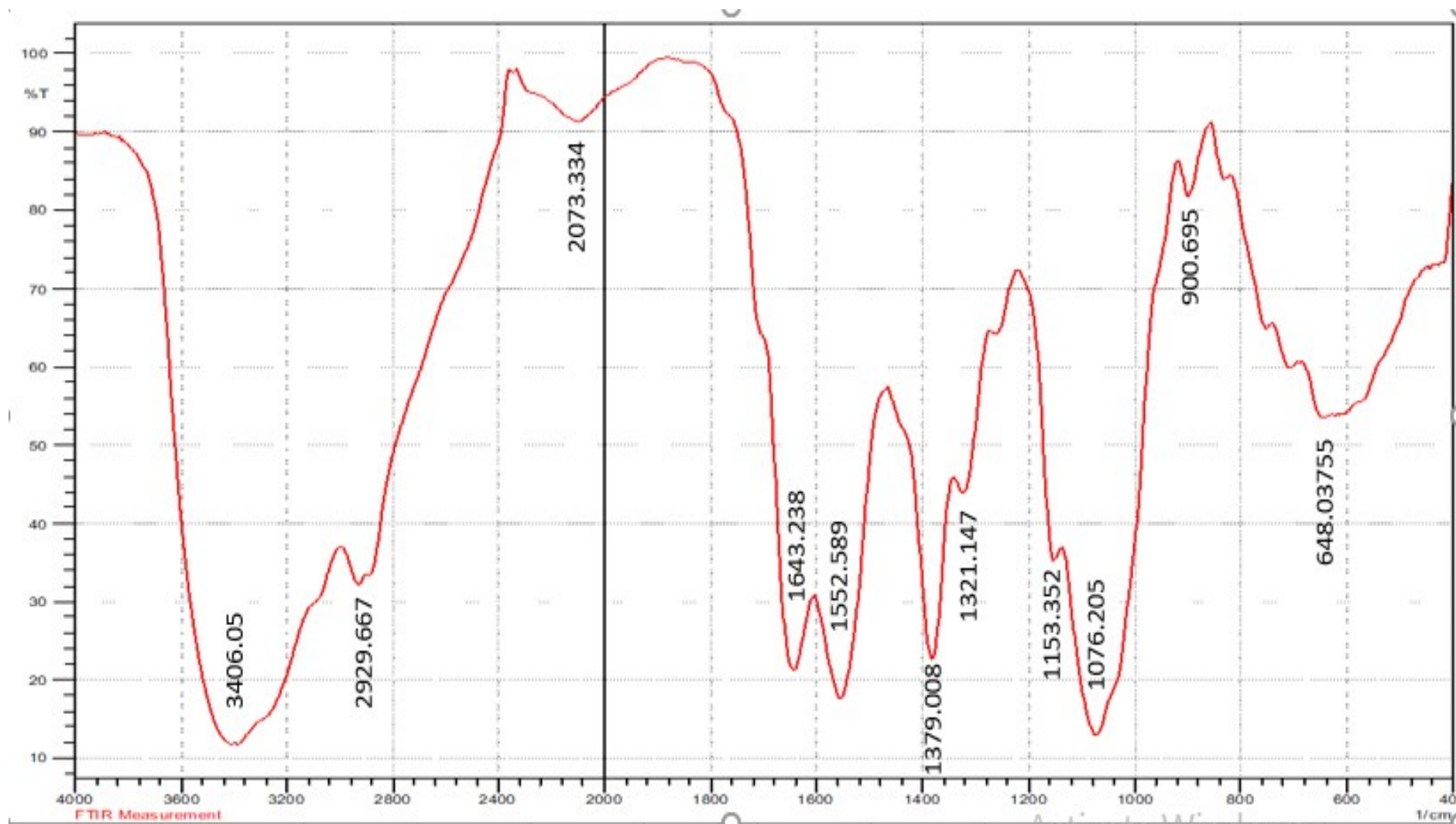
Figure S2: Infrared of Chitosan Phthalate (CP).
