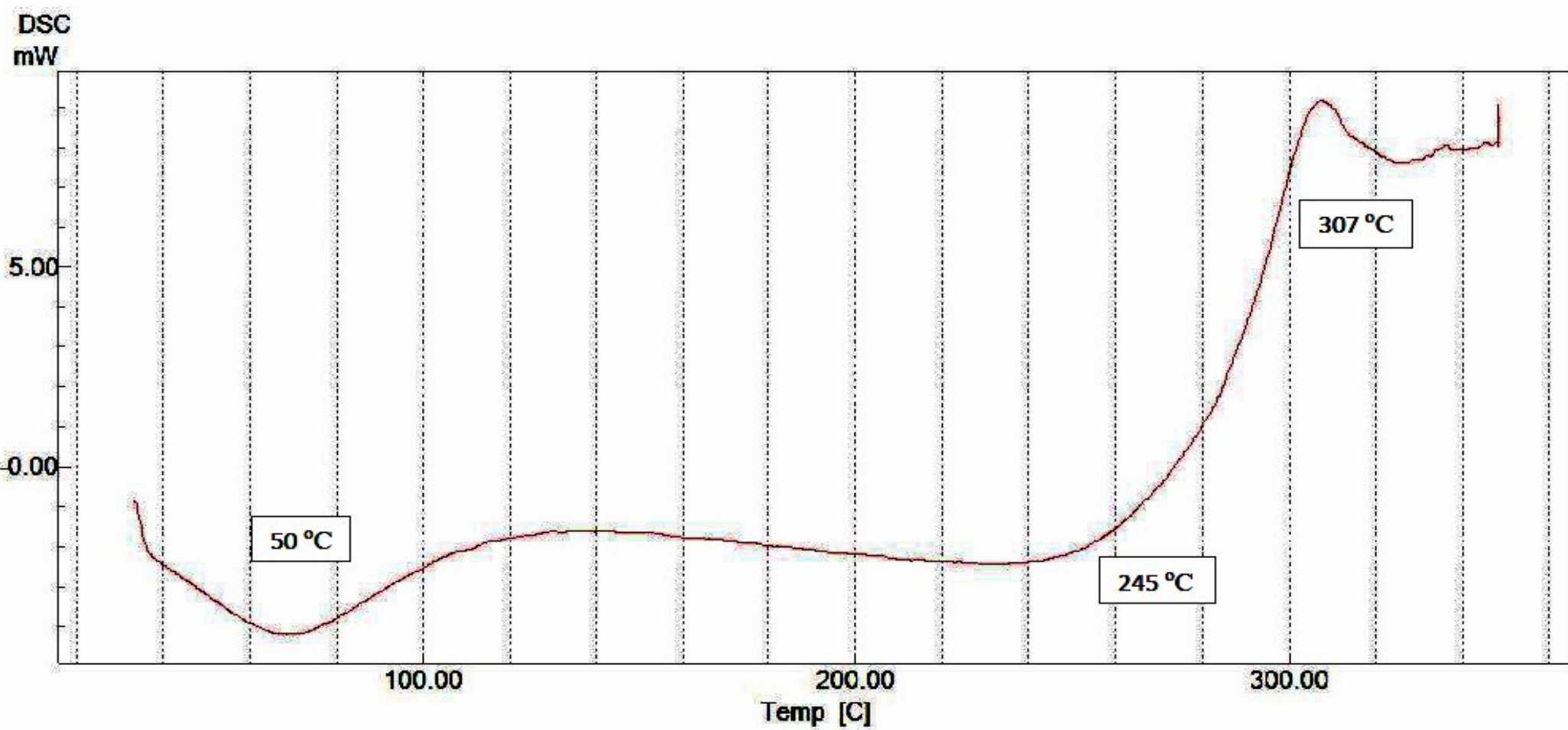
Figure S3: DSC of Chitosan (C).
