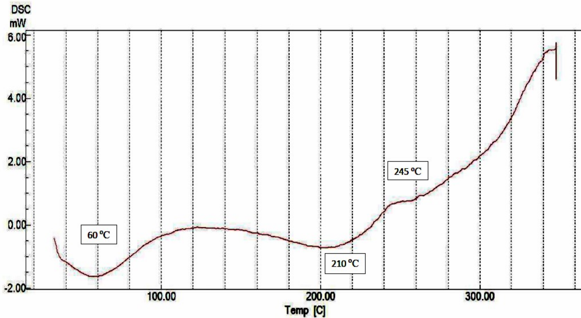
Figure S4: DSC of Chitosan Phthalate (CP)
