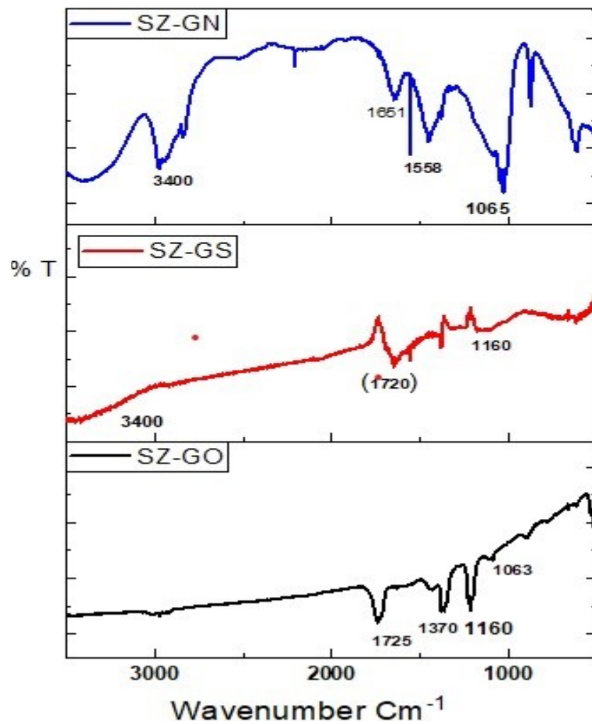
S2: FTIR spectra of GO (SZ-GO), S-GO (SZ-GS) and N-GO (SZ-GN)
