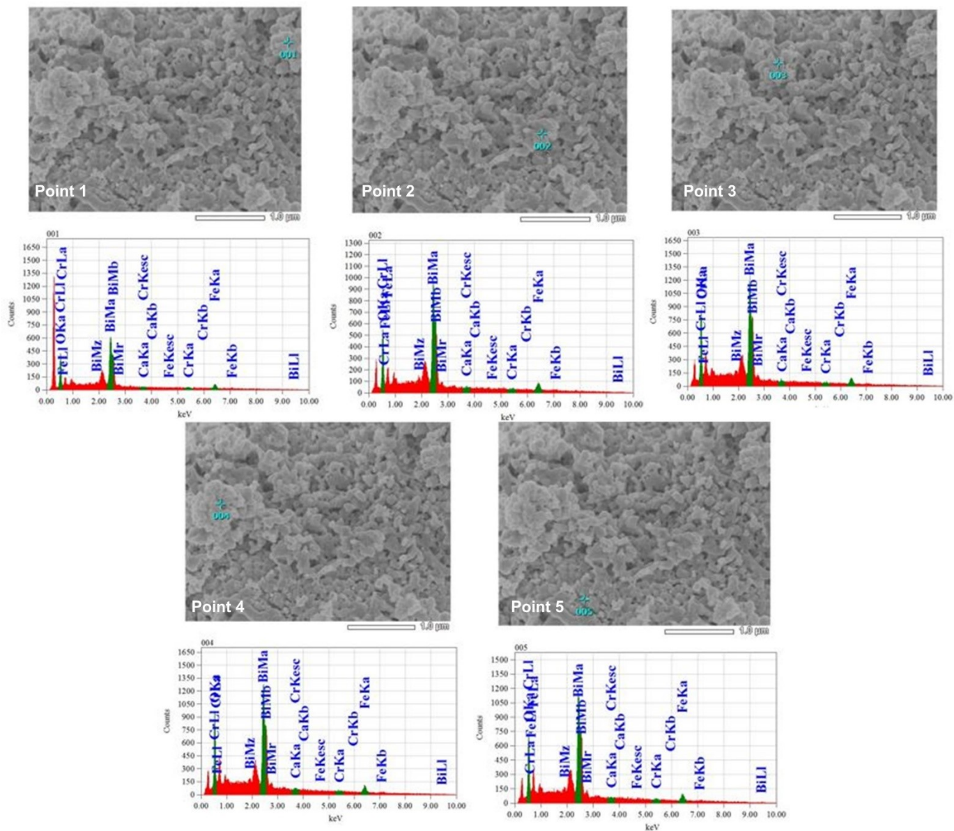
Figure S5: EDS spectra from multiple points of the BCFOCr5 sample
