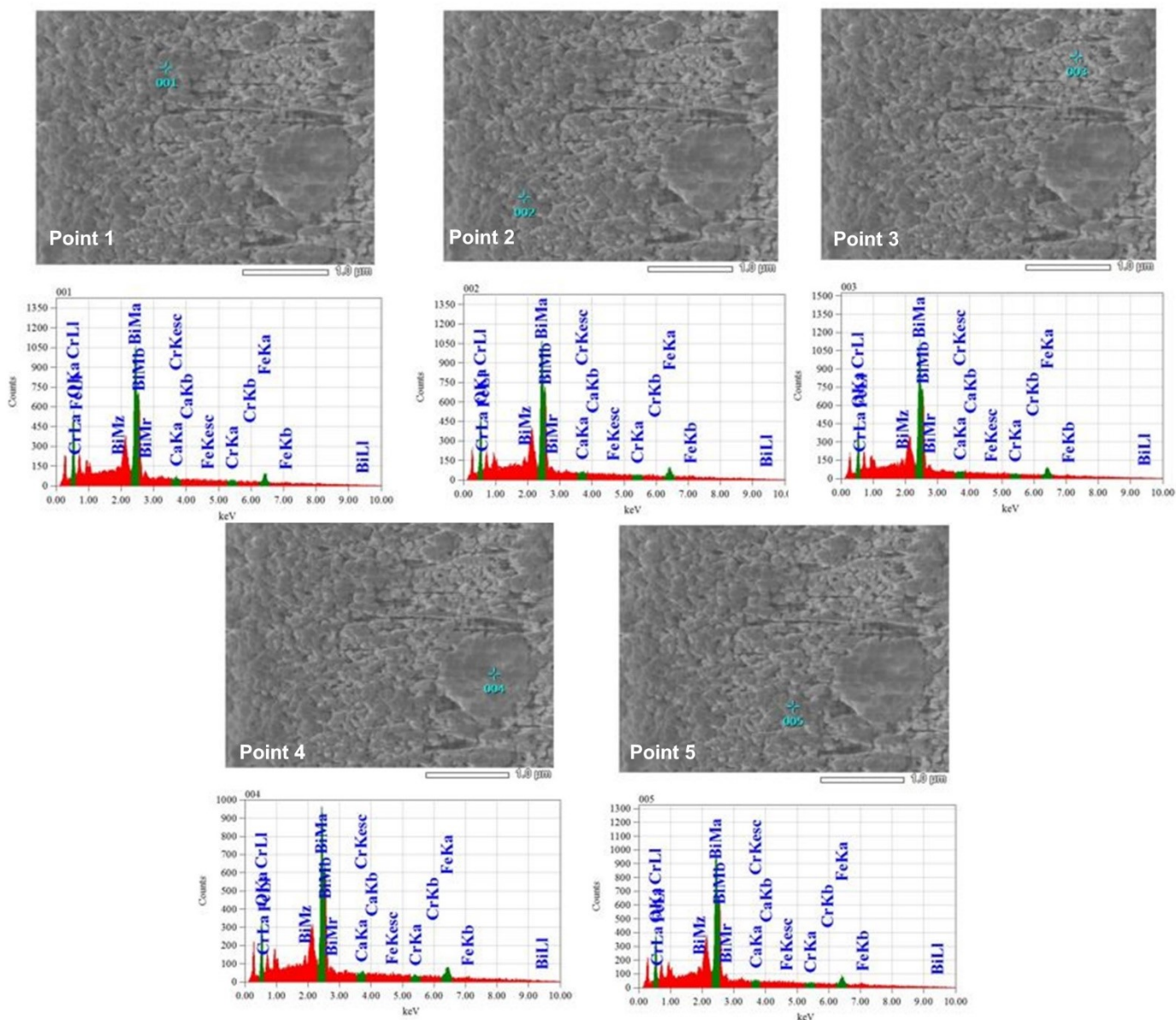
Figure S4: EDS spectra from multiple points of the BCFOCr 3 sample
