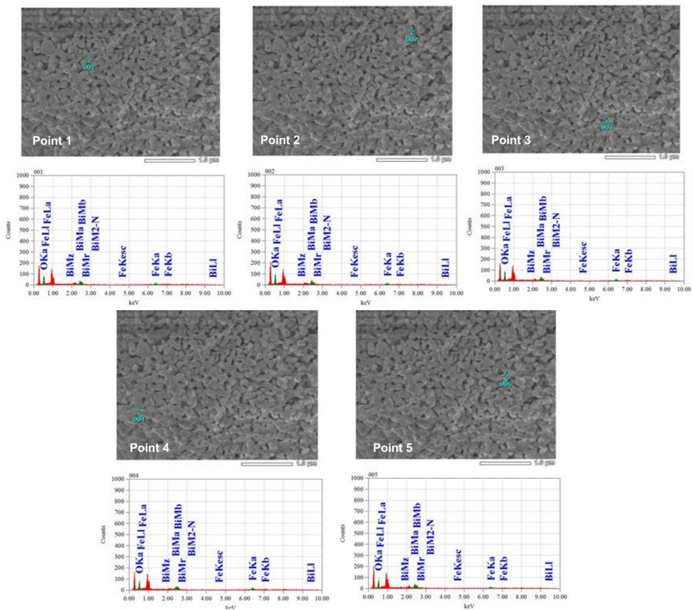
Figure S1: EDS spectra from multiple points of the BFO sample
