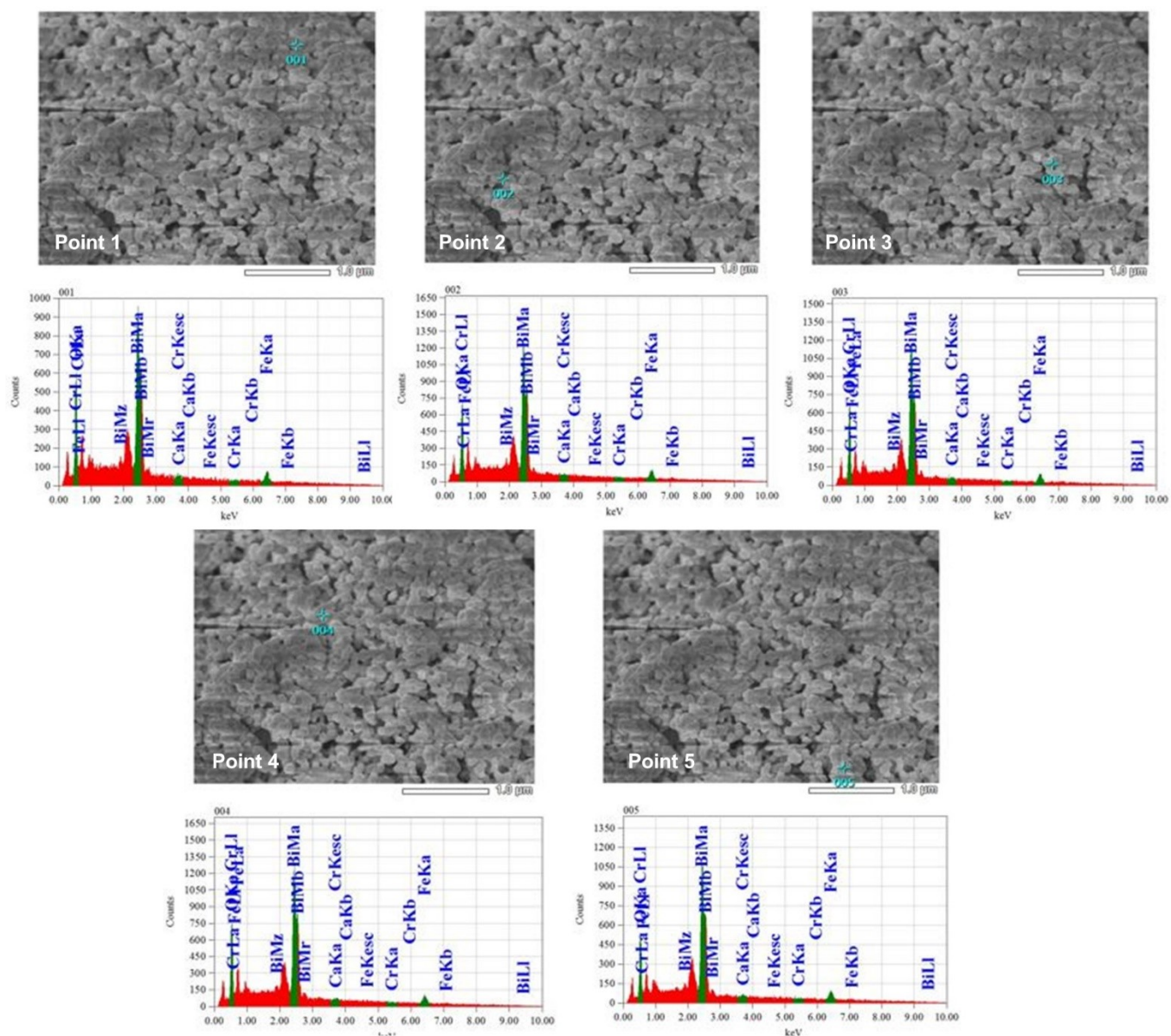
Figure S3: EDS spectra from multiple points of the BCFOCr1 sample
