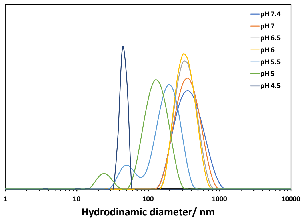
Figure S 2. DLS intensity-average particle size distributions of PDMA 50 -co-PDPA 200 recorded at different pH.
