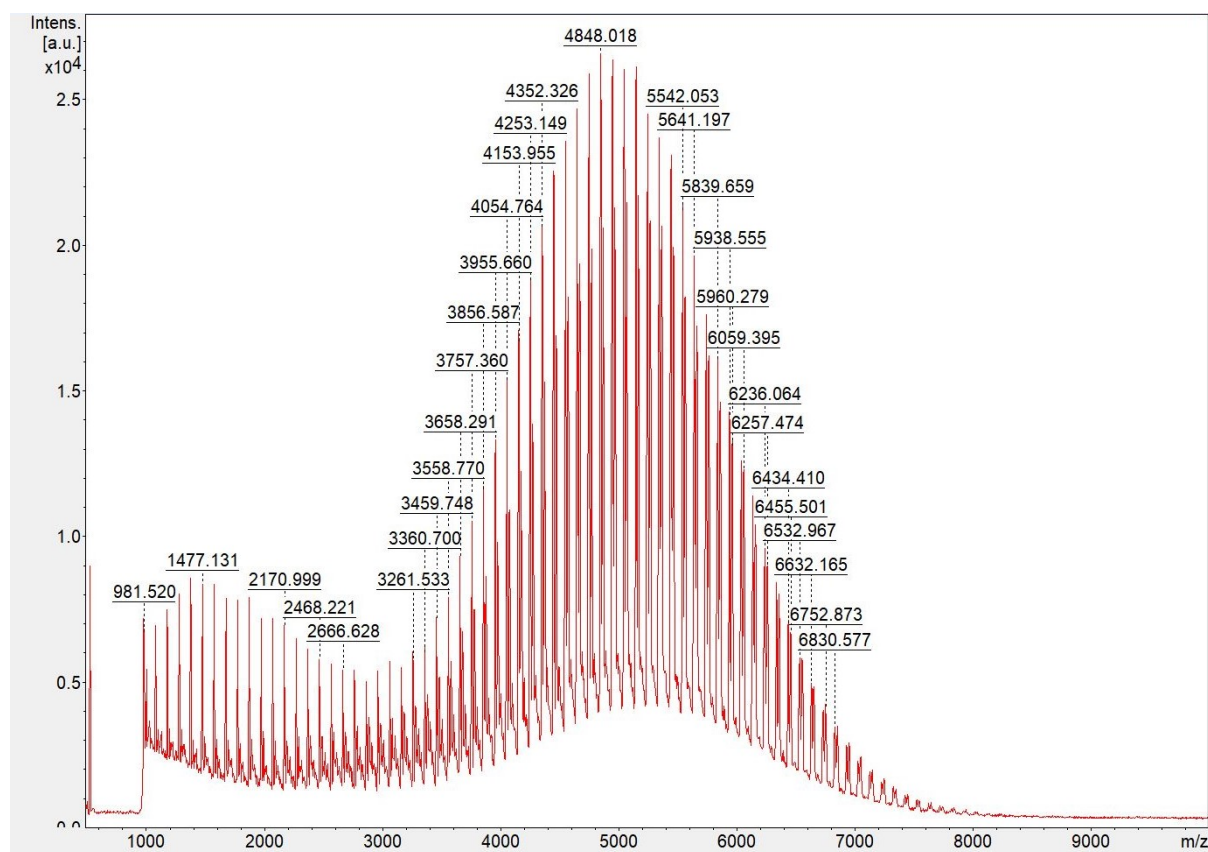
Figure S 1. MALDI-TOF of PDMA macro-CTA
