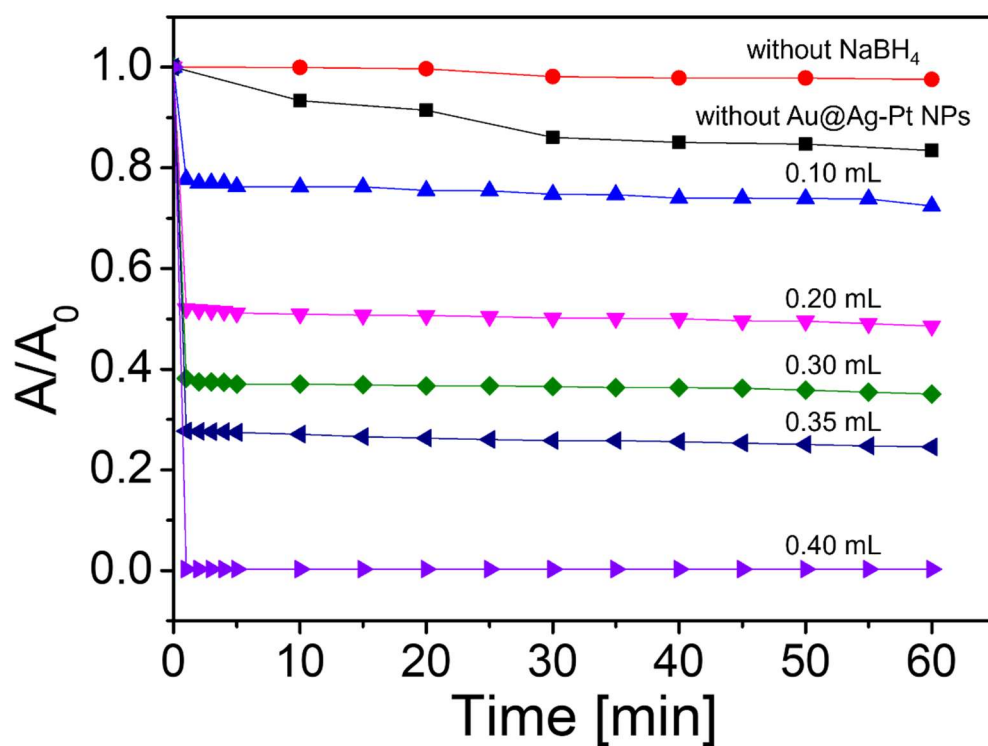
Fig. S2. Time-dependent absorbance variation of methylene blue (MB) during the reduction reaction, where A is the absorbance at 664 nm and A_0 is the initial absorbance.
