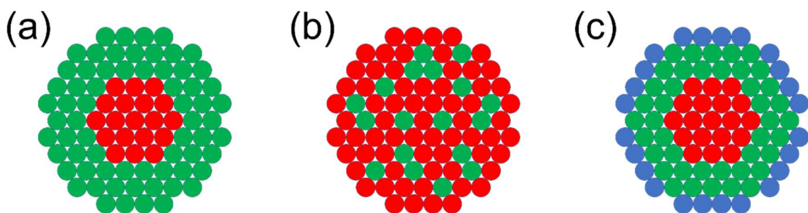
Fig. S1. Schematic diagram of (a) core-shell, (b) alloy, and (c) core@multi-shell structures, where each color represents a different element.
