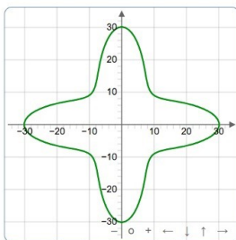
Young's modulus in (yz) plane
