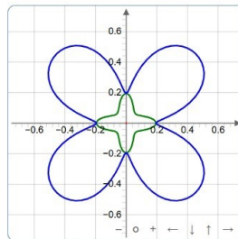
Poisson's ratio in (yz) plane
