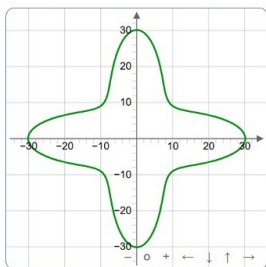
Young's modulus in (xz) plane
