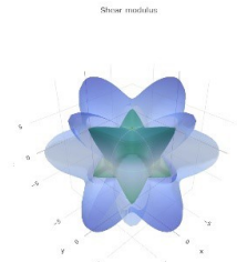
Shear modulus
