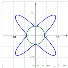
Shear modulus in (xy) plane
