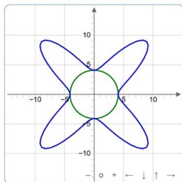
Shear modulus in (xz) plane
