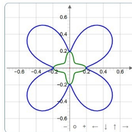
Poisson's ratio in (xz) plane
