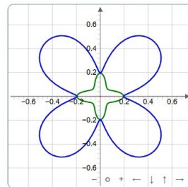
Poisson's ratio in (xy) plane
