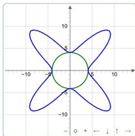
Shear modulus in (yz) plane
