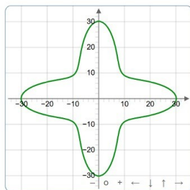
Young's modulus in (xy) plane
