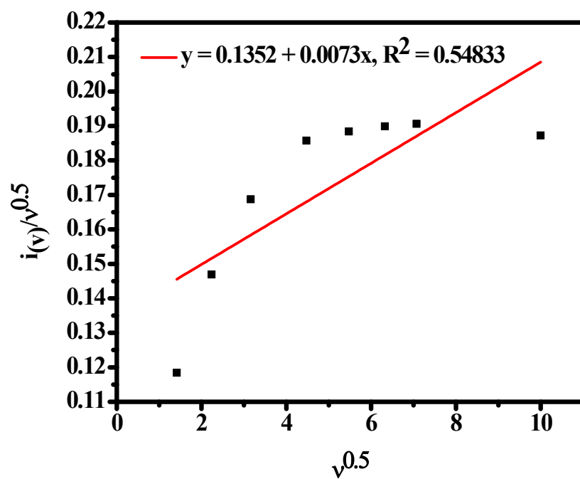
Fig. SI-4 Plot of \frac{i(v)}{v^{0.5}} versus v^{0.5} for the determination of capacitive and diffusion contributions
