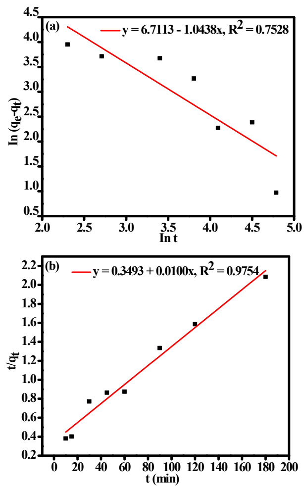
Fig. SI-3. (a) pseudo-first-order kinetics and (b) pseudo-second-order kinetics
