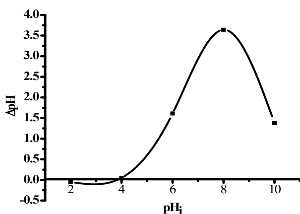
Fig. SI-1. pHpzc of H-WSAC
