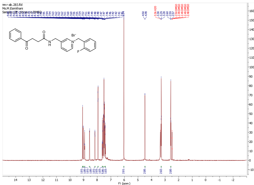
Figure S 3. 1 HNMR spectra of compound 7b.
