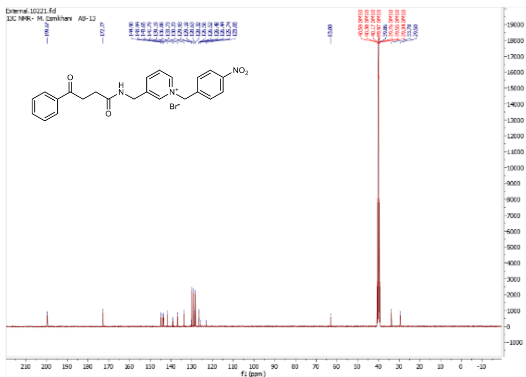
Figure S 22. 13 C NMR spectra of compound 7j.
