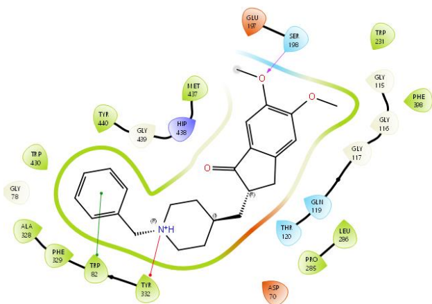
Figure S 36. 2D interaction of donepezil in the active site of BCHE
