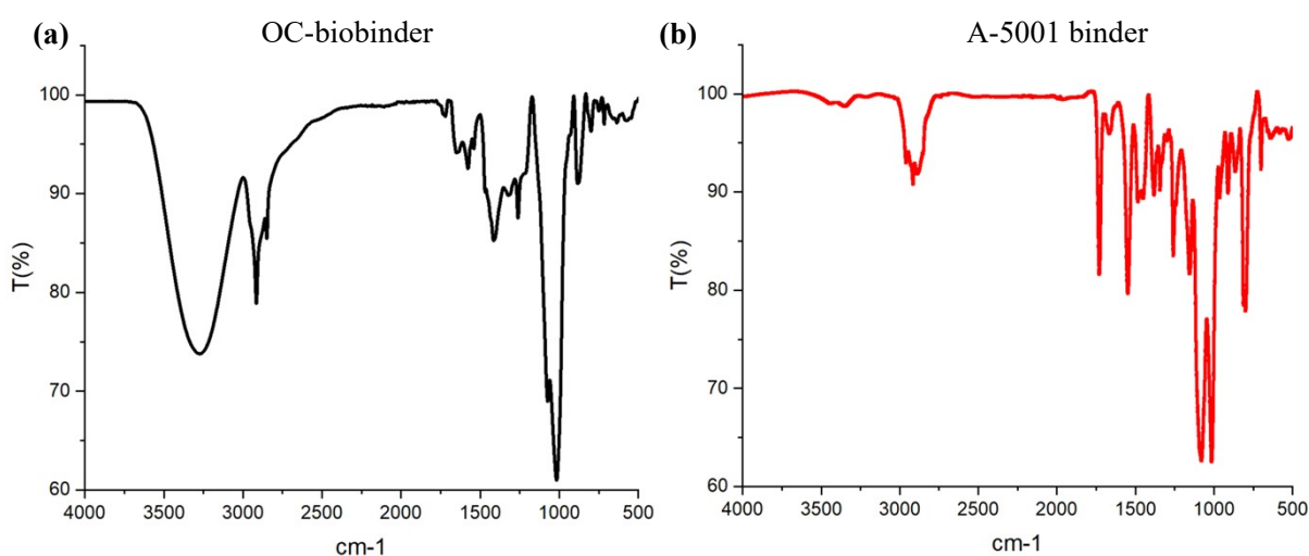
Figure S1. ATR-FTIR curve of the (a) OC-biobinder, and (b) ATR-FTIR curve of A-5001 binder.
