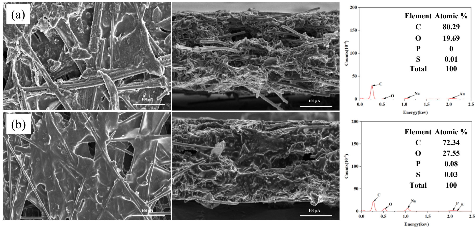
Fig. S1 FE-SEM images and EDS mappings of the tops and cross sections of (a) CP with one layer of LOx-PEGDGE, and (b) CP with four layers of LOx-PEGDGE (optimized electrode) after five repeated cycles.
