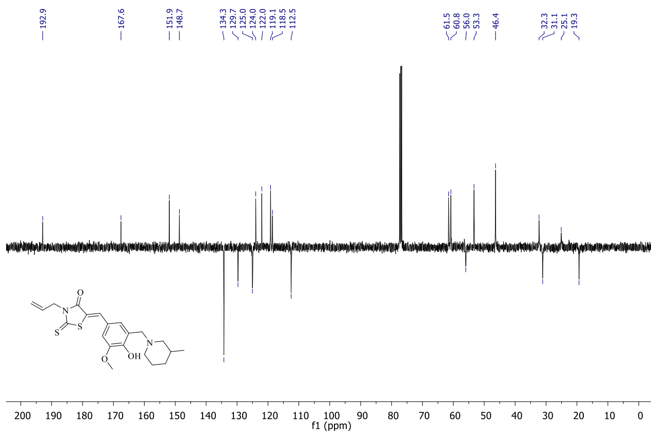
Figure S18. 13 C NMR Spectrum of Compound 5
