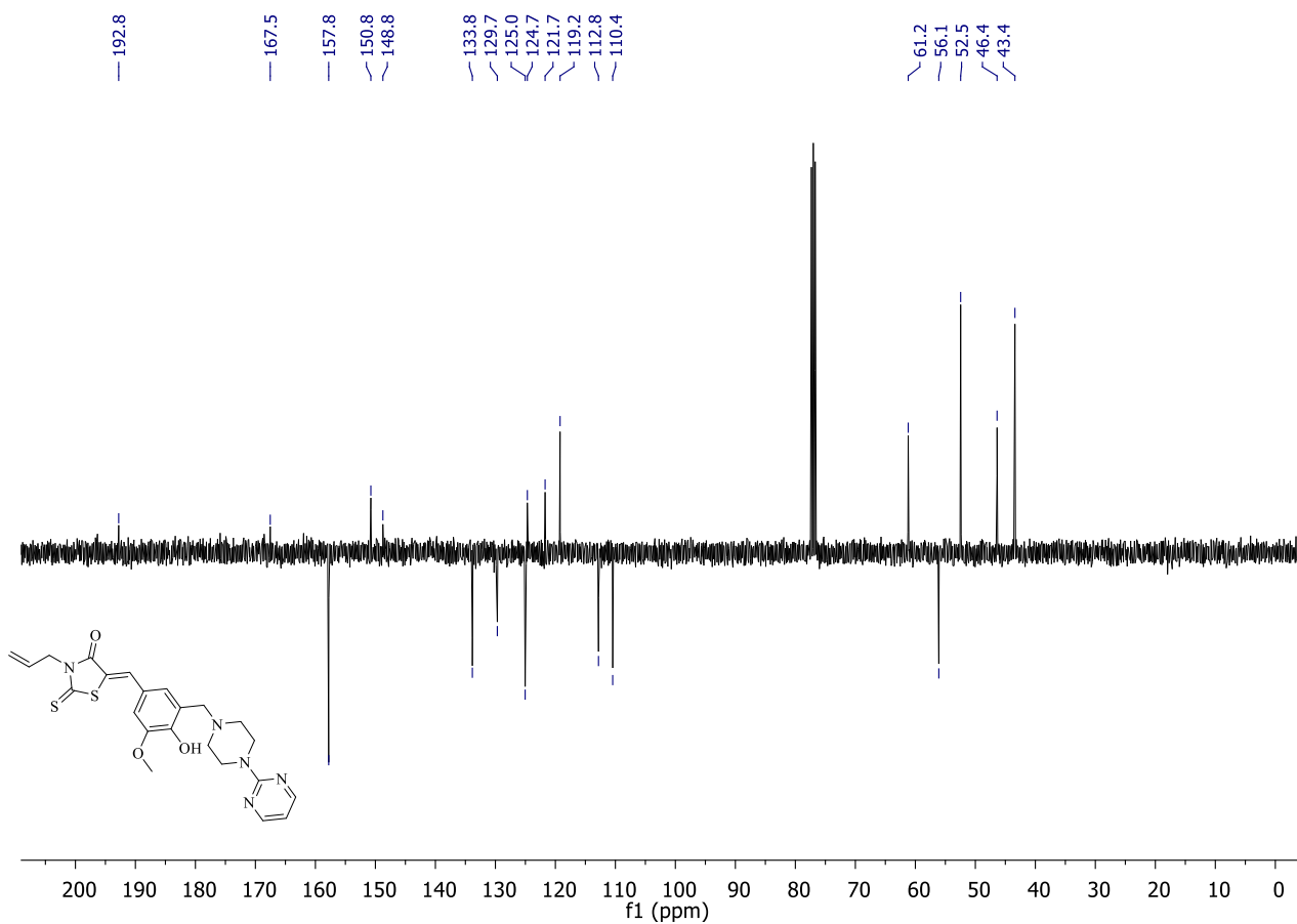
Figure S26. 13 C NMR Spectrum of Compound 7
