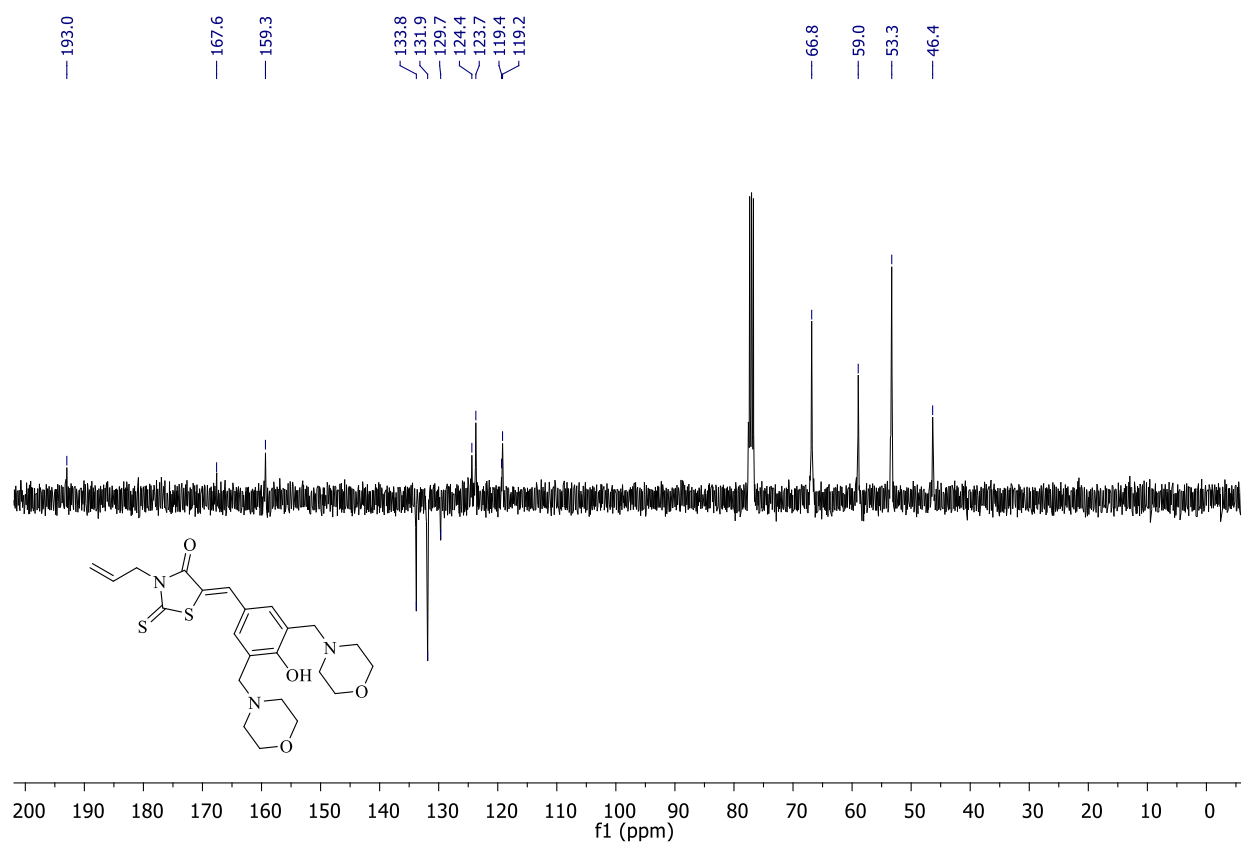
Figure S50. 13 C NMR Spectrum of Compound 13
