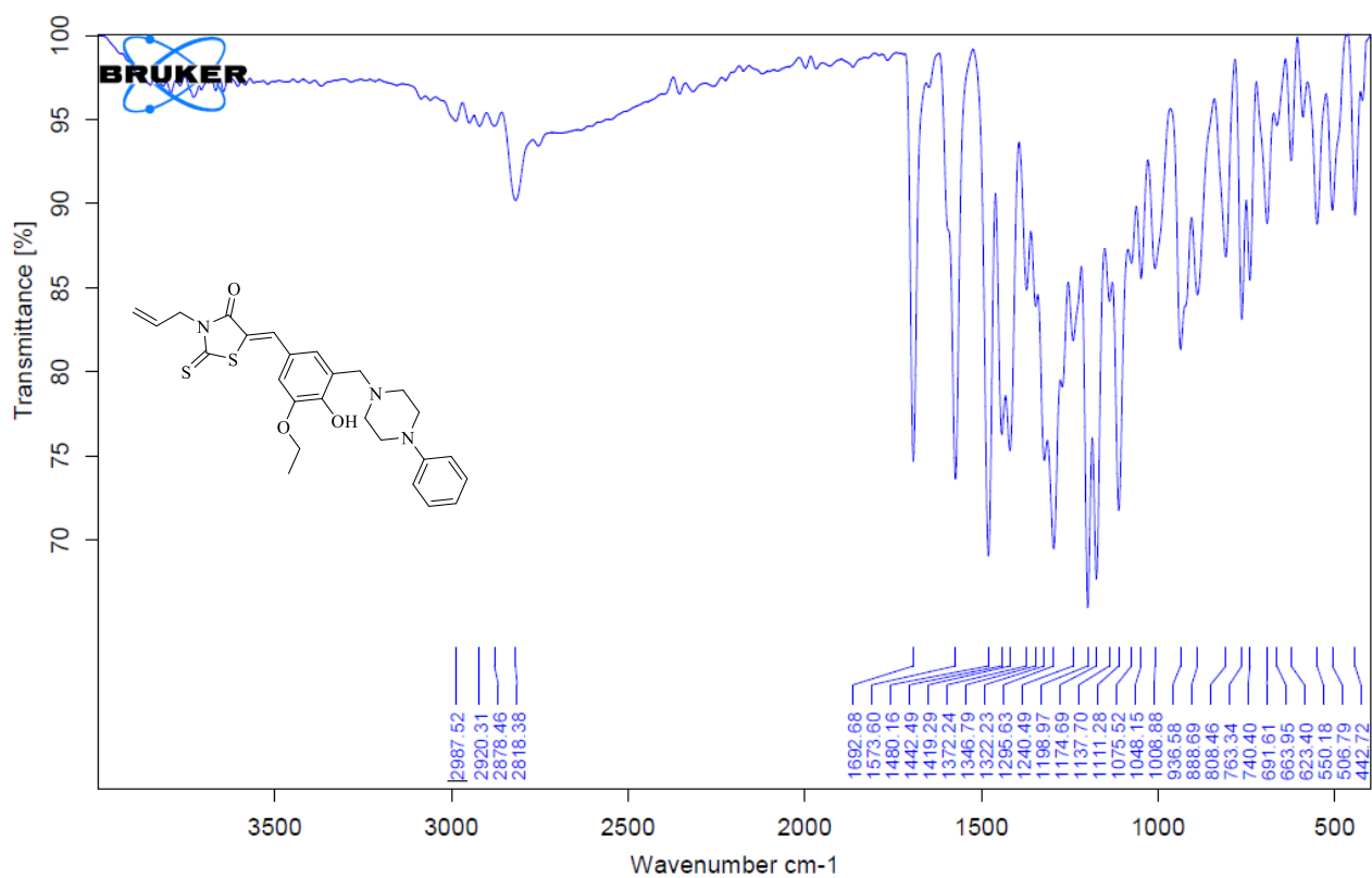
Figure S39. FTIR Spectrum of Compound 10
