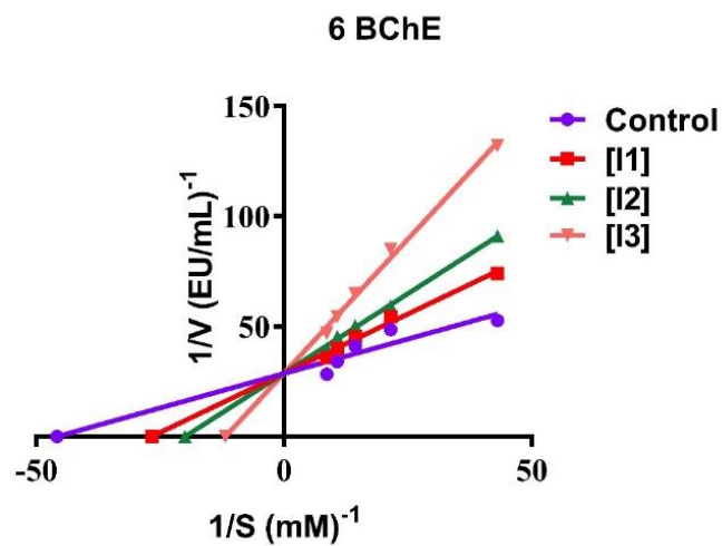
Figure S71. Lineweaver-Burk plots of compound 6 for BChE
