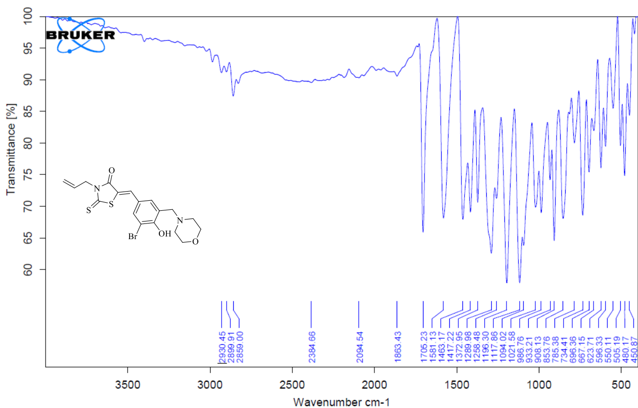
Figure S47. FTIR Spectrum of Compound 12
