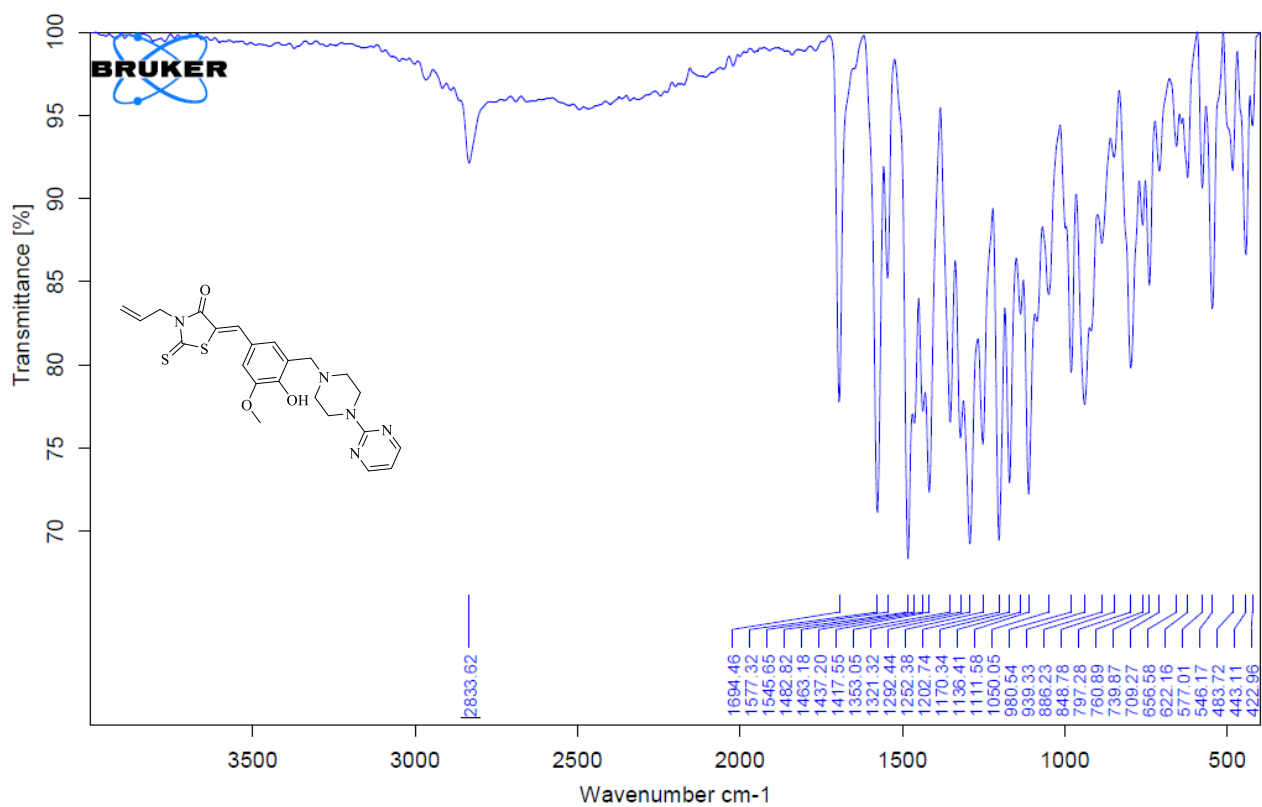
Figure S27. FTIR Spectrum of Compound 7
