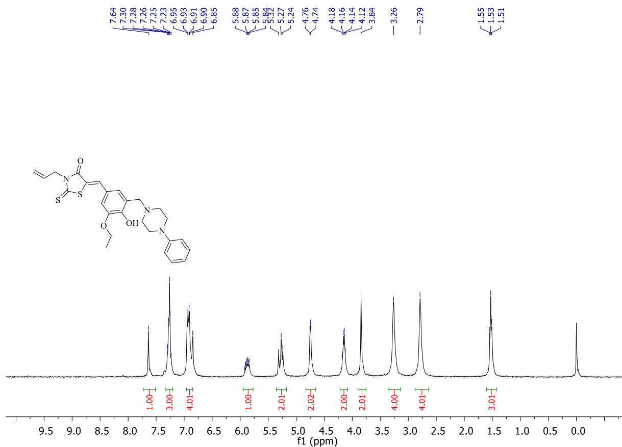
Figure S37. 1 H NMR Spectrum of Compound 10
