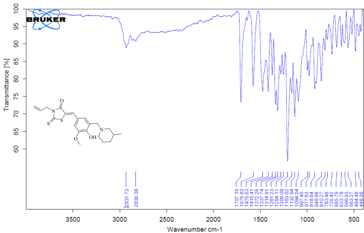
Figure S19. FTIR Spectrum of Compound 5
