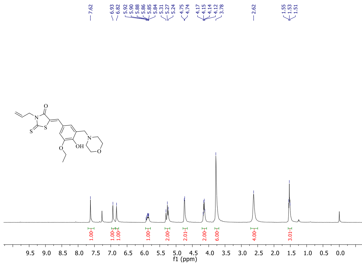
Figure S29. 1 H NMR Spectrum of Compound 8
