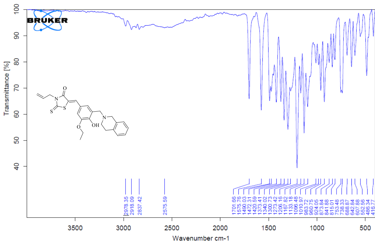
Figure S43. FTIR Spectrum of Compound 11
