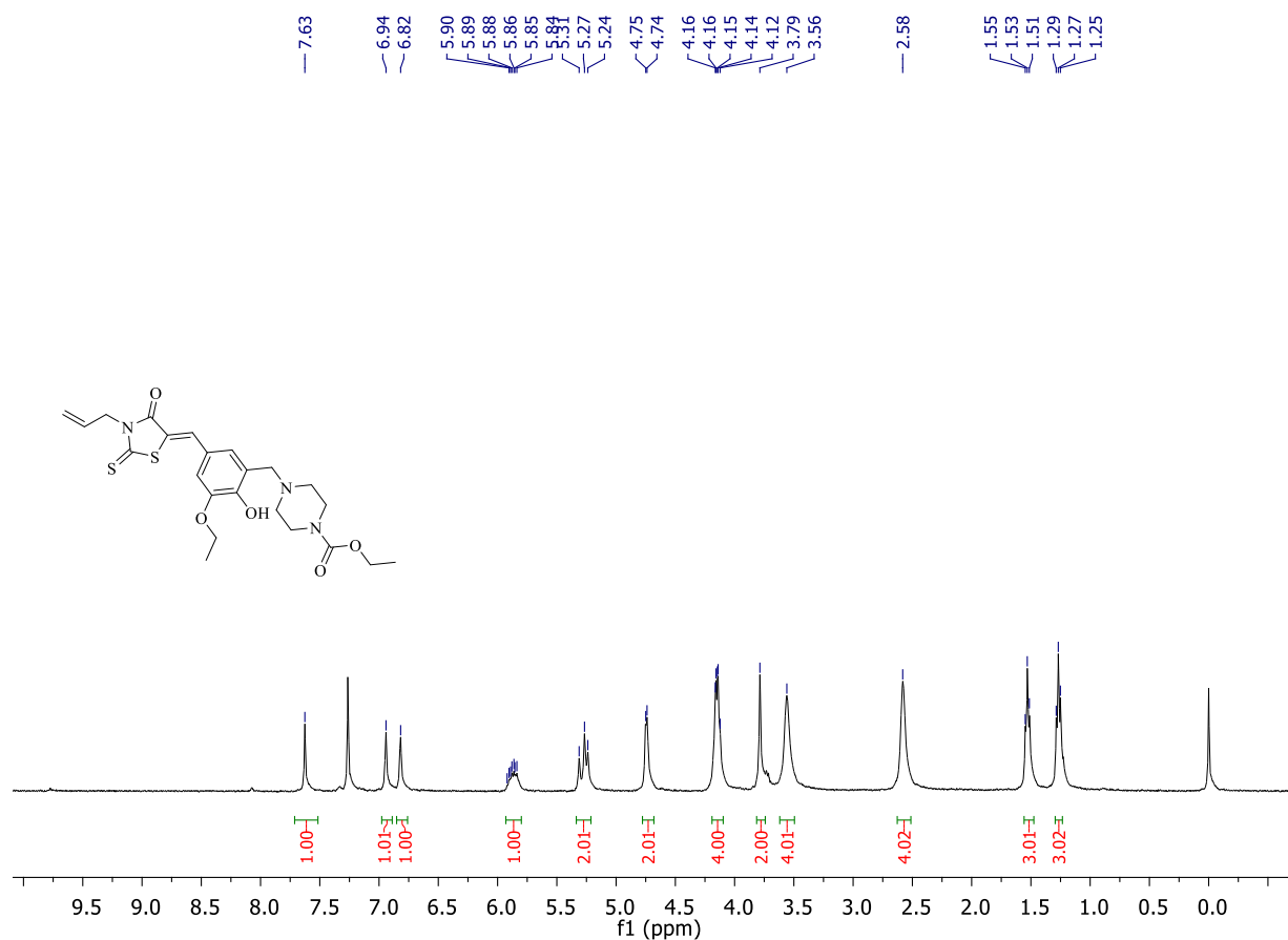
Figure S33. 1 H NMR Spectrum of Compound 9
