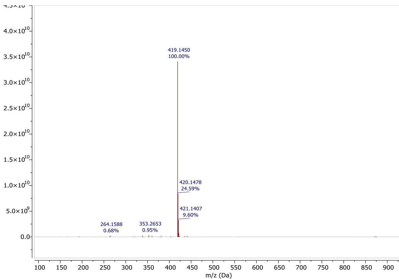
Figure S20. HRMS Spectrum of Compound 5
