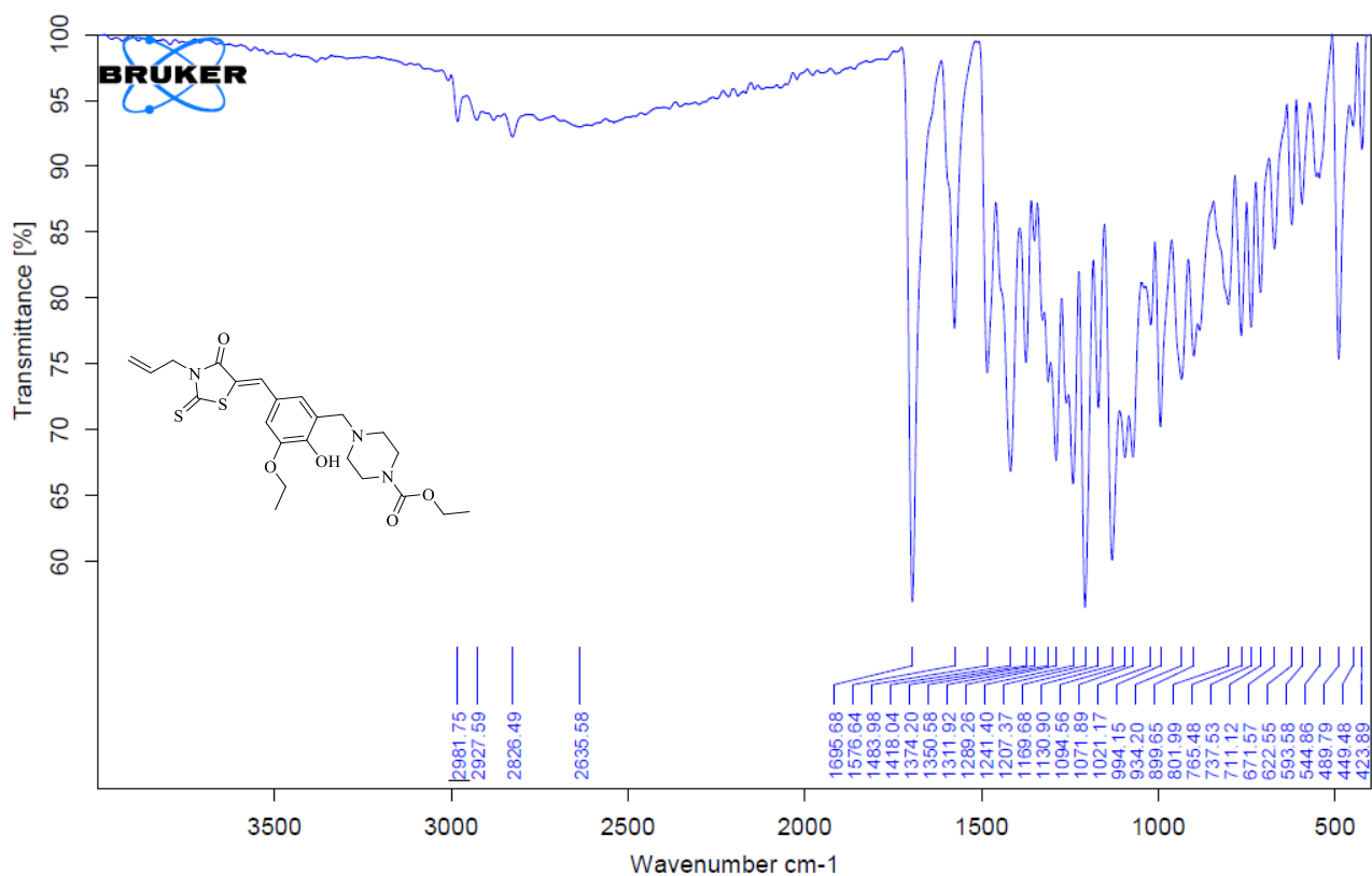
Figure S35. FTIR Spectrum of Compound 9
