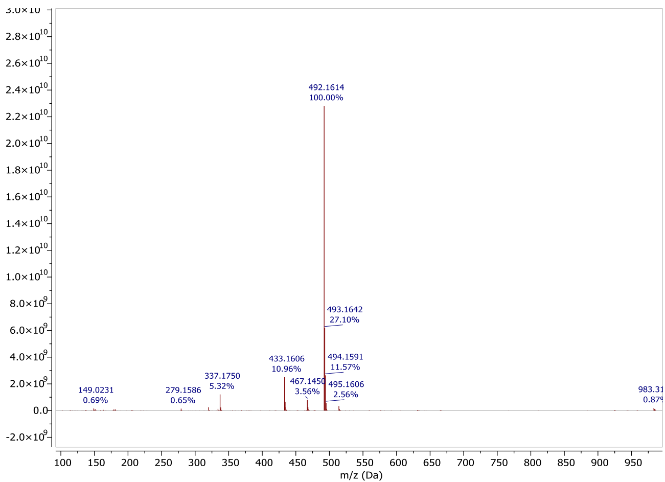
Figure S36. HRMS Spectrum of Compound 9
