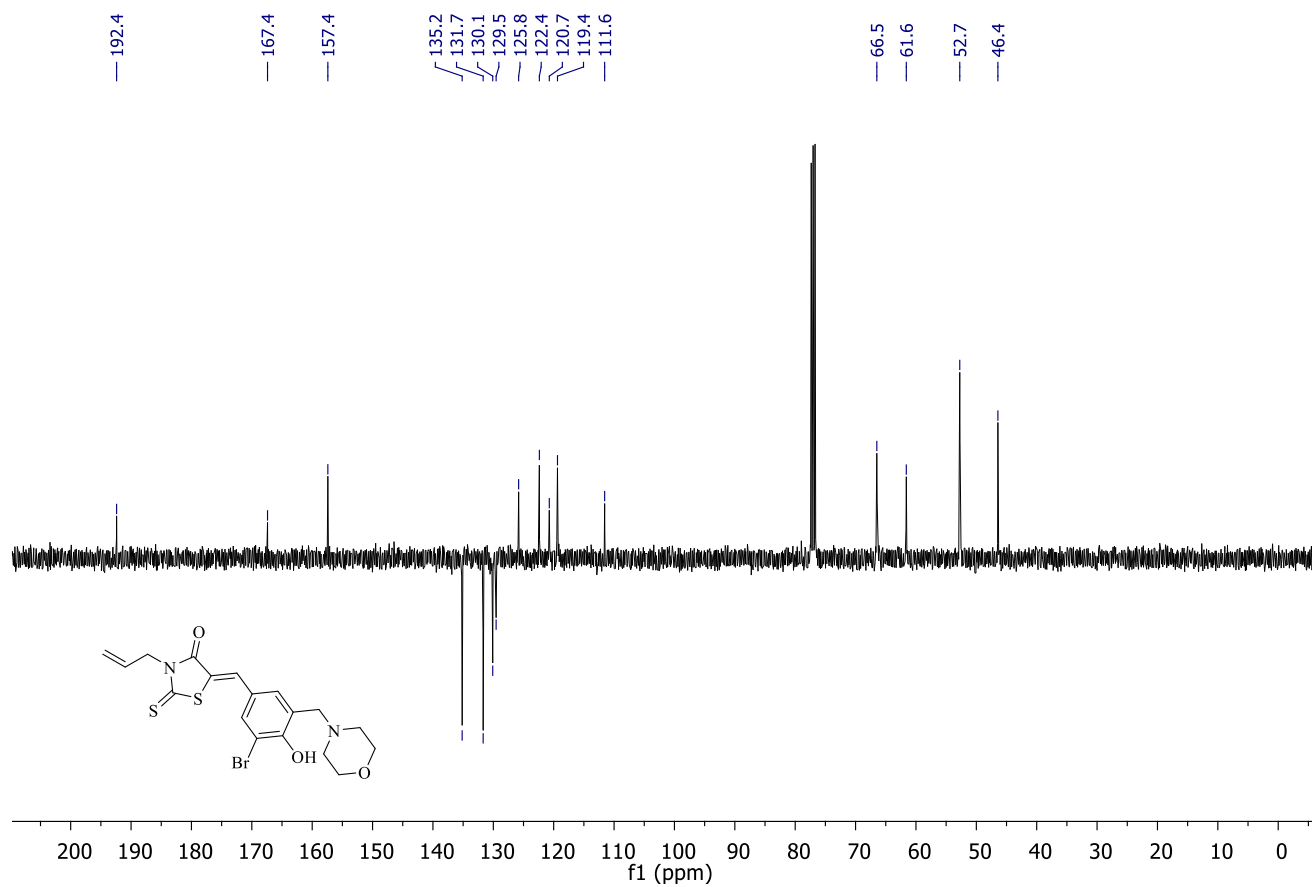
Figure S46. 13 C NMR Spectrum of Compound 12
