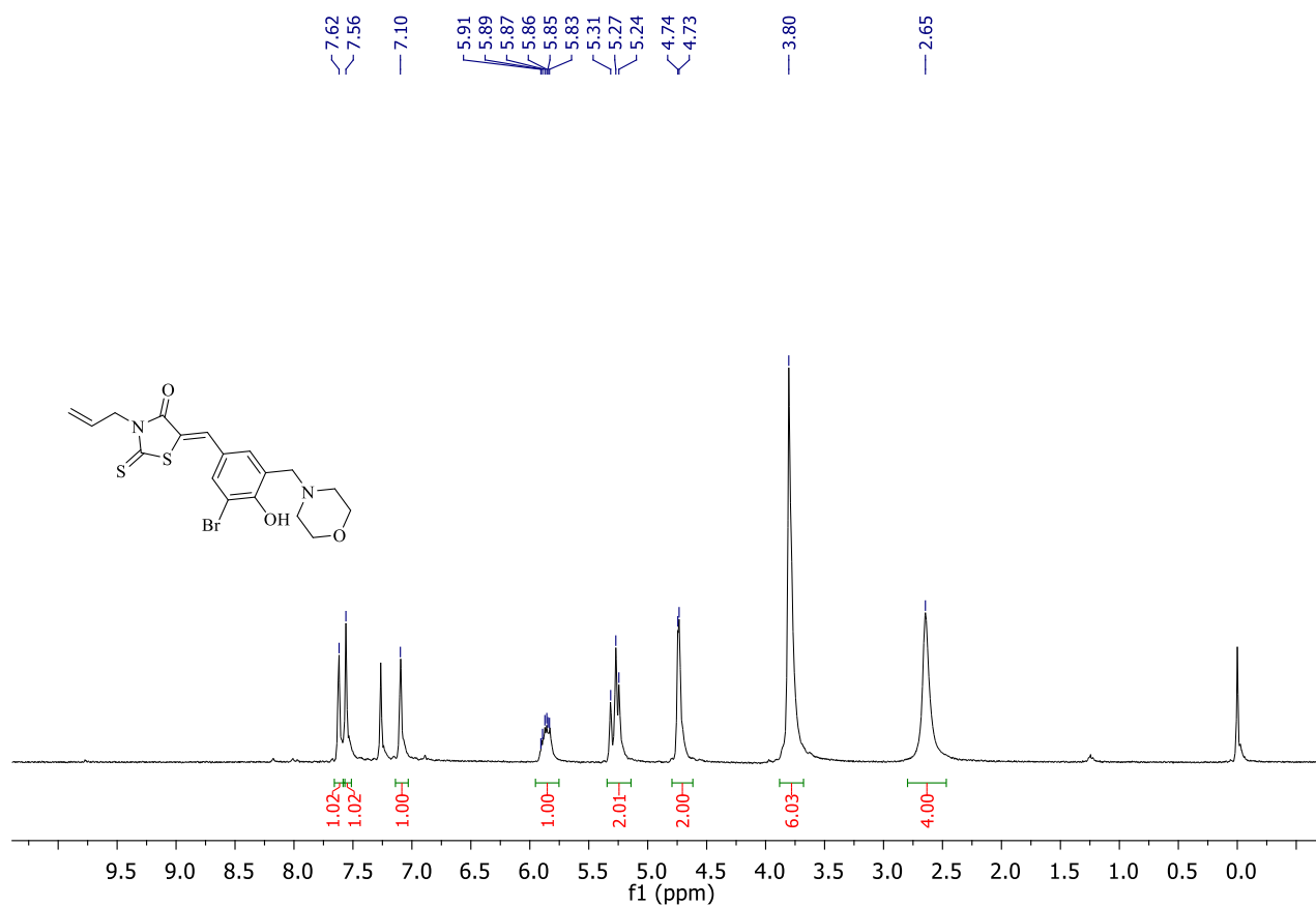
Figure S45. 1 H NMR Spectrum of Compound 12
