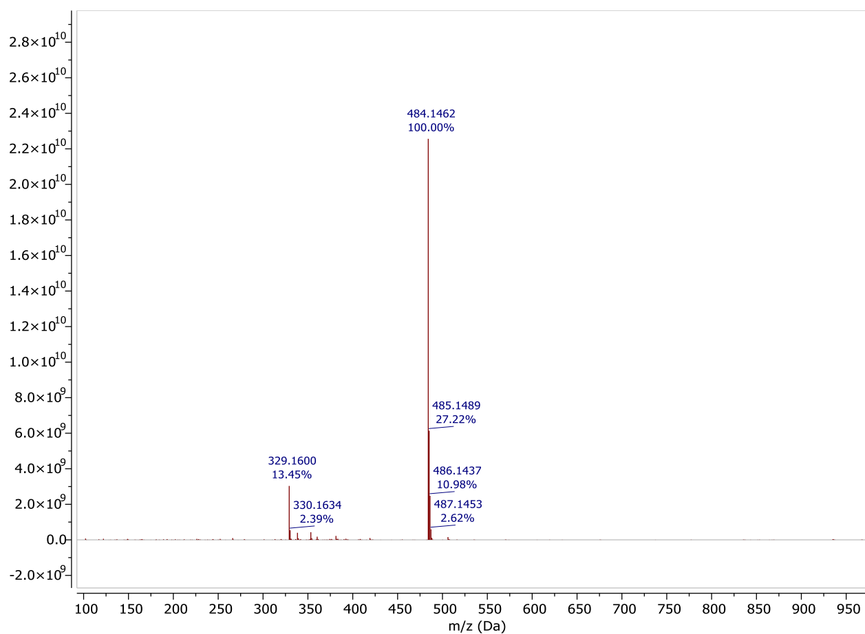
Figure S28. HRMS Spectrum of Compound 7
