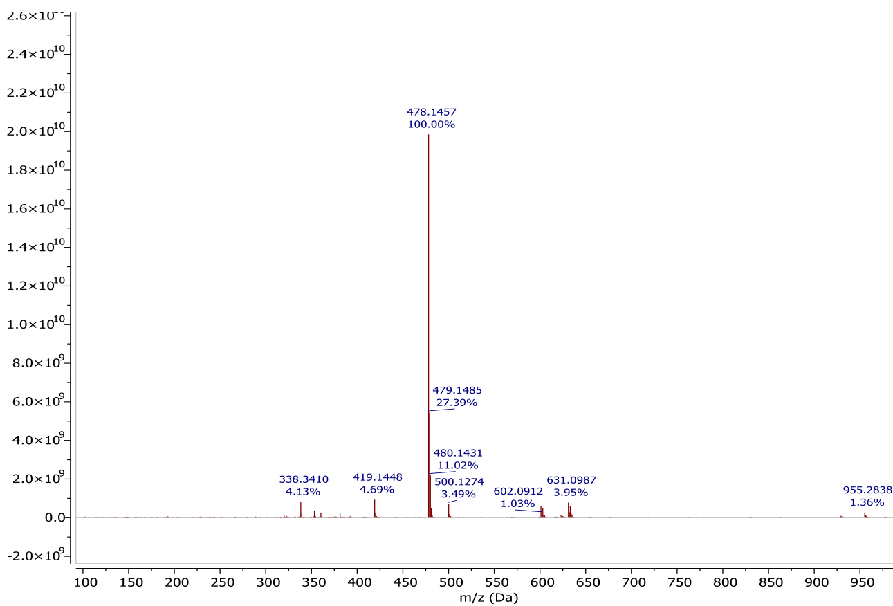
Figure S16. HRMS Spectrum of Compound 4
