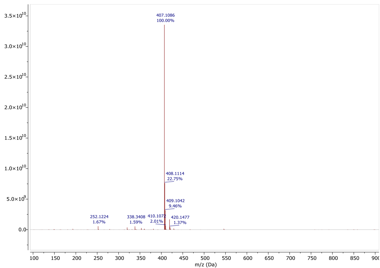
Figure S4. HRMS Spectrum of Compound 1
