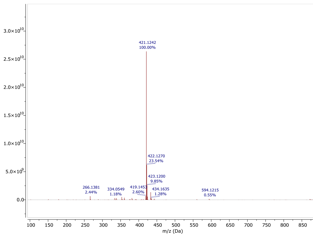
Figure S32. HRMS Spectrum of Compound 8
