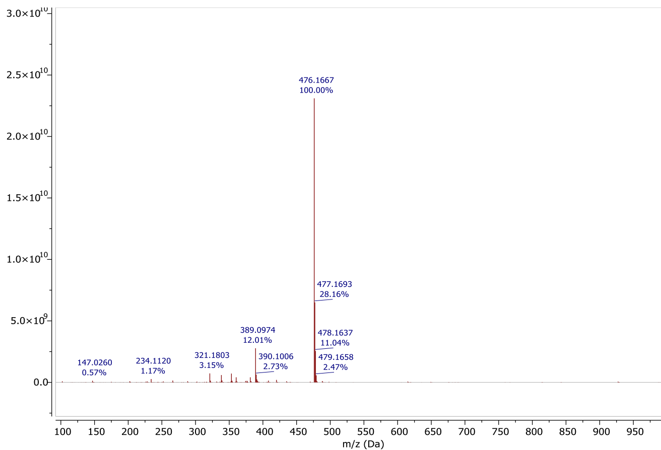
Figure S52. HRMS Spectrum of Compound 13
