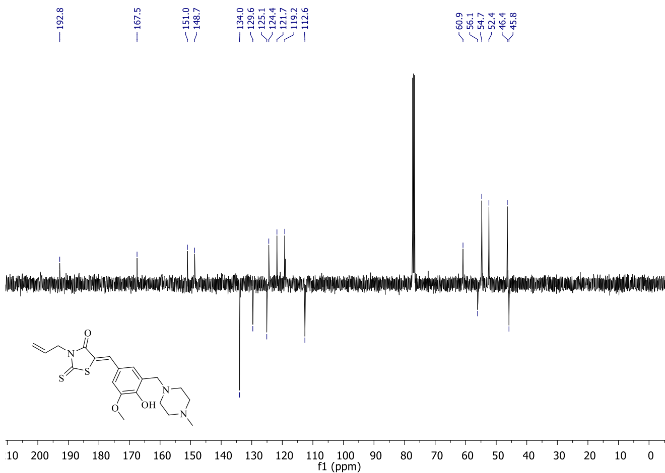
Figure S6. 13 C NMR Spectrum of Compound 2
