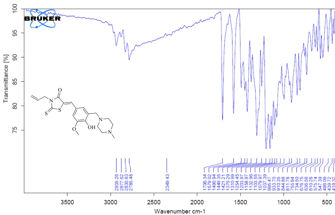
Figure S7. FTIR Spectrum of Compound 2
