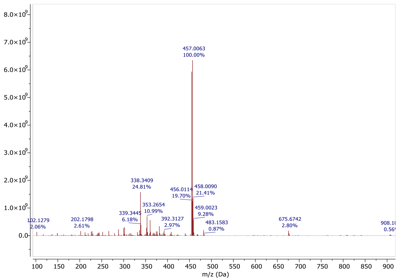
Figure S48. HRMS Spectrum of Compound 12
