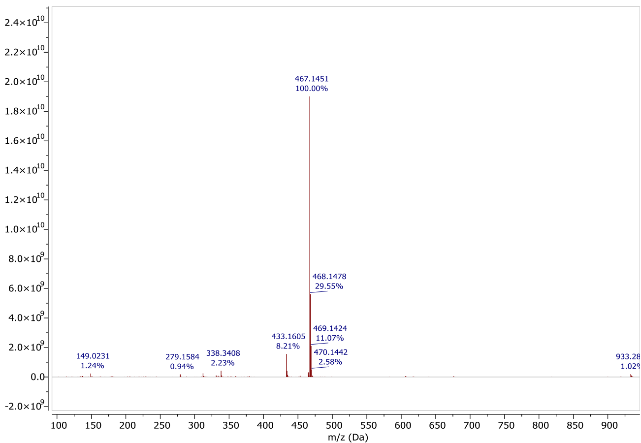
Figure S44. HRMS Spectrum of Compound 11
