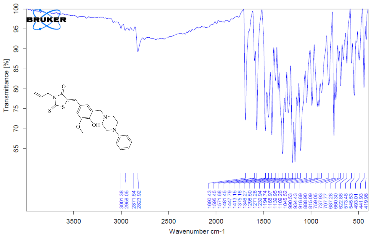
Figure S11. FTIR Spectrum of Compound 3
