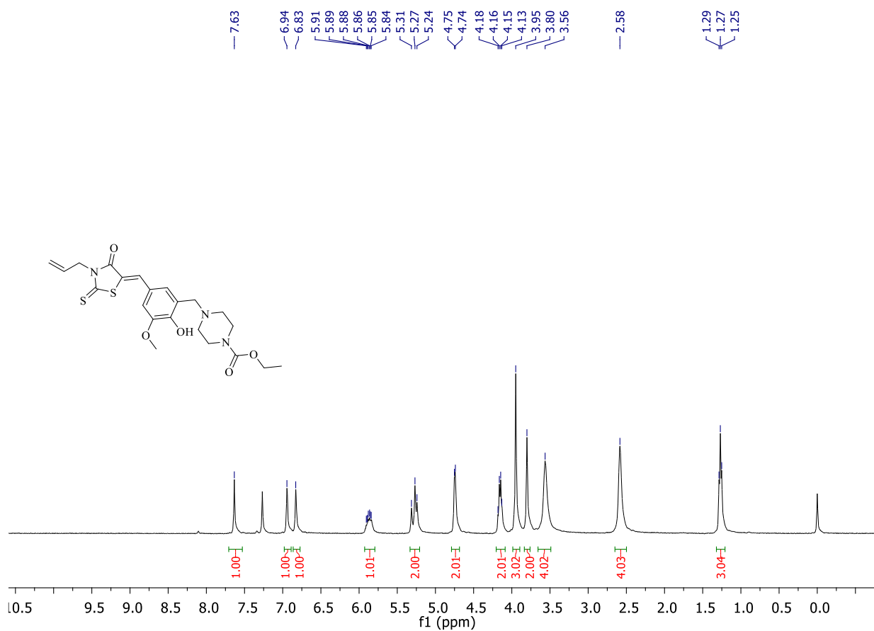
Figure S13. 1 H NMR Spectrum of Compound 4
