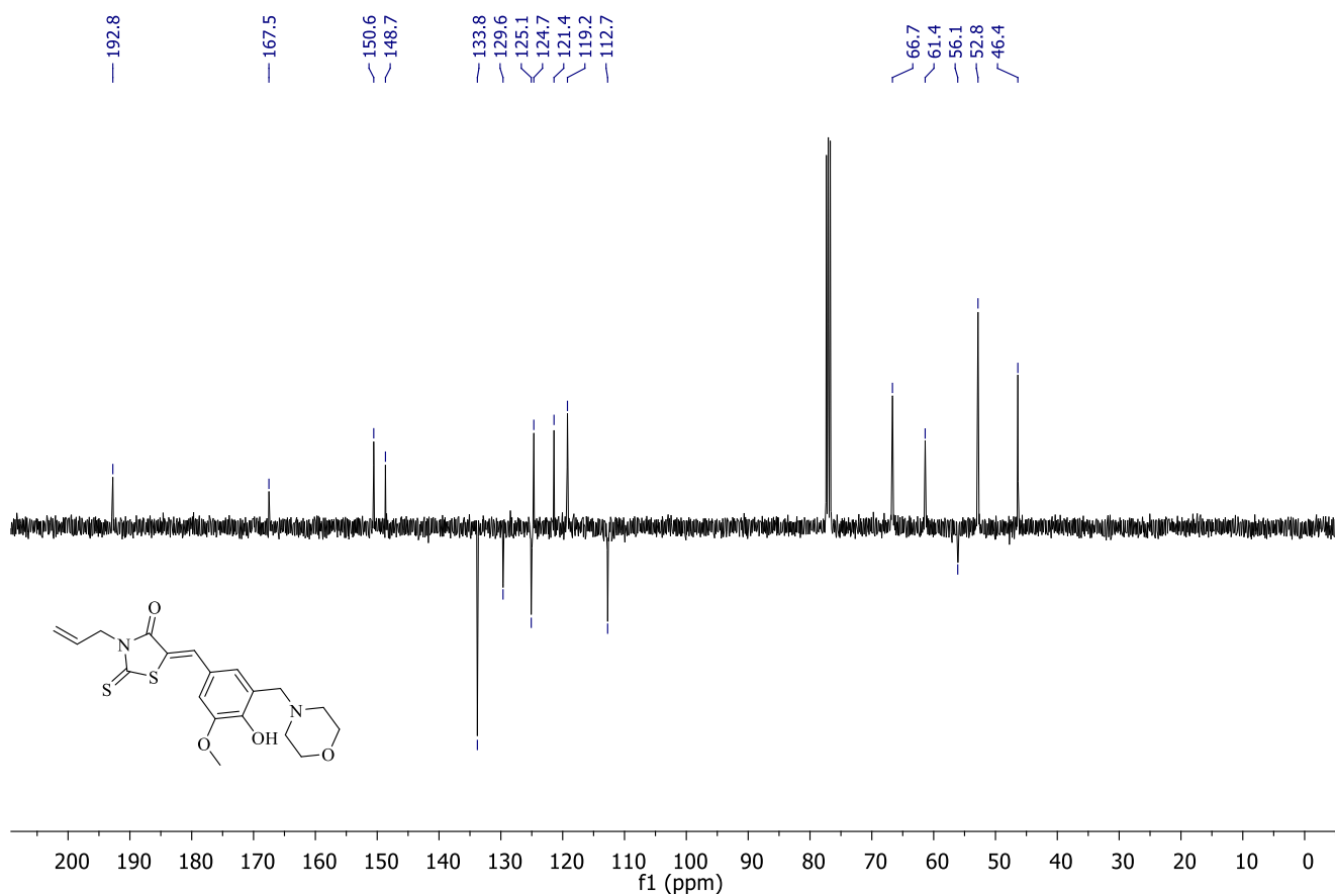
Figure S2. 13 C NMR Spectrum of Compound 1
