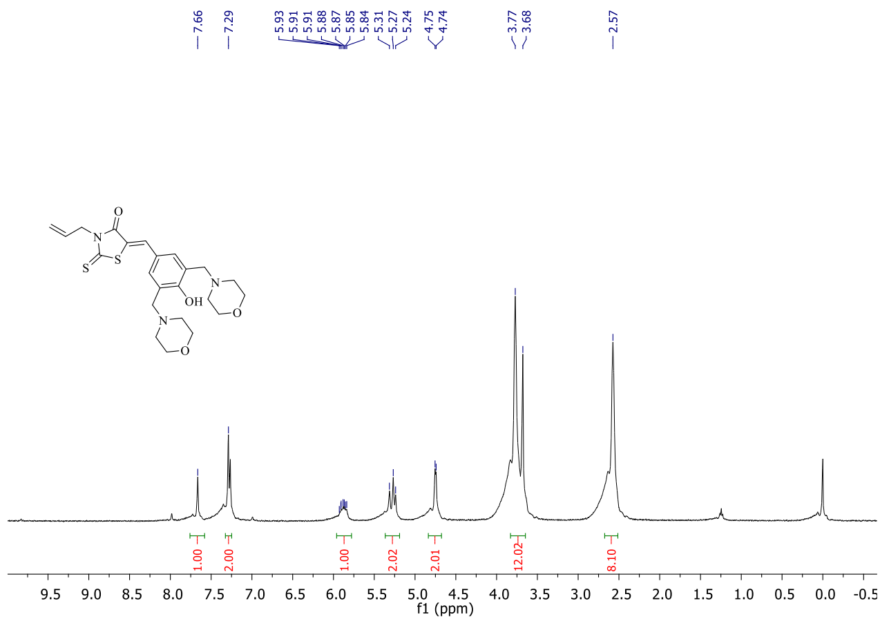
Figure S49. 1 H NMR Spectrum of Compound 13
