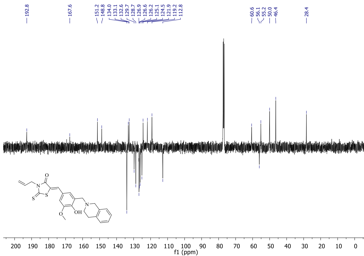
Figure S22. 13 C NMR Spectrum of Compound 6
