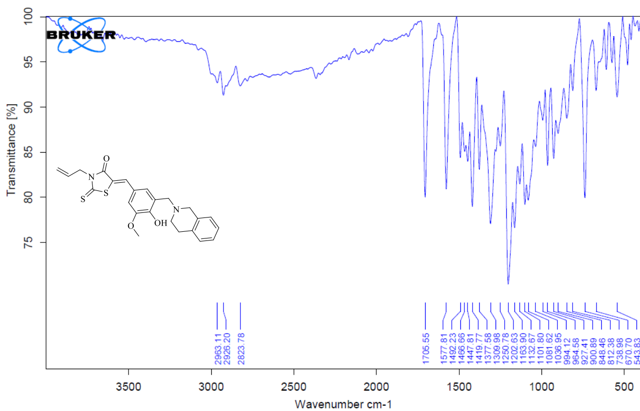
Figure S23. FTIR Spectrum of Compound 6
