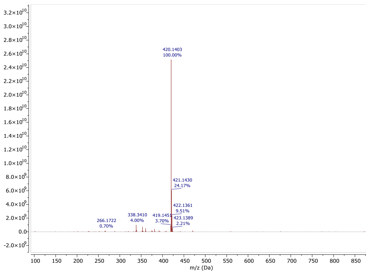
Figure S8. HRMS Spectrum of Compound 2
