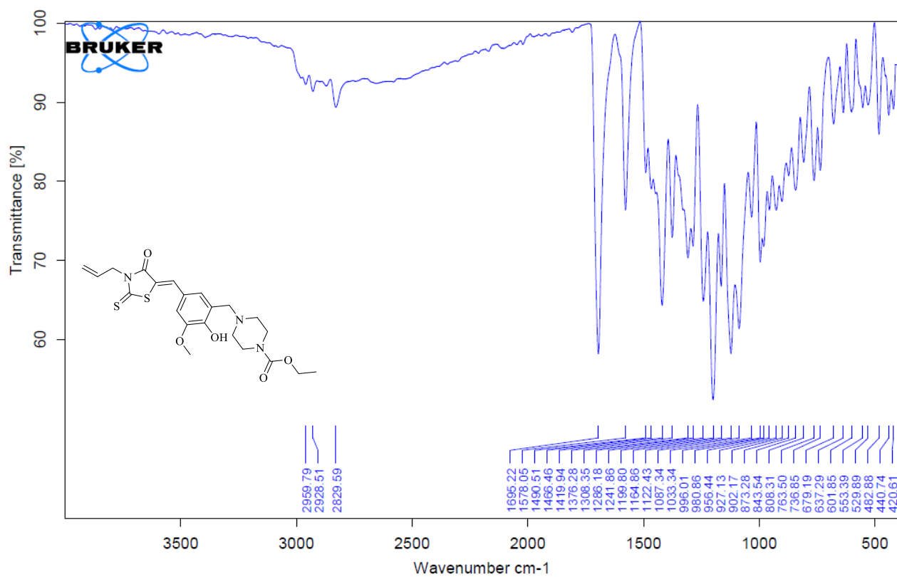
Figure S15. FTIR Spectrum of Compound 4
