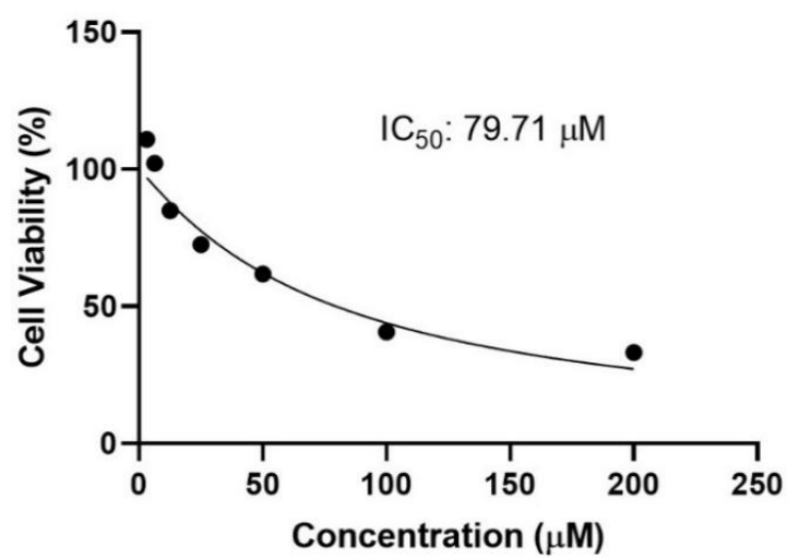
Figure S80. IC 50 Graph of Compound 6 for HUVEC
