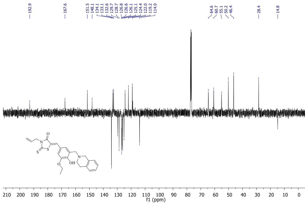
Figure S42. 13 C NMR Spectrum of Compound 11
