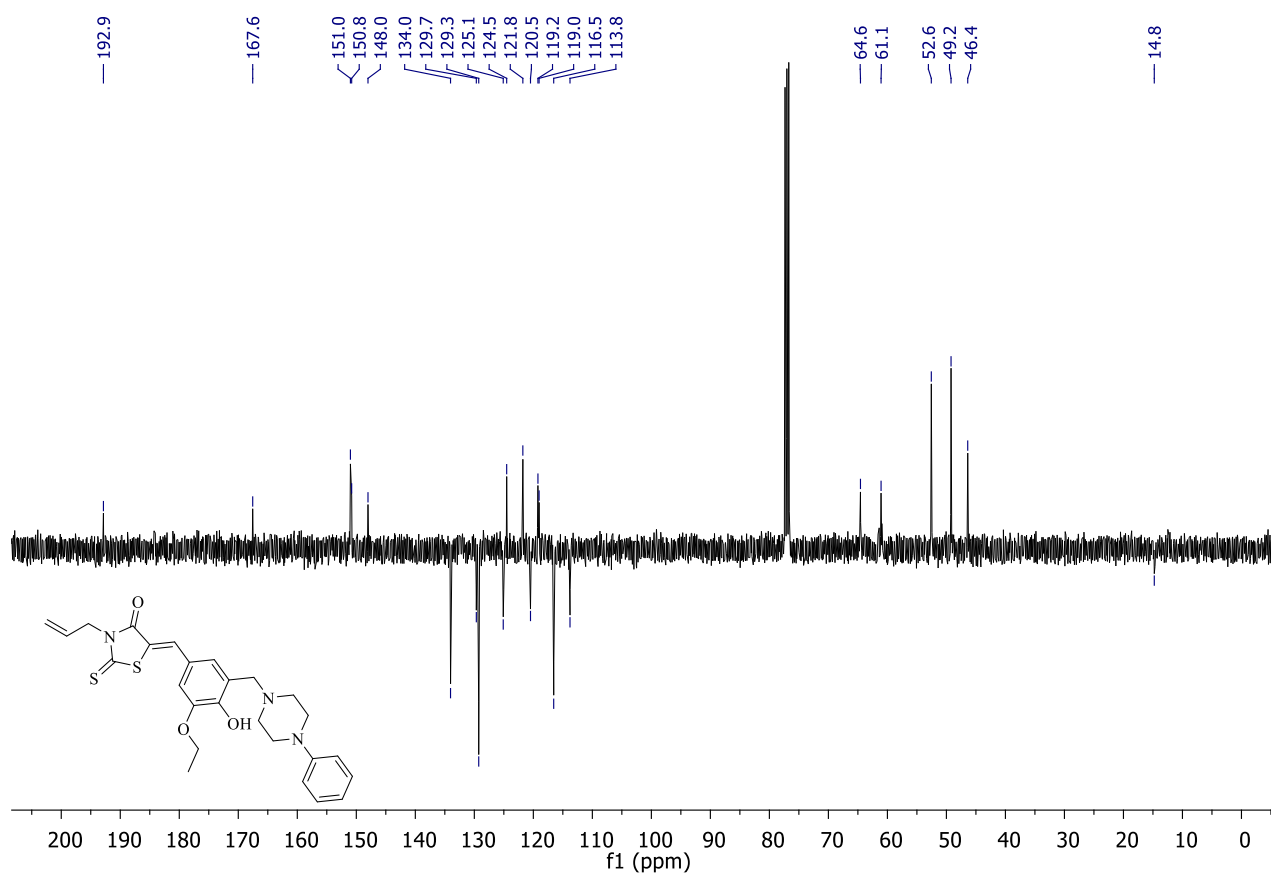
Figure S38. 13 C NMR Spectrum of Compound 10
