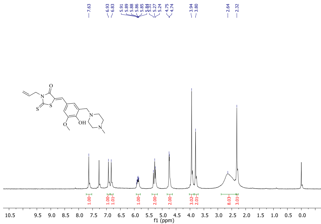
Figure S5. 1 H NMR Spectrum of Compound 2
