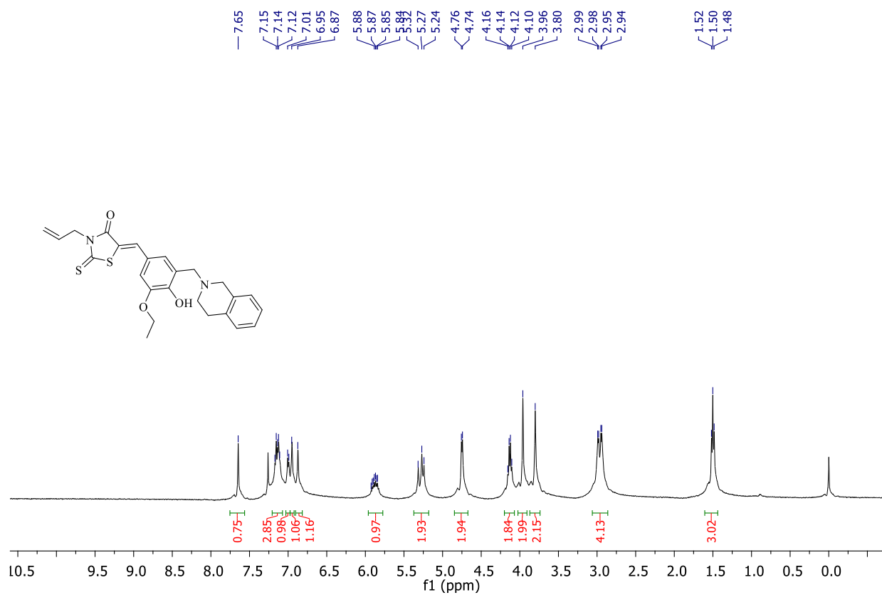
Figure S41. 1 H NMR Spectrum of Compound 11
