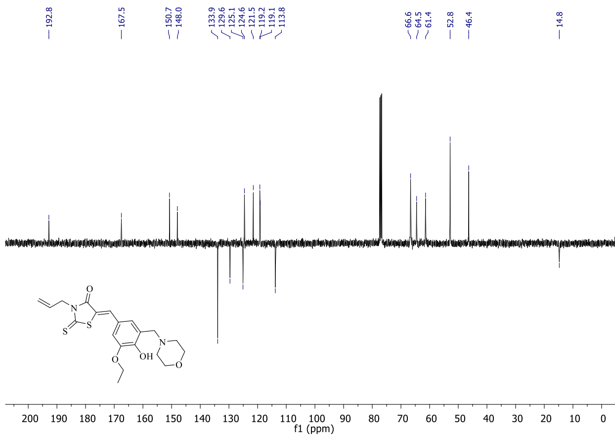
Figure S30. 13 C NMR Spectrum of Compound 8
