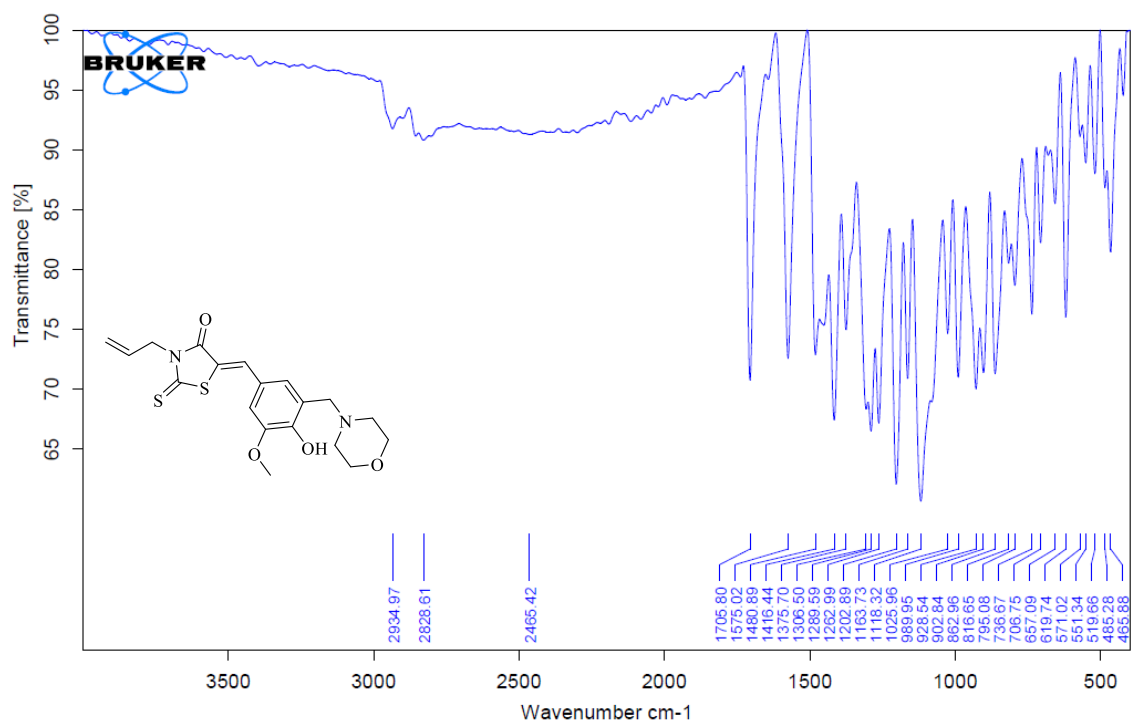
Figure S3. FTIR Spectrum of Compound 1
