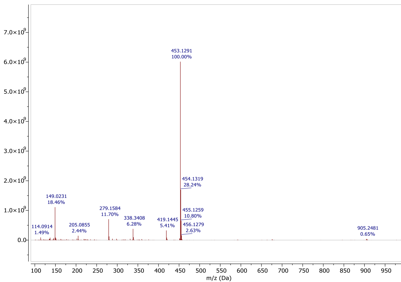
Figure S24. HRMS Spectrum of Compound 6
