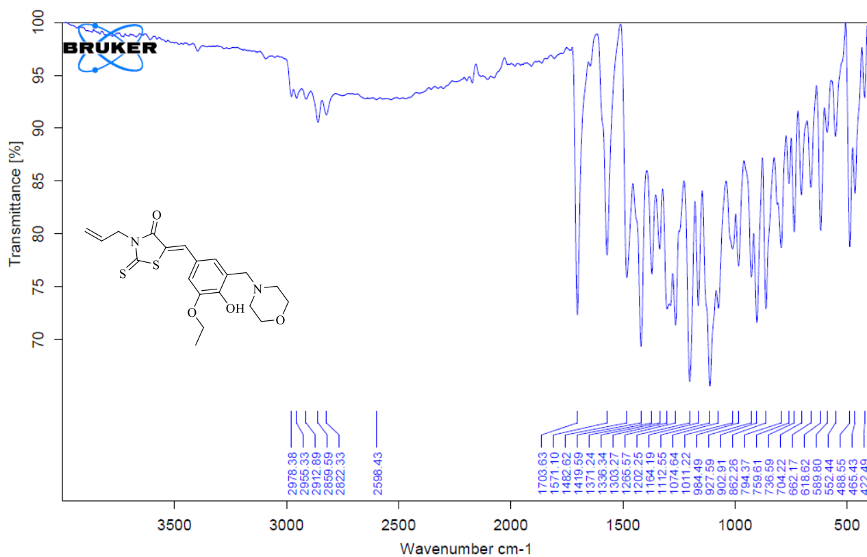
Figure S31. FTIR Spectrum of Compound 8
