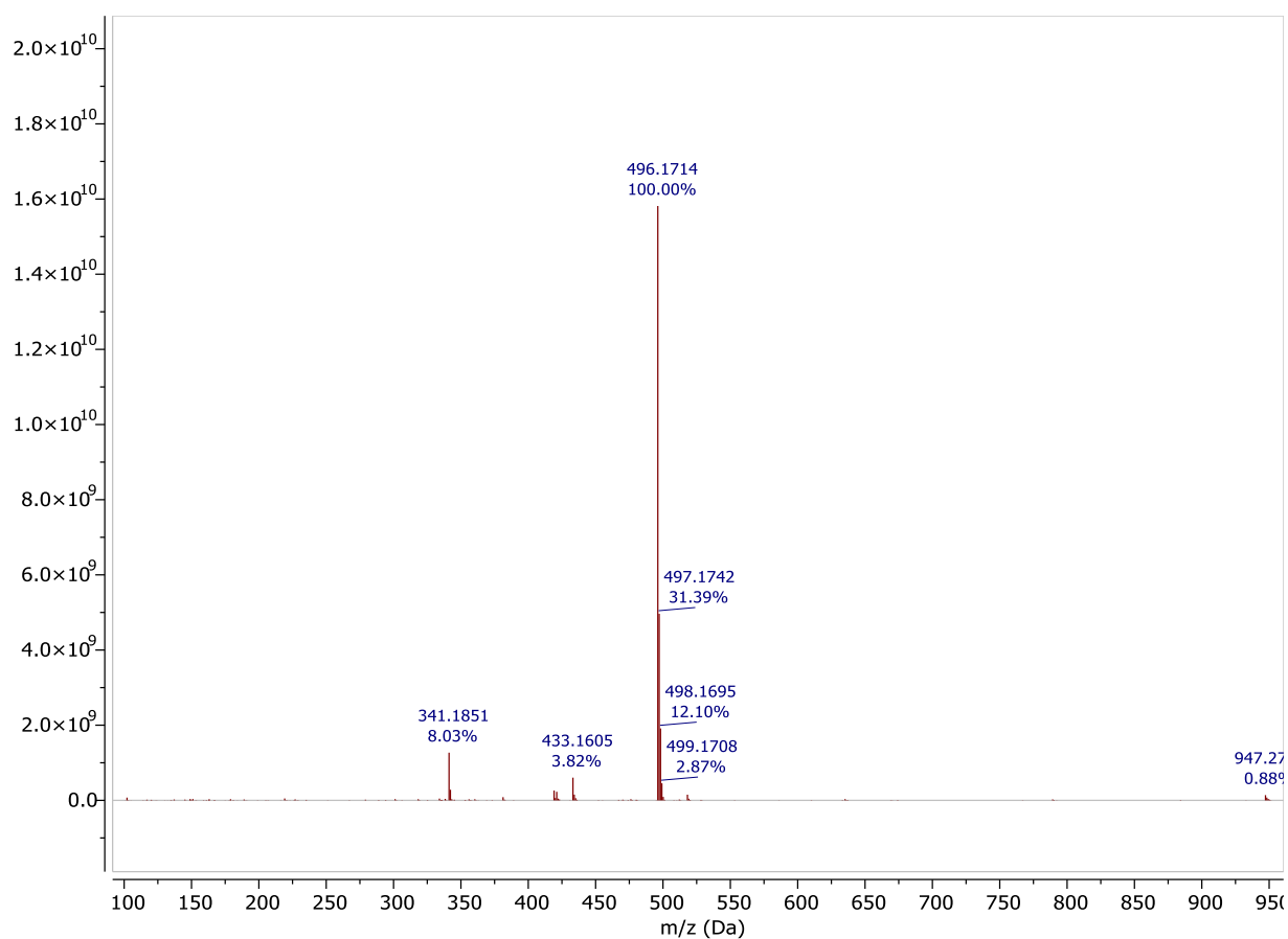
Figure S40. HRMS Spectrum of Compound 10
