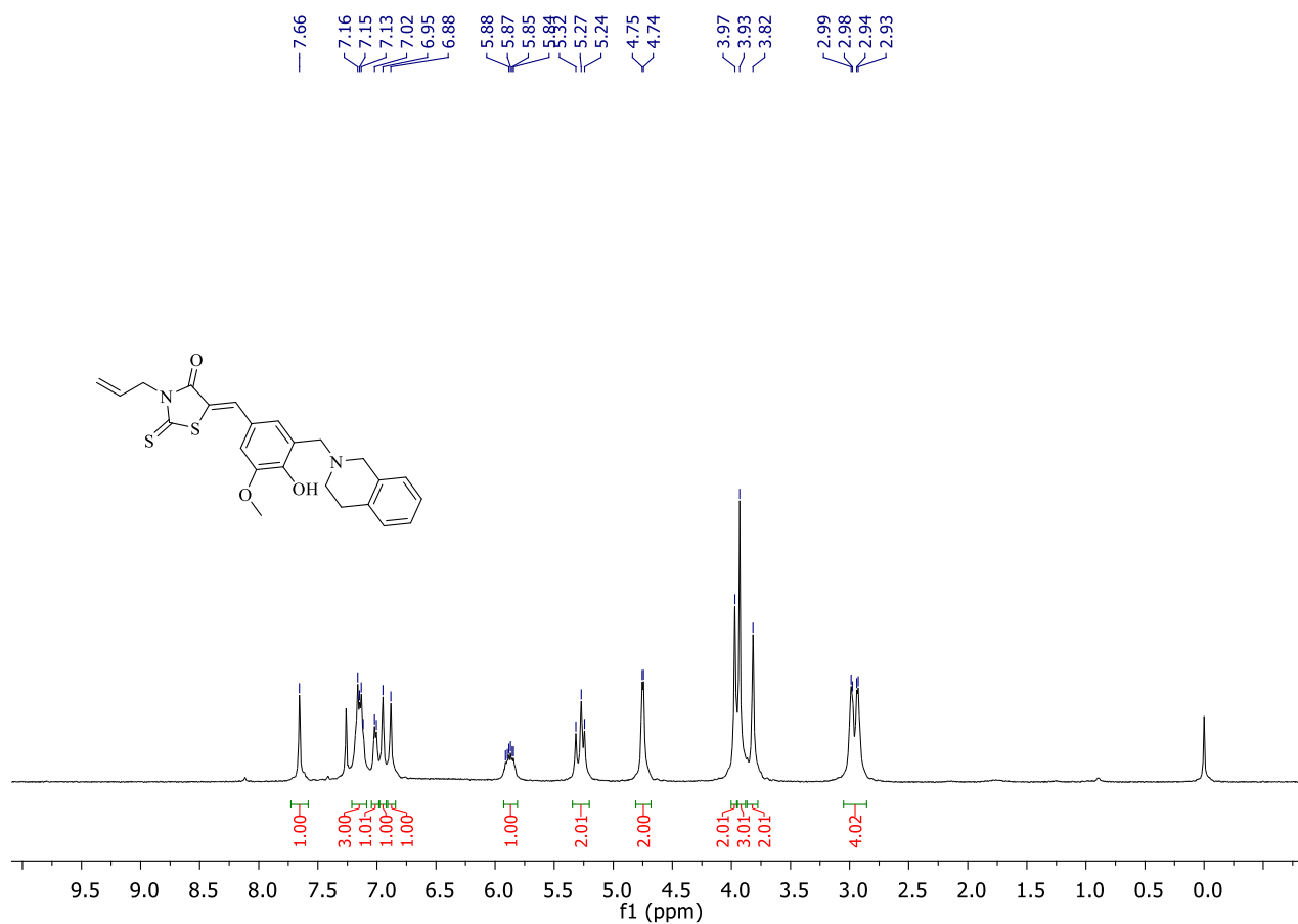
Figure S21. 1 H NMR Spectrum of Compound 6
