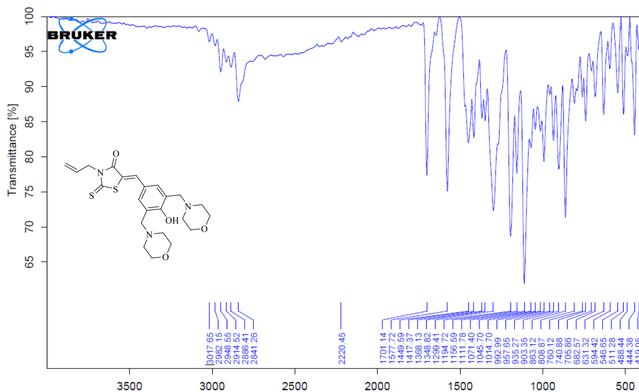
Figure S51. FTIR Spectrum of Compound 13
