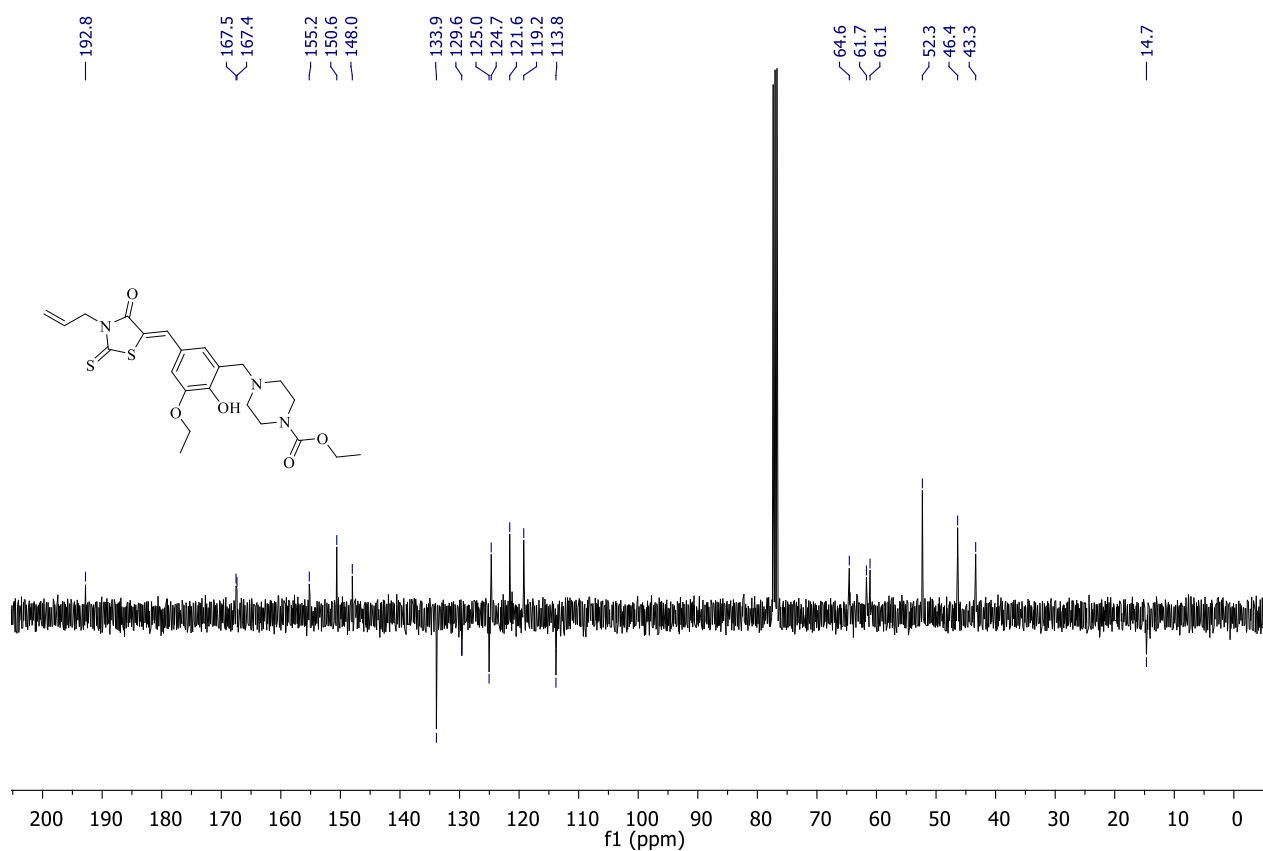
Figure S34. 13 C NMR Spectrum of Compound 9
