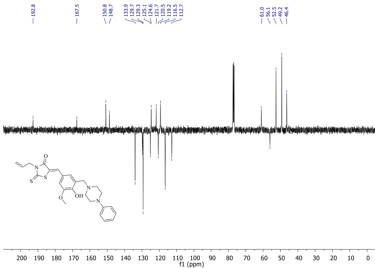
Figure S10. 13 C NMR Spectrum of Compound 3
