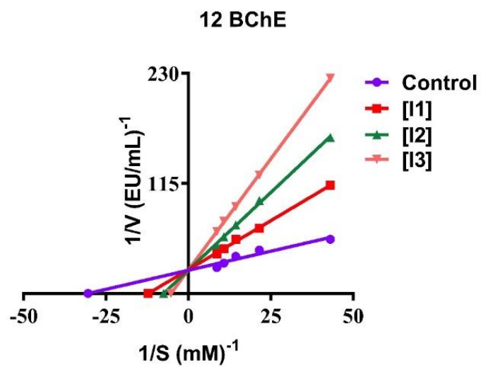
Figure S77. Lineweaver-Burk plots of compound 12 for BChE
