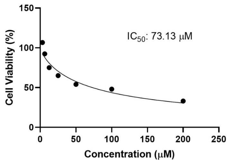
Figure S79. IC 50 Graph of Compound 4 for HUVEC
