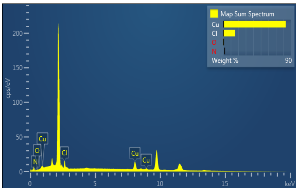
Figure S1: EDX Colour Mapping of Sample OA120D00 (a) Sum Spectra Map of the Selected Surface (b)
