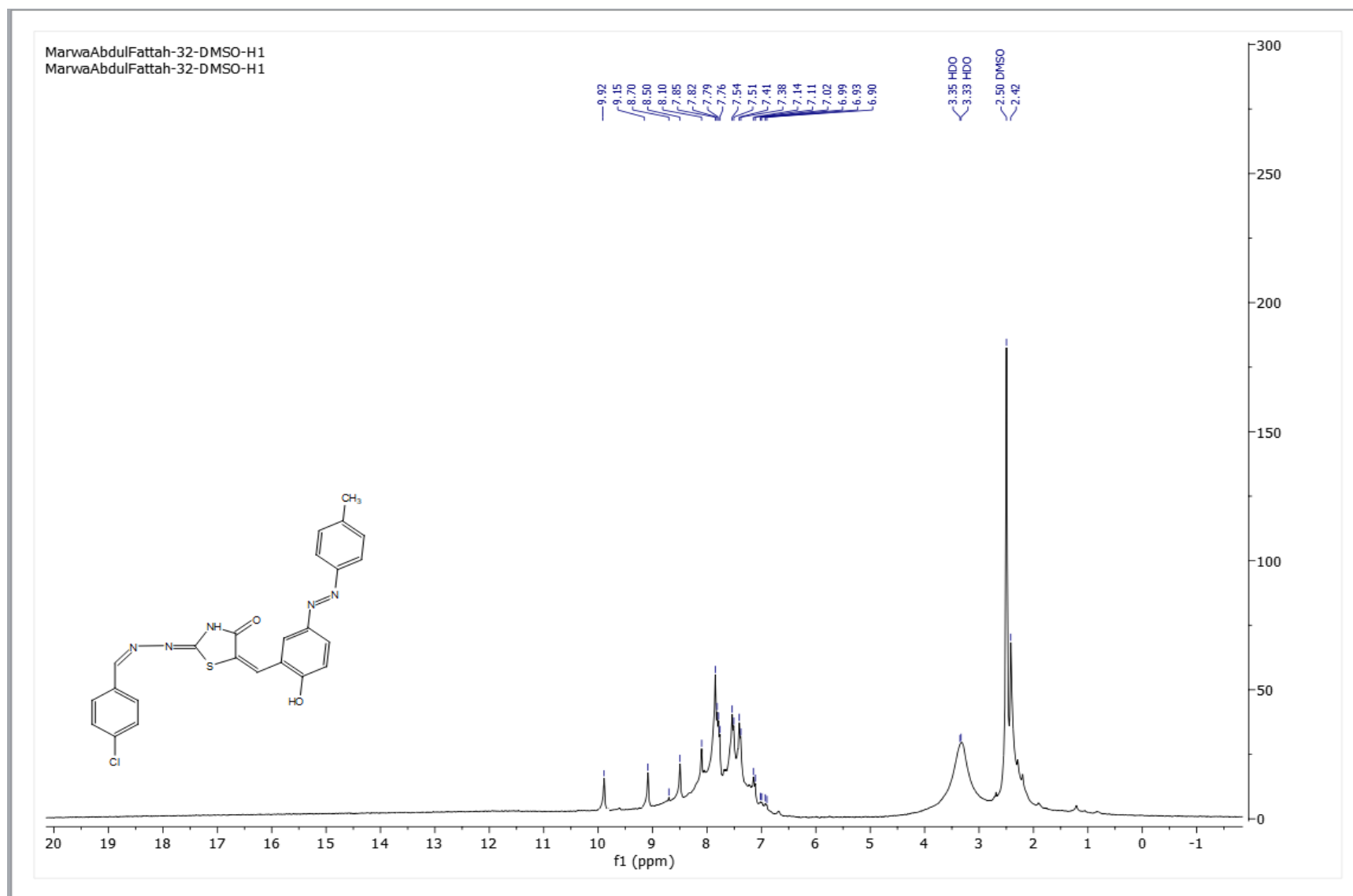
Figure. S4b B: ^1\text{H} -NMR spectrum of compound 4b (dye 2).
