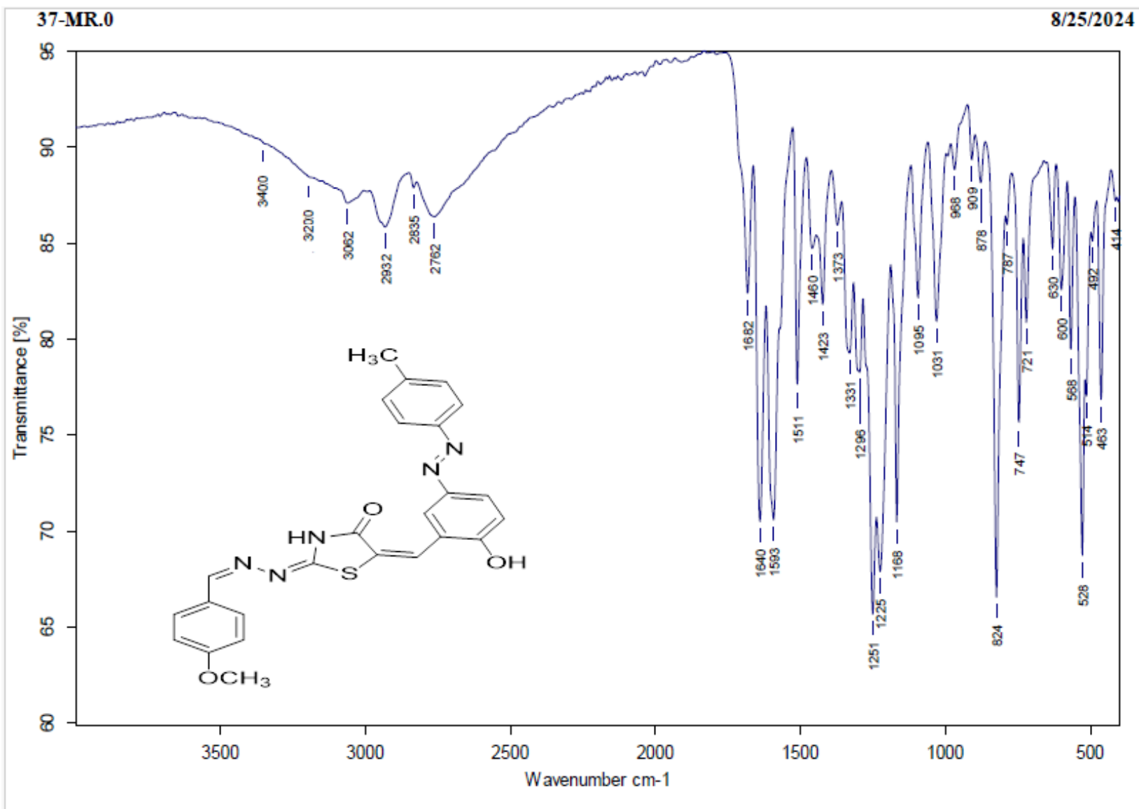
Figure. S6b A: IR spectrum of compound 6ab(dye 6) .
