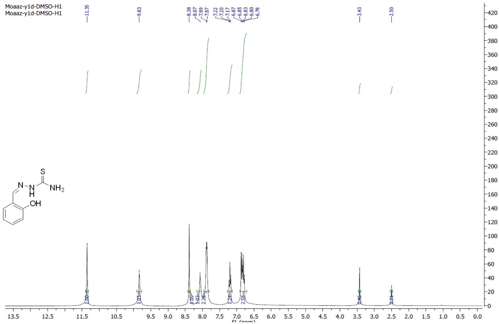
Figure. S1d B: ^1\text{H} -NMR spectrum of compound 1d
