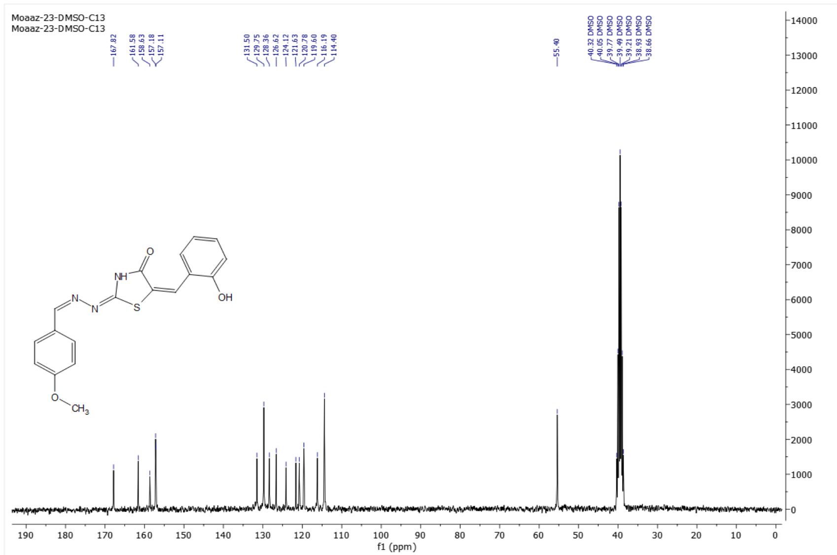
Figure. S3c C: ^{13}\text{C} -NMR spectrum of compound 3c .
