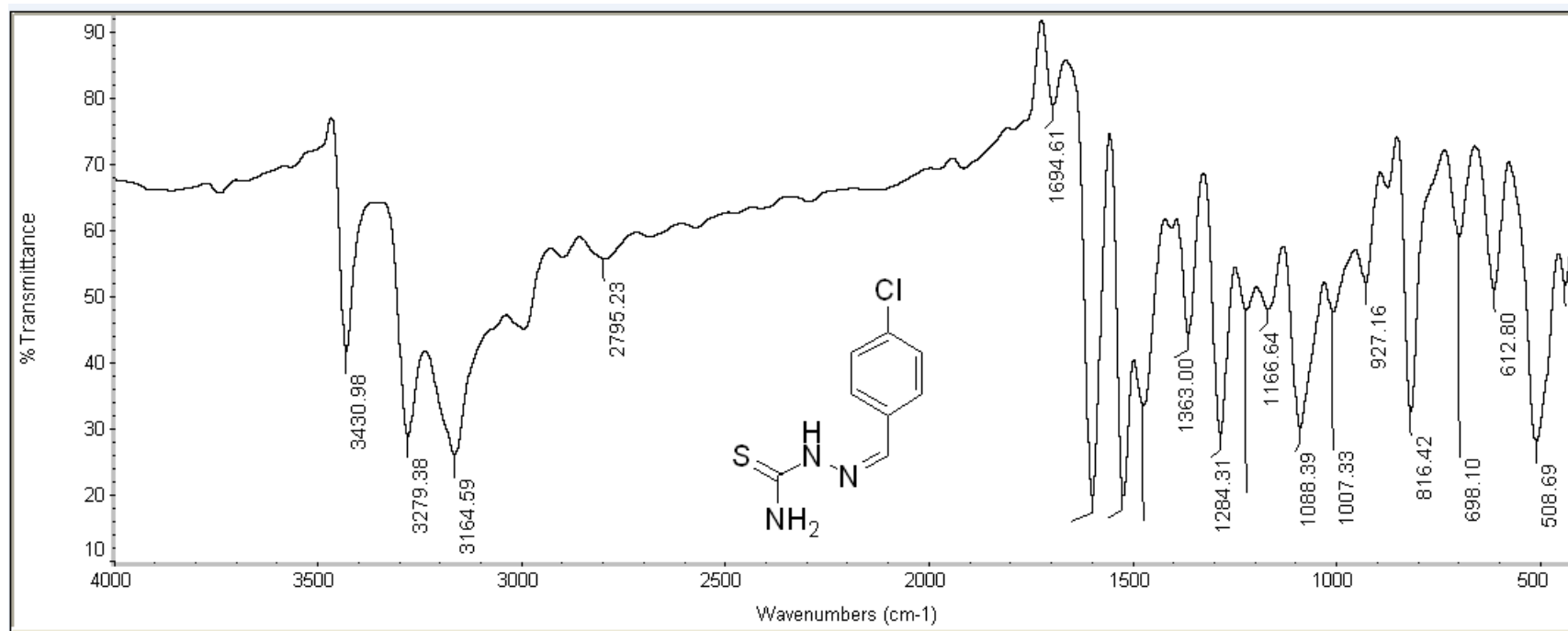
Figure. S1a A: IR spectrum of compound 1a
