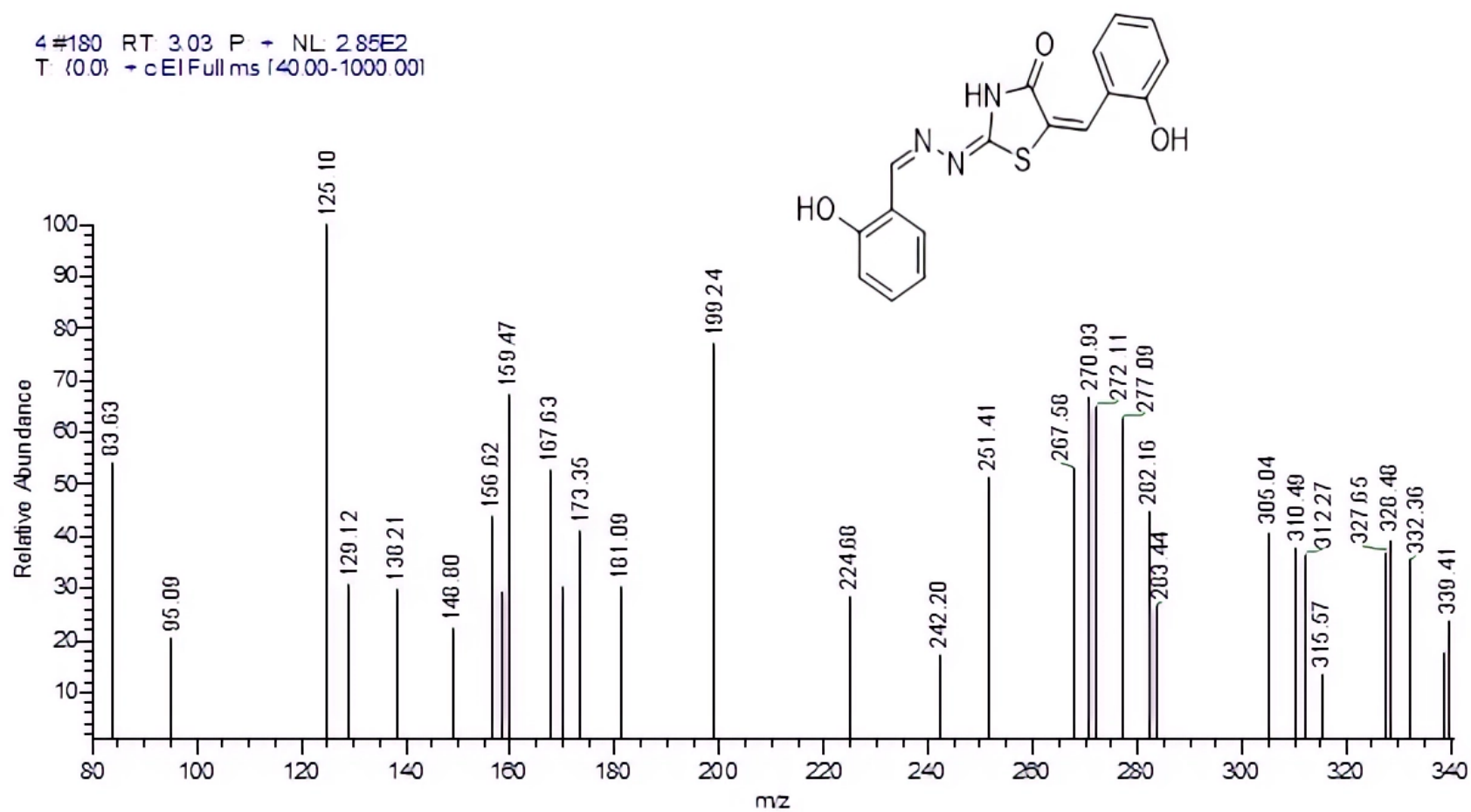
Figure. S3d D: Mass spectrum of compound 3d .
