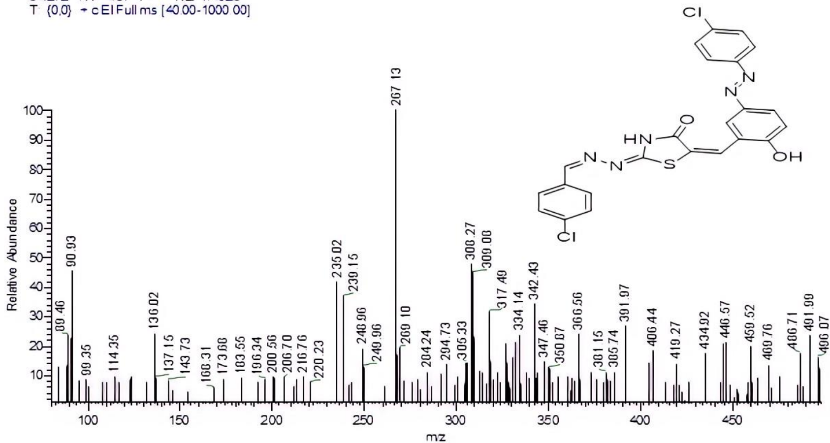
Figure. S4a D: Mass spectrum of compound 4a(dye 1).
