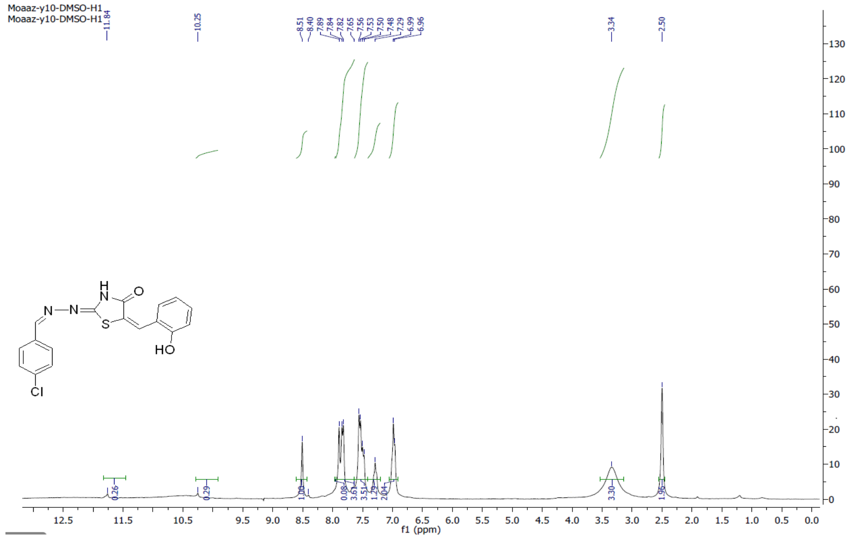
Figure. S3a B: ^1\text{H} -NMR spectrum of compound 3a
