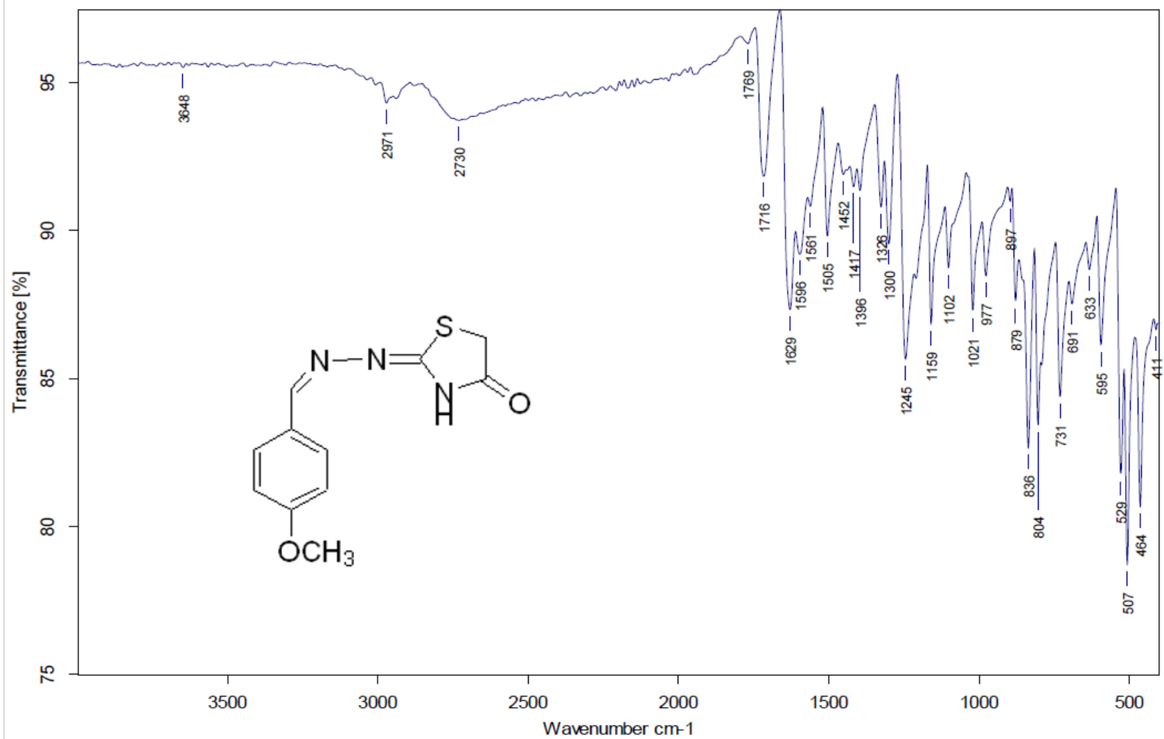
Figure. S 2c A: IR spectrum of compound 2c
