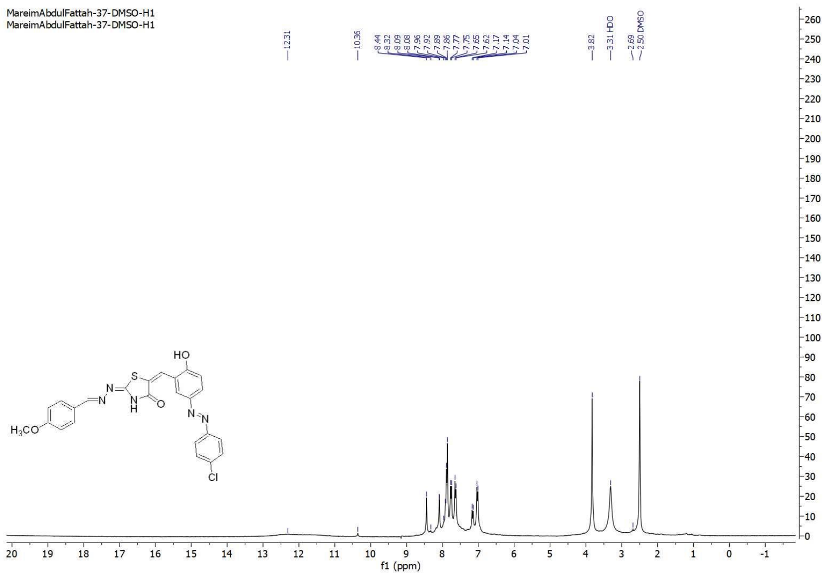
Figure. S6a B: 1 H-NMR spectrum of compound 6a (dye 5 ).
