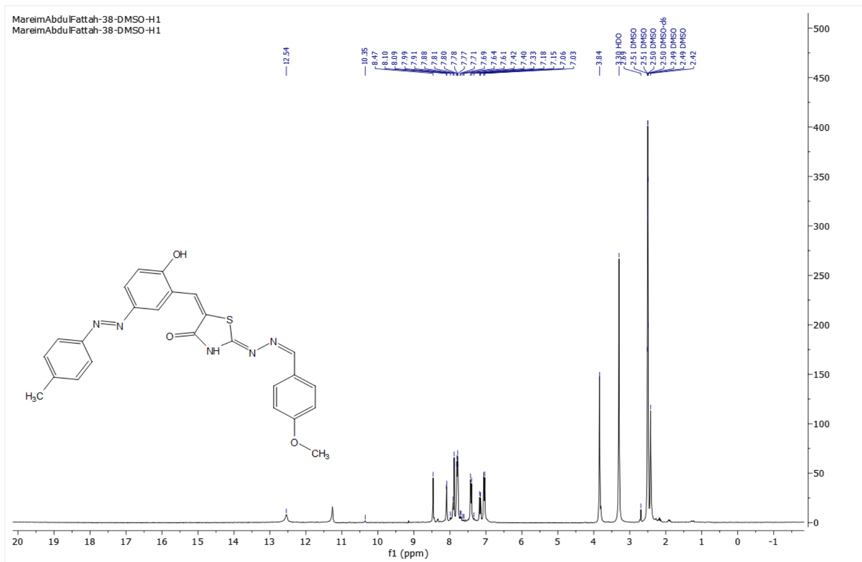
Figure. S6b B: 1 H-NMR spectrum of compound 6b (dye 6 ).
