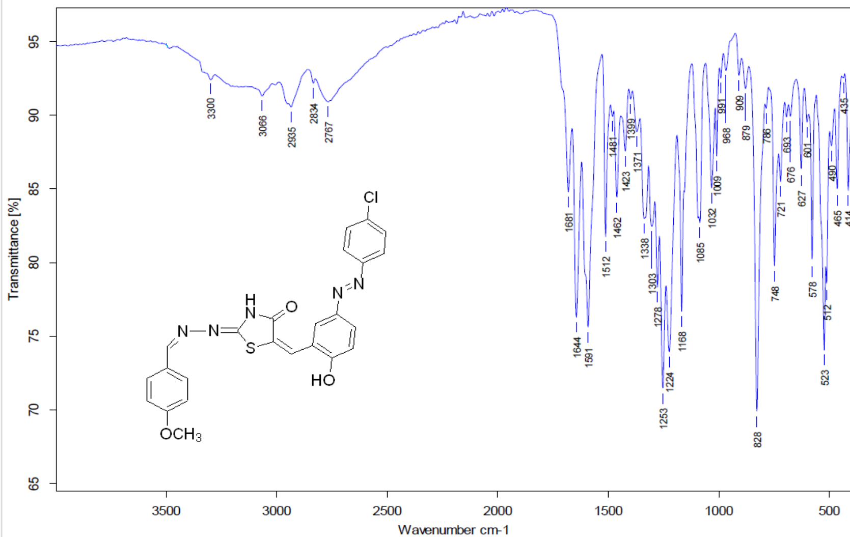
Figure. S6a A: IR spectrum of compound 6a(dye 5).
