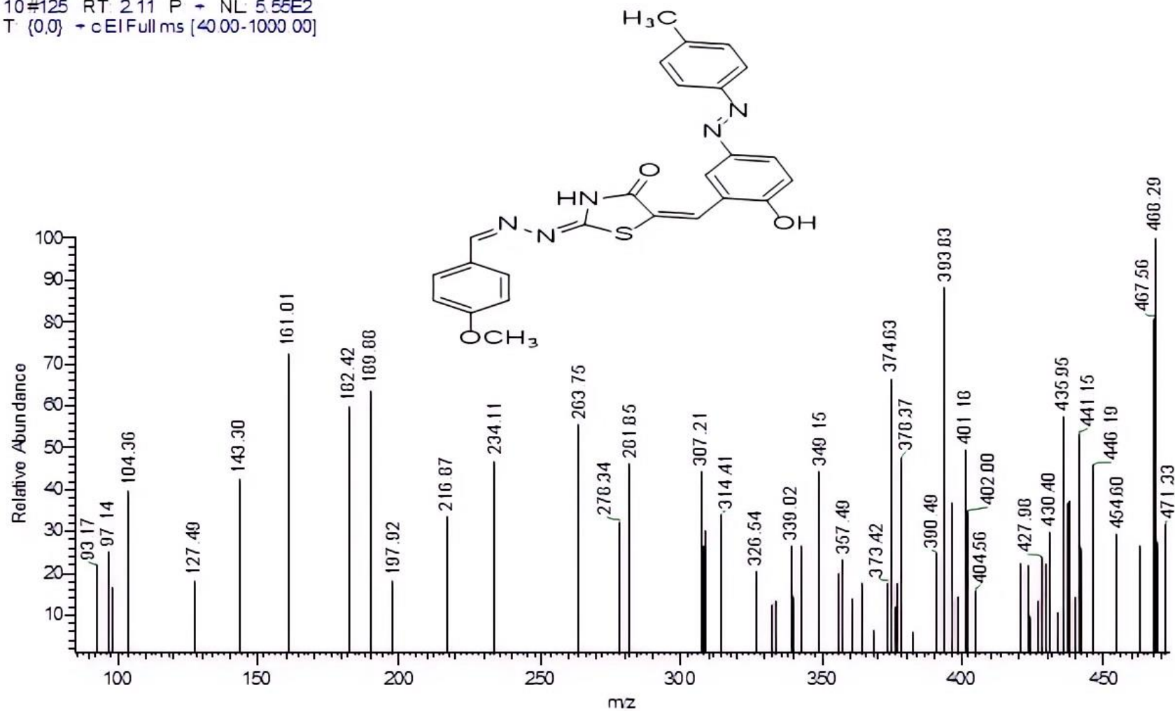
Figure. S6b D: Mass spectrum of compound 6b(dye 6) .
