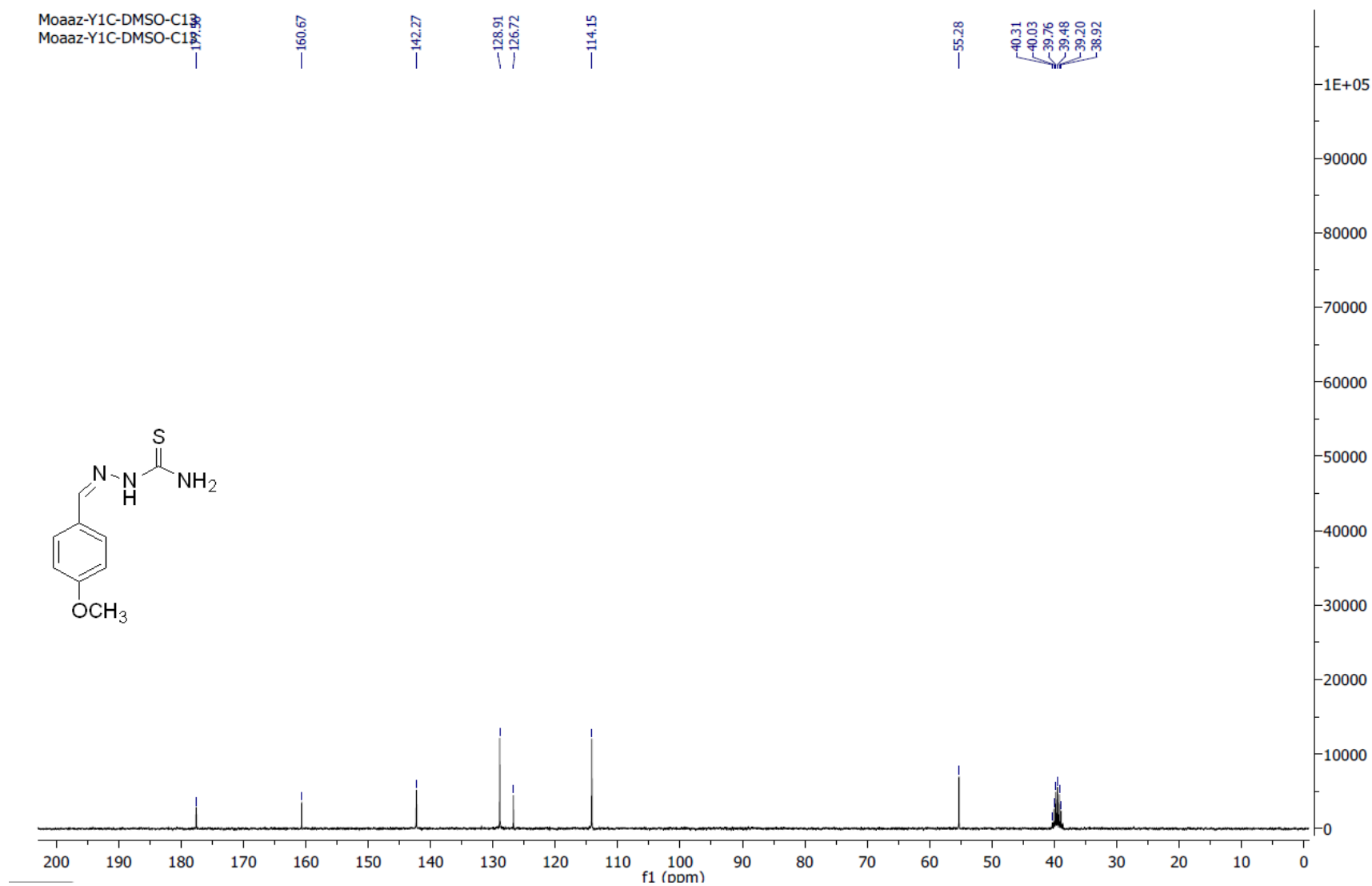
Figure. S1c C: 13 C-NMR spectrum of compound 1c
