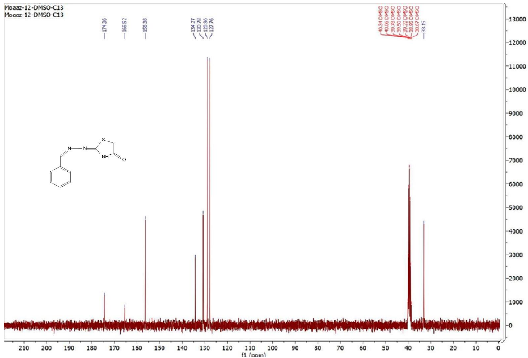
Figure. S2b C: ^{13}\text{C} -NMR spectrum of compound 2b
