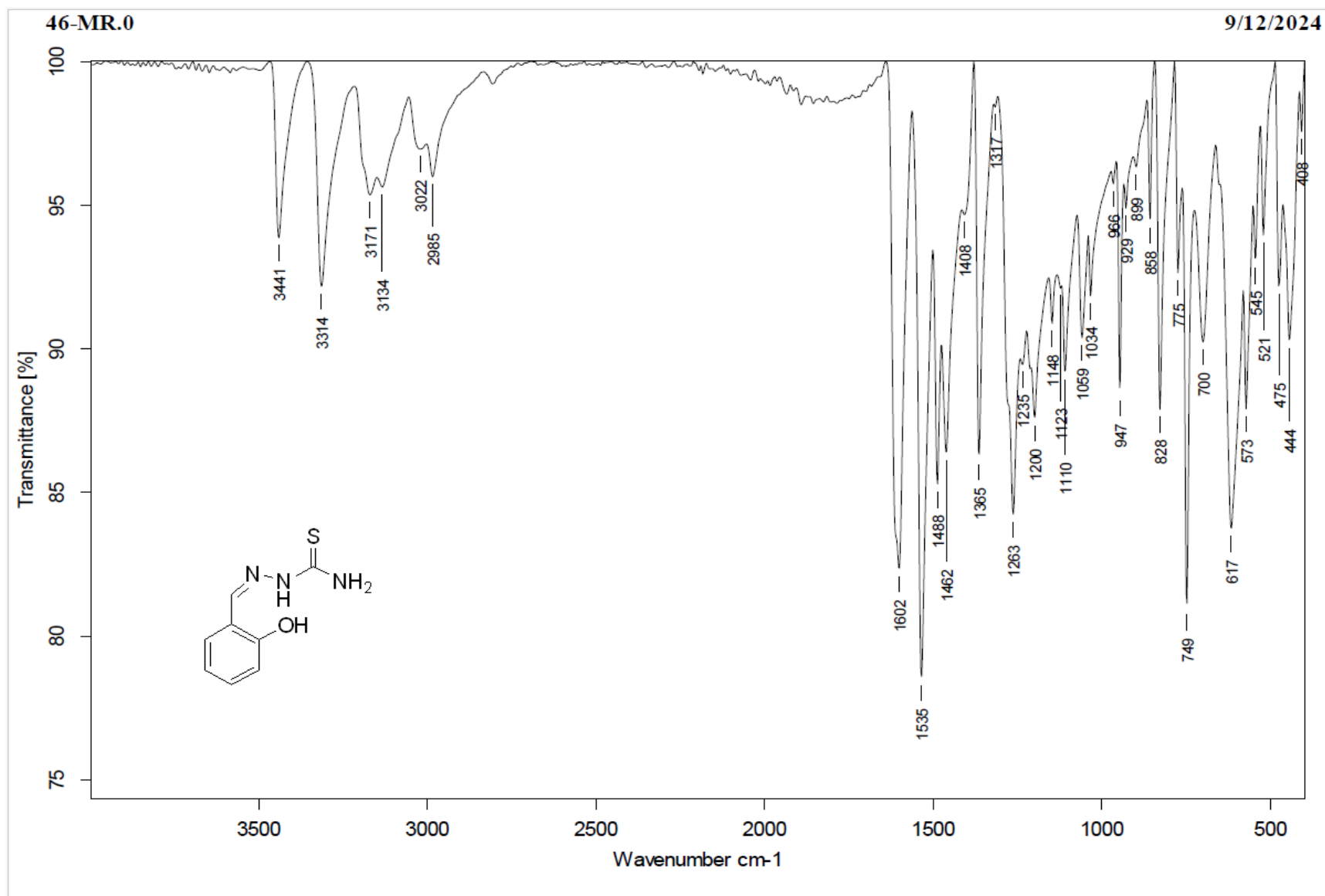
Figure. S1d A: IR spectrum of compound 1d
