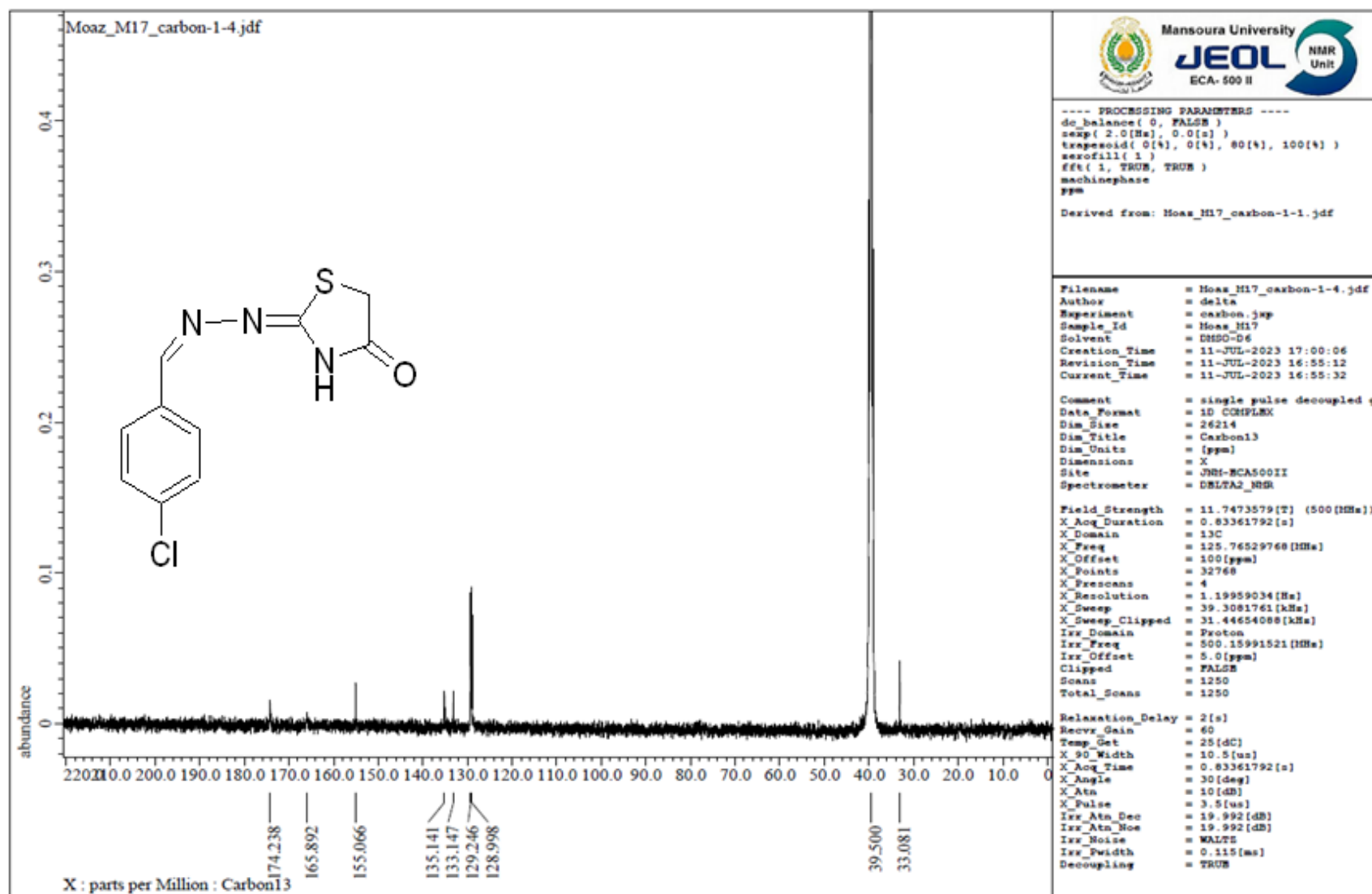
Figure. S2a C: ^{13}\text{C} -NMR spectrum of compound 2a
