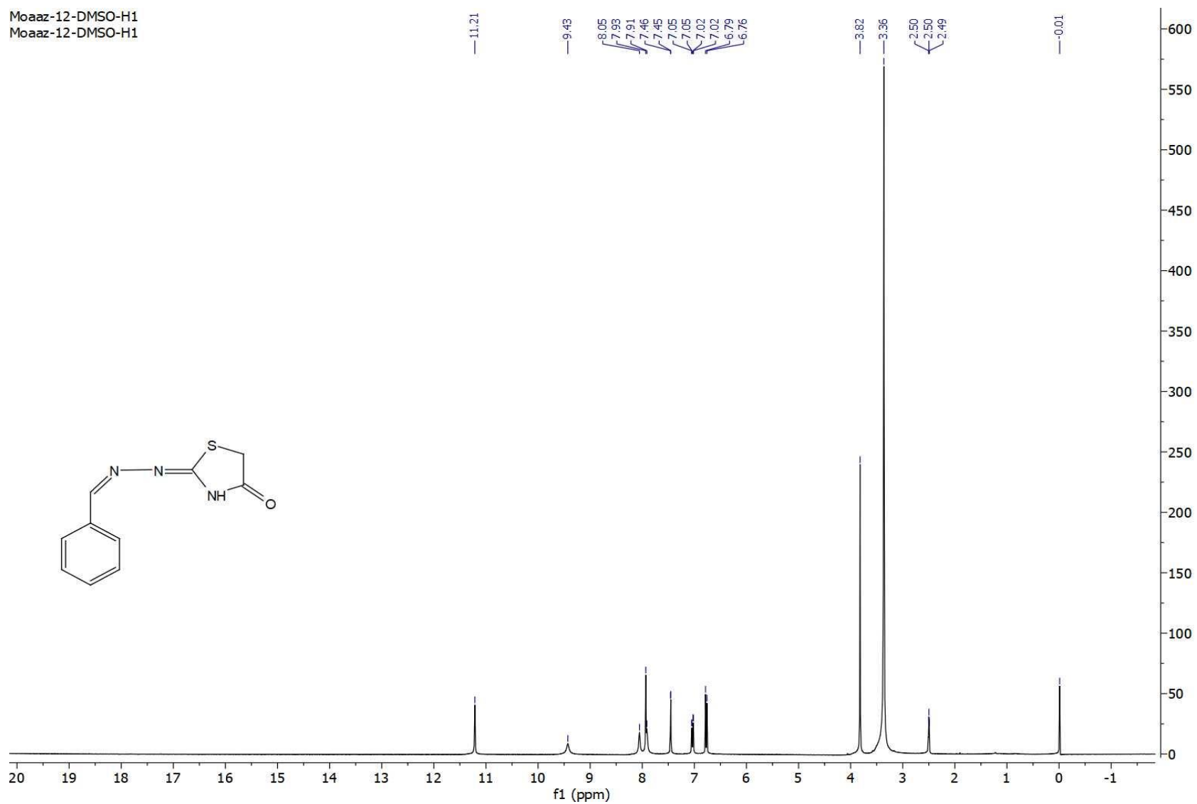
Figure. S2b B: 1 H-NMR spectrum of compound 2b
