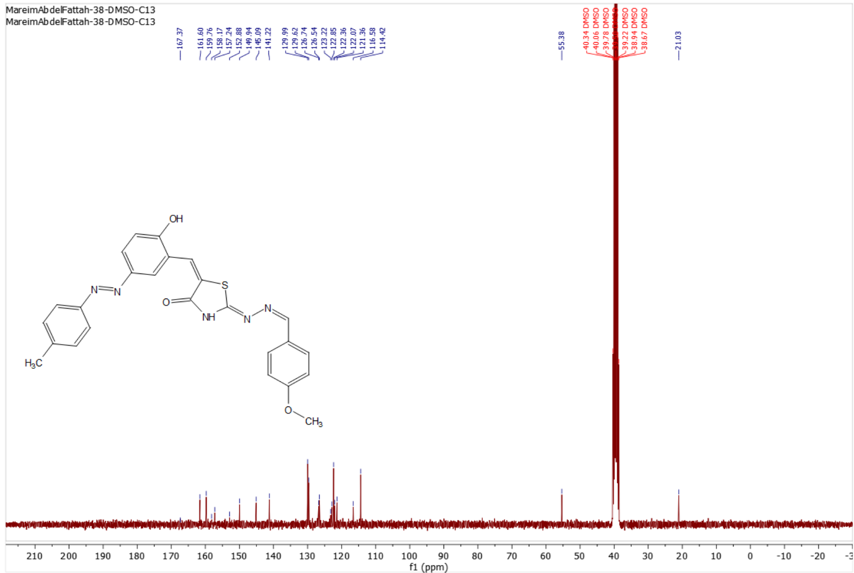
Figure. S6b C: 13 C-NMR spectrum of compound 6b (dye 6 ).
