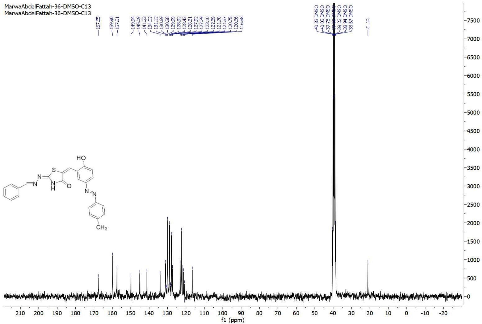
Figure. S5b C: 13 C-NMR spectrum of compound 5b (dye 4 ).
