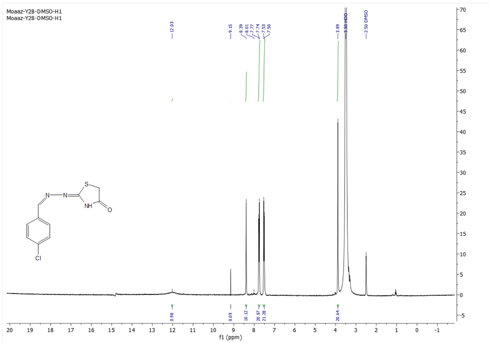
Figure. S2a B: ^1\text{H} -NMR spectrum of compound 2a
