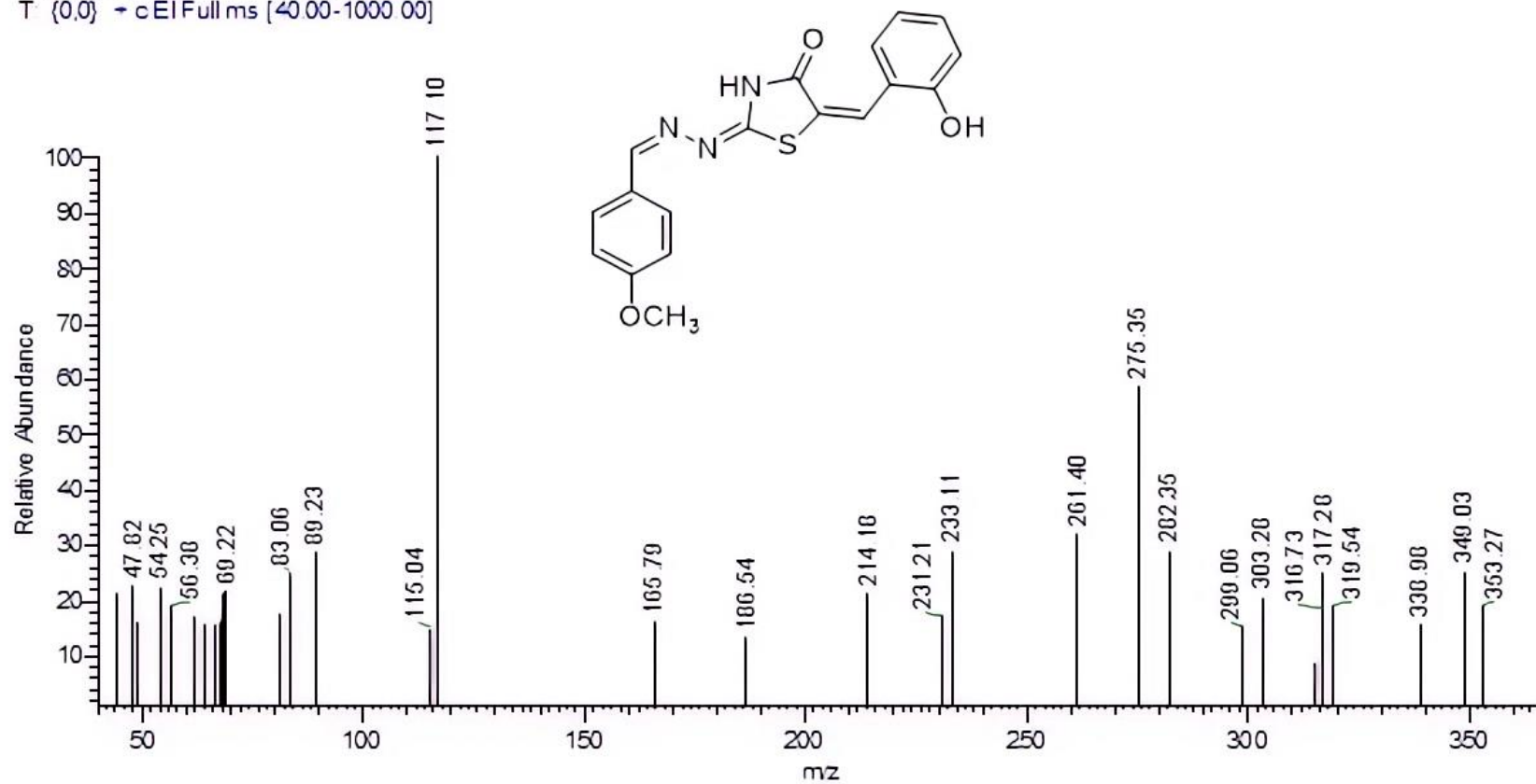
Figure. S3c D: Mass spectrum of compound 3c.
