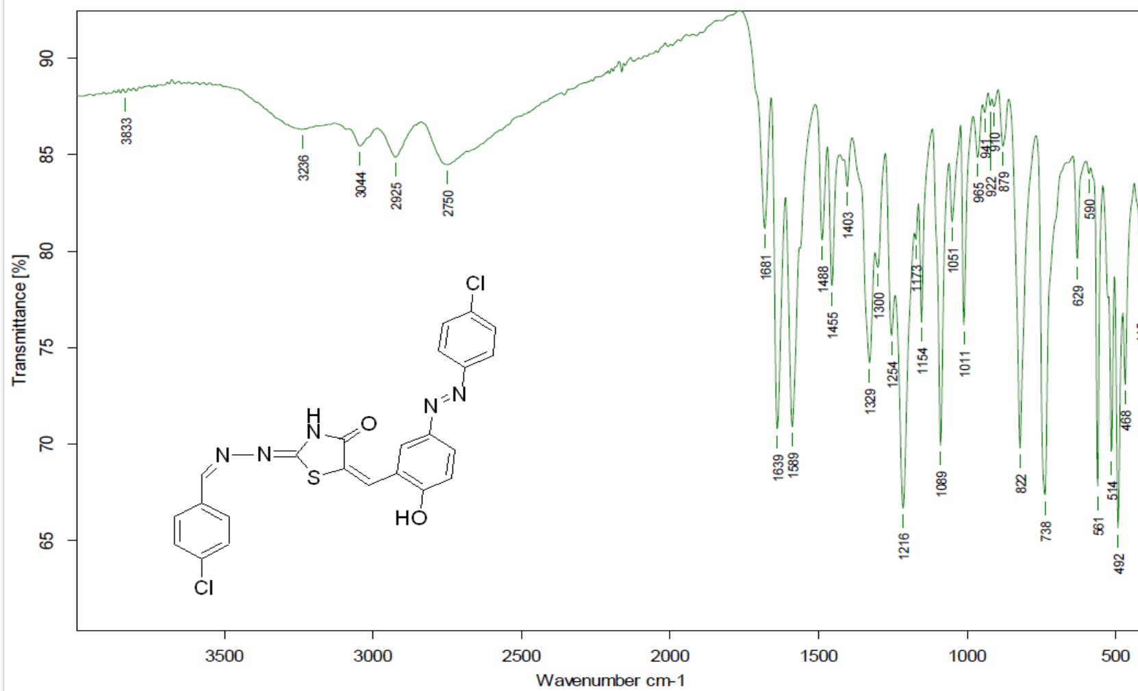
Figure. S4a A: IR spectrum of compound 4a (dye 1).
