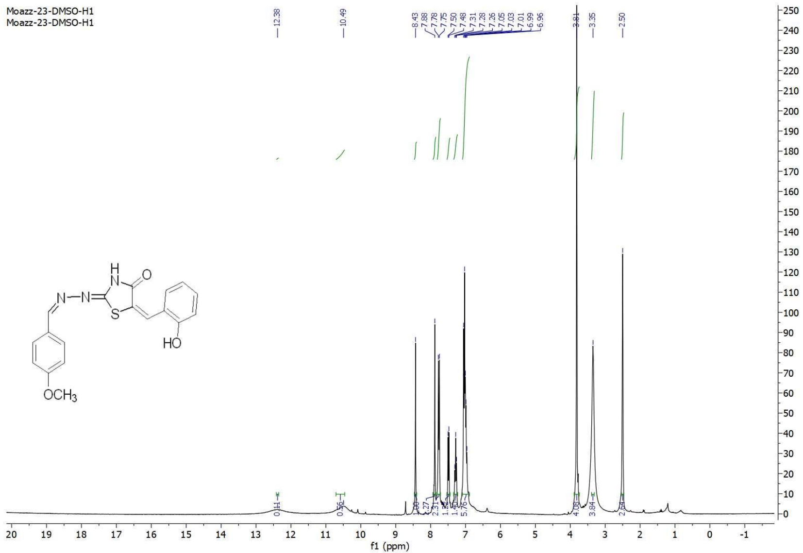
Figure. S3c B: ^1\text{H} -NMR spectrum of compound 3c
