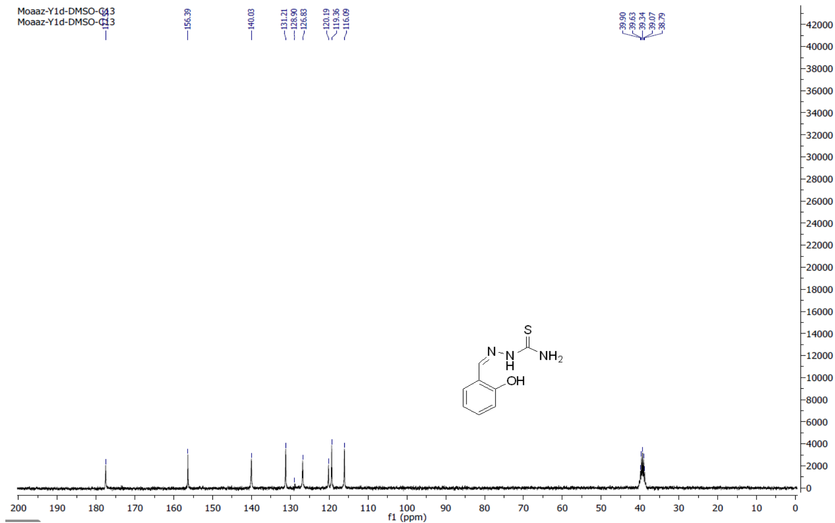
Figure. S1d C: ^{13}\text{C} -NMR spectrum of compound 1d
