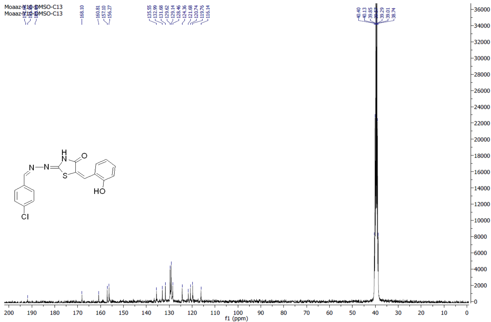
Figure. S3a C: ^{13}\text{C} -NMR spectrum of compound 3a
