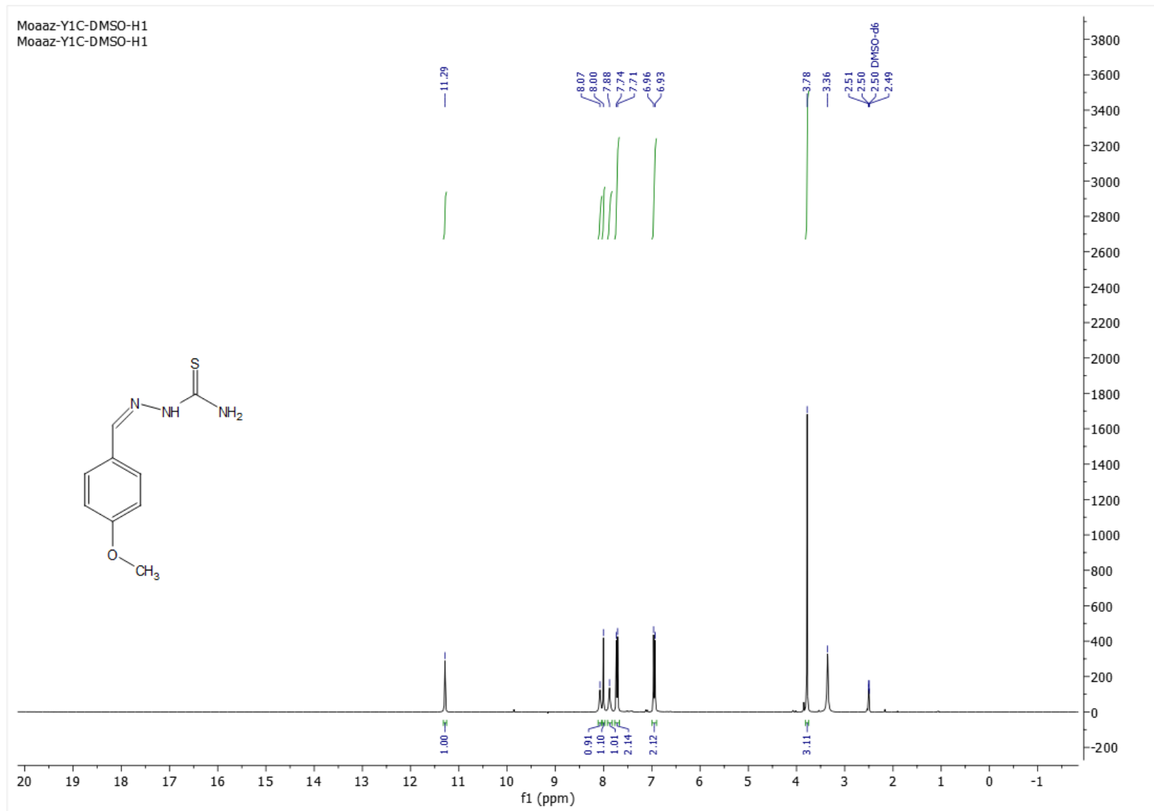
Figure. S1c B: 1 H-NMR spectrum of compound 1c
