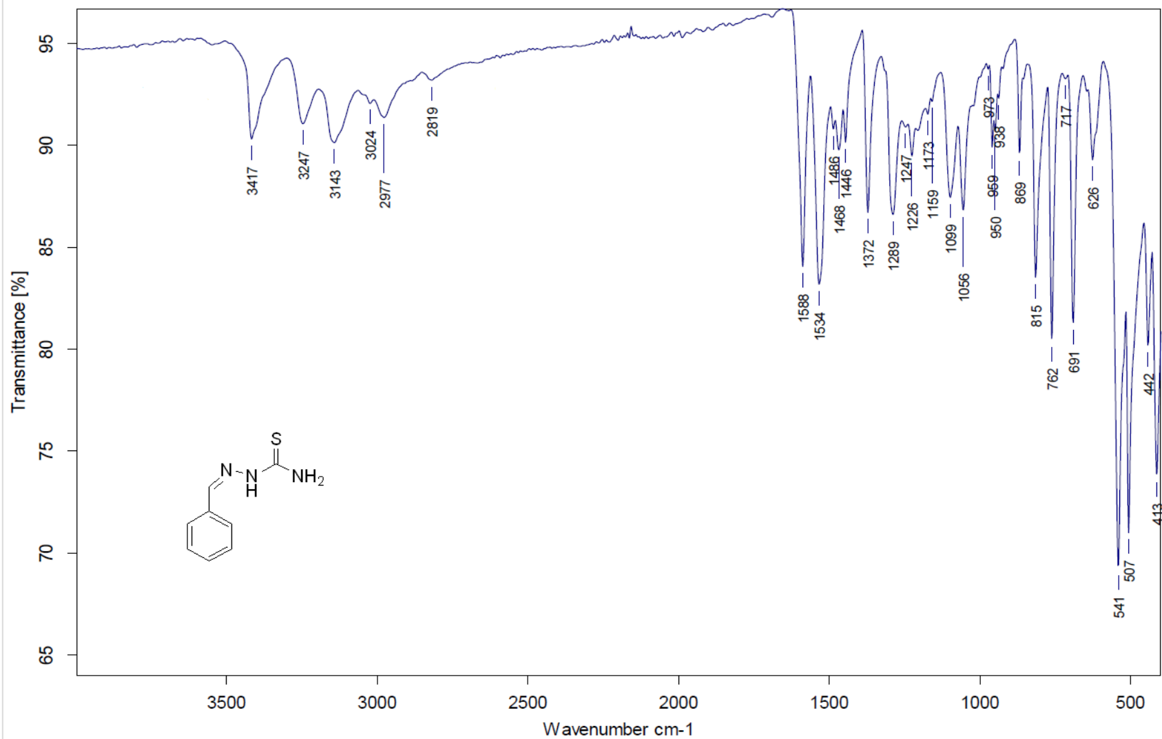
Figure. S1b A: IR spectrum of compound 1b
