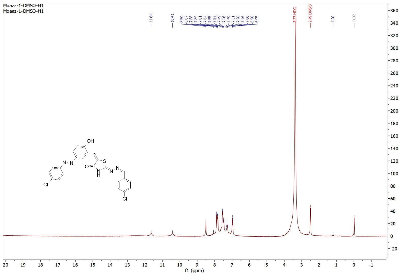
Figure. S4a B: ^1\text{H} -NMR spectrum of compound 4a (dye 1 ).
