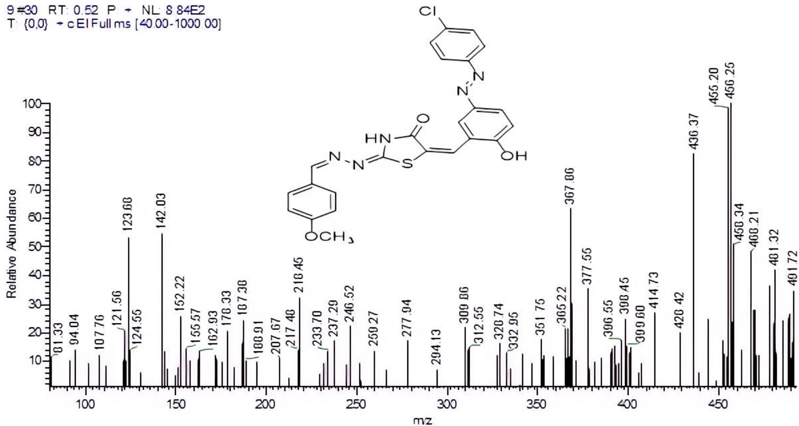
Figure. S6a D: Mass spectrum of compound 6a(dye 5).
