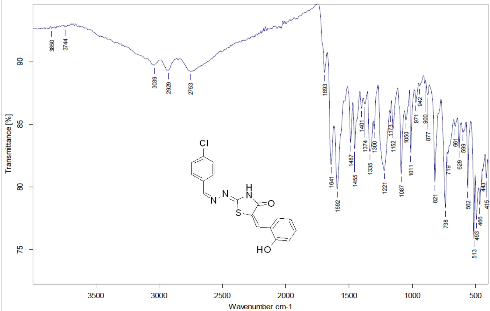
Figure. S3a A: IR spectrum of compound 3a
