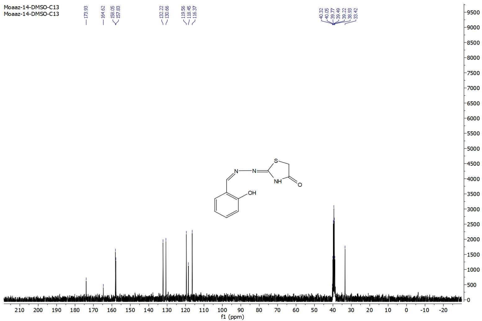
Figure. S2d C: ^{13}\text{C} -NMR spectrum of compound 2d
