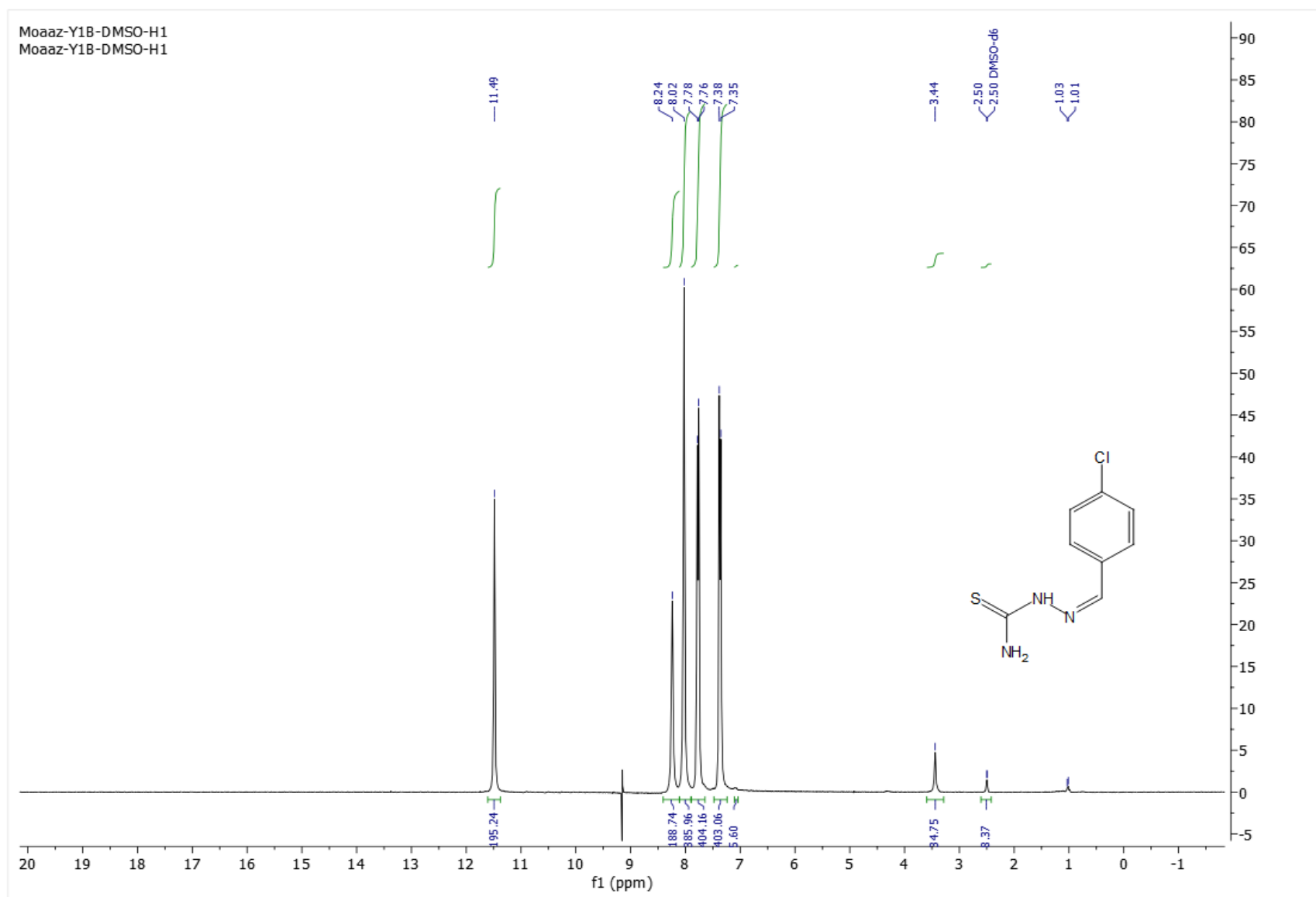
Figure. S1a B: ^1\text{H} -NMR spectrum of compound 1a
