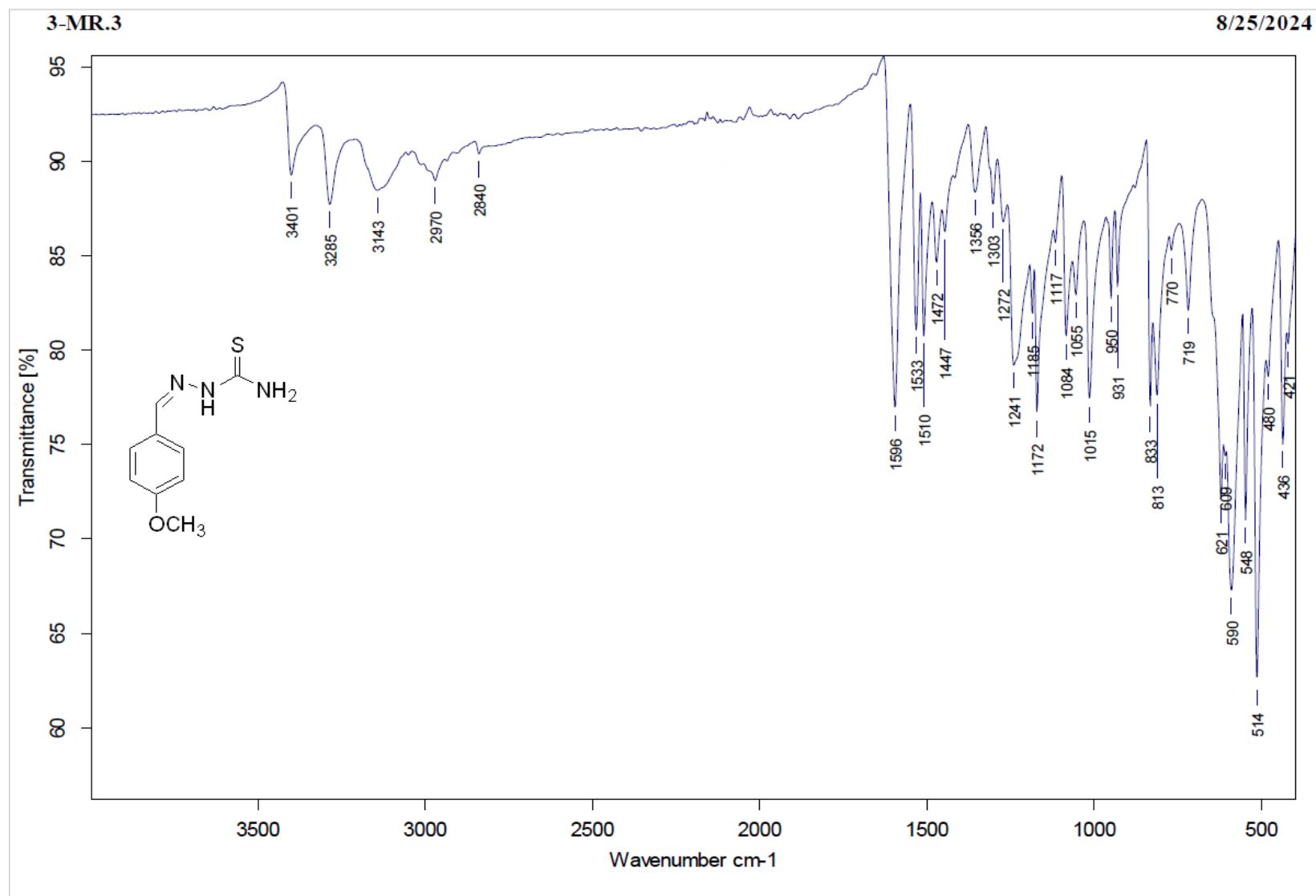
Figure. S1c A: IR spectrum of compound 1c
