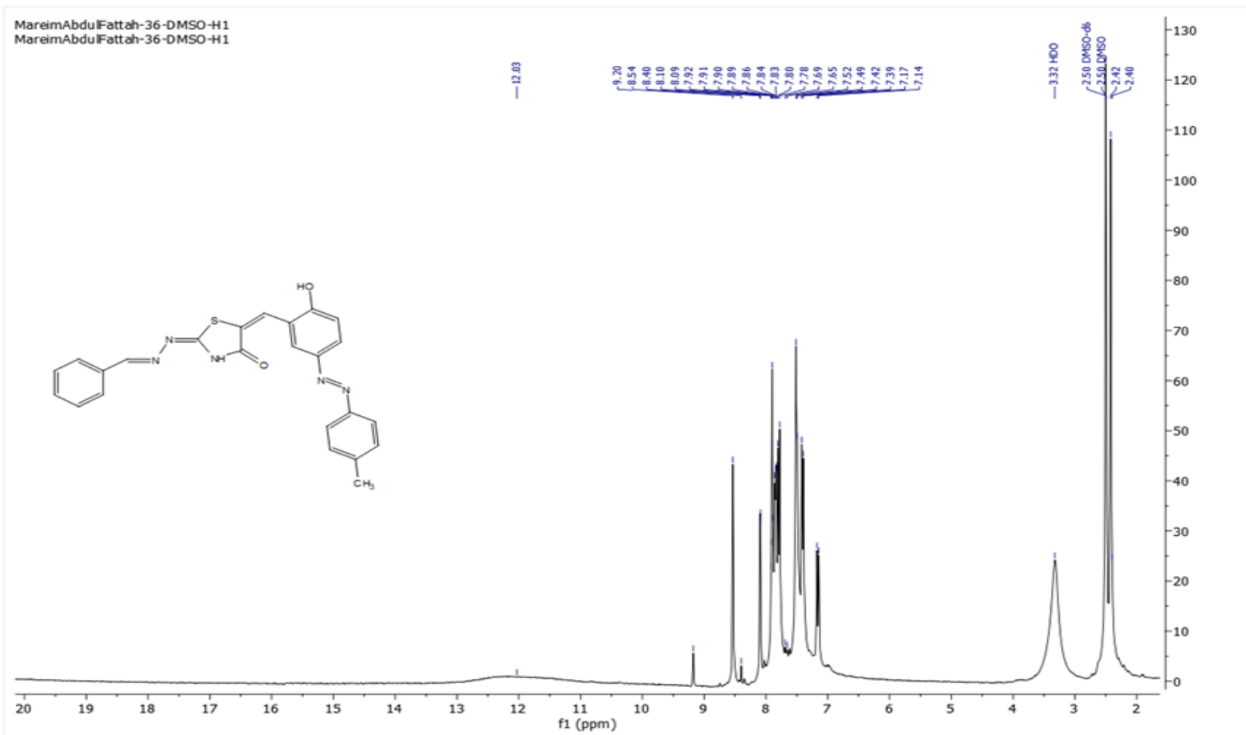
Figure. S5b B: 1 H-NMR spectrum of compound 5B(dye 4).
