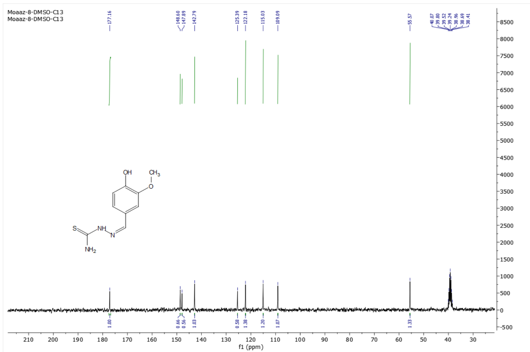
Figure. S1fC: 13 C-NMR spectrum of compound 1f
