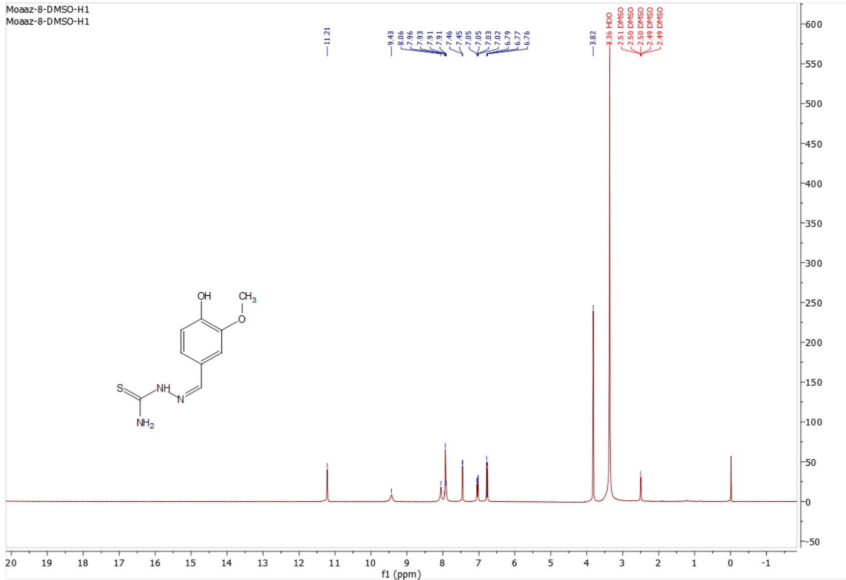
Figure. S1fB: 1 H-NMR spectrum of compound 1f
