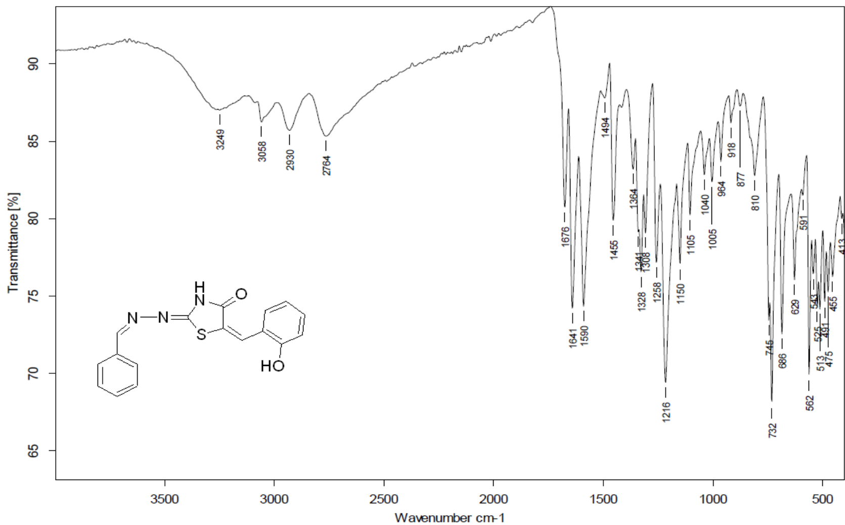
Figure. S3b A: IR spectrum of compound 3b
