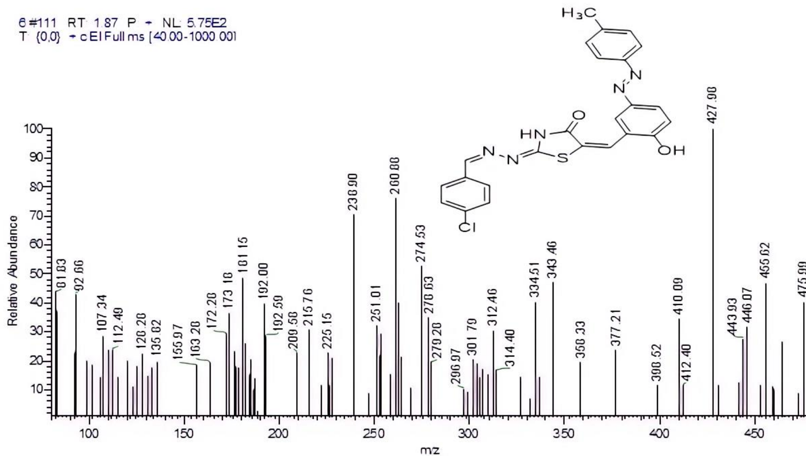
Figure. S4b D: Mass spectrum of compound 4b(dye 2).
