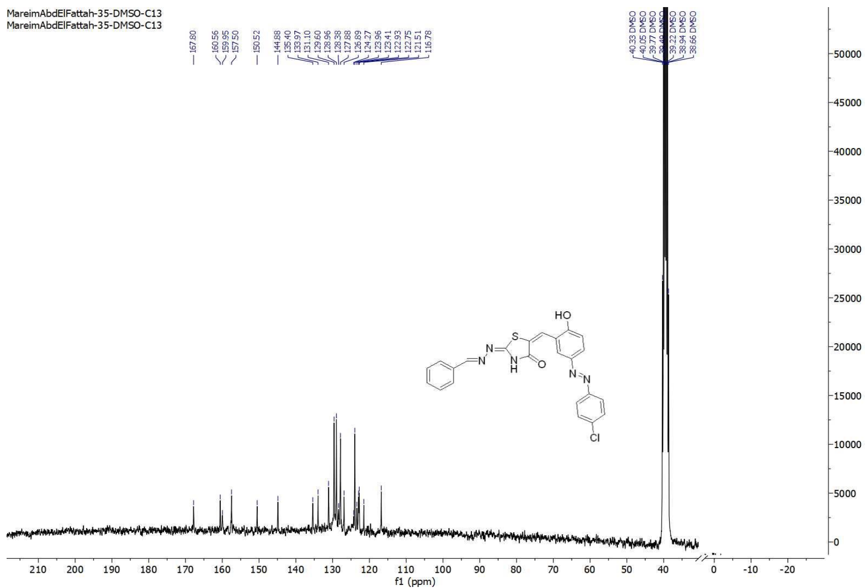
Figure. S5a C: ^{13}\text{C} -NMR spectrum of compound 5a (dye 3 ).
