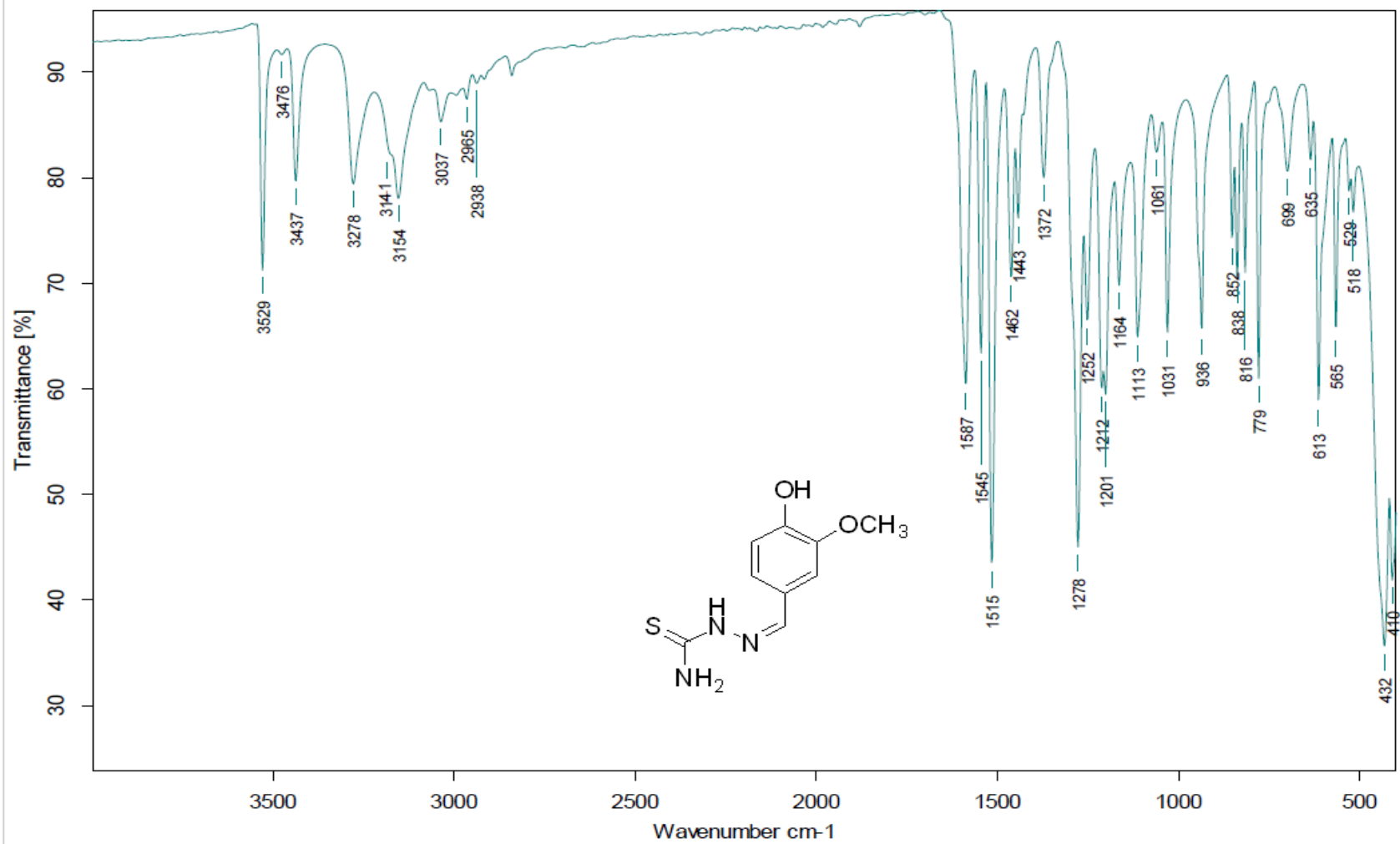
Figure. S1f A: IR spectrum of compound 1f
