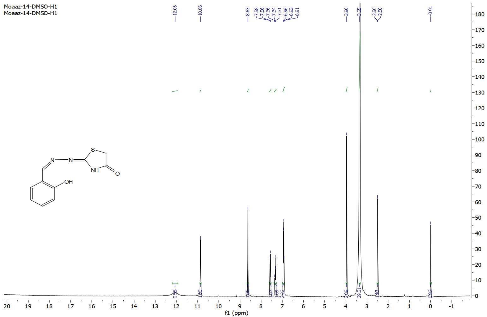
Figure. S2d B: 1 H-NMR spectrum of compound 2d
