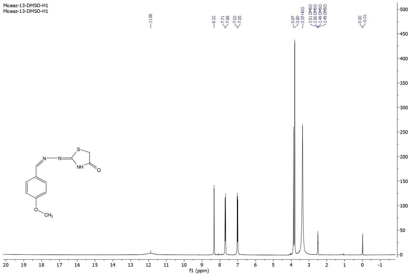
Figure. S2c B: 1 H-NMR spectrum of compound 2c
