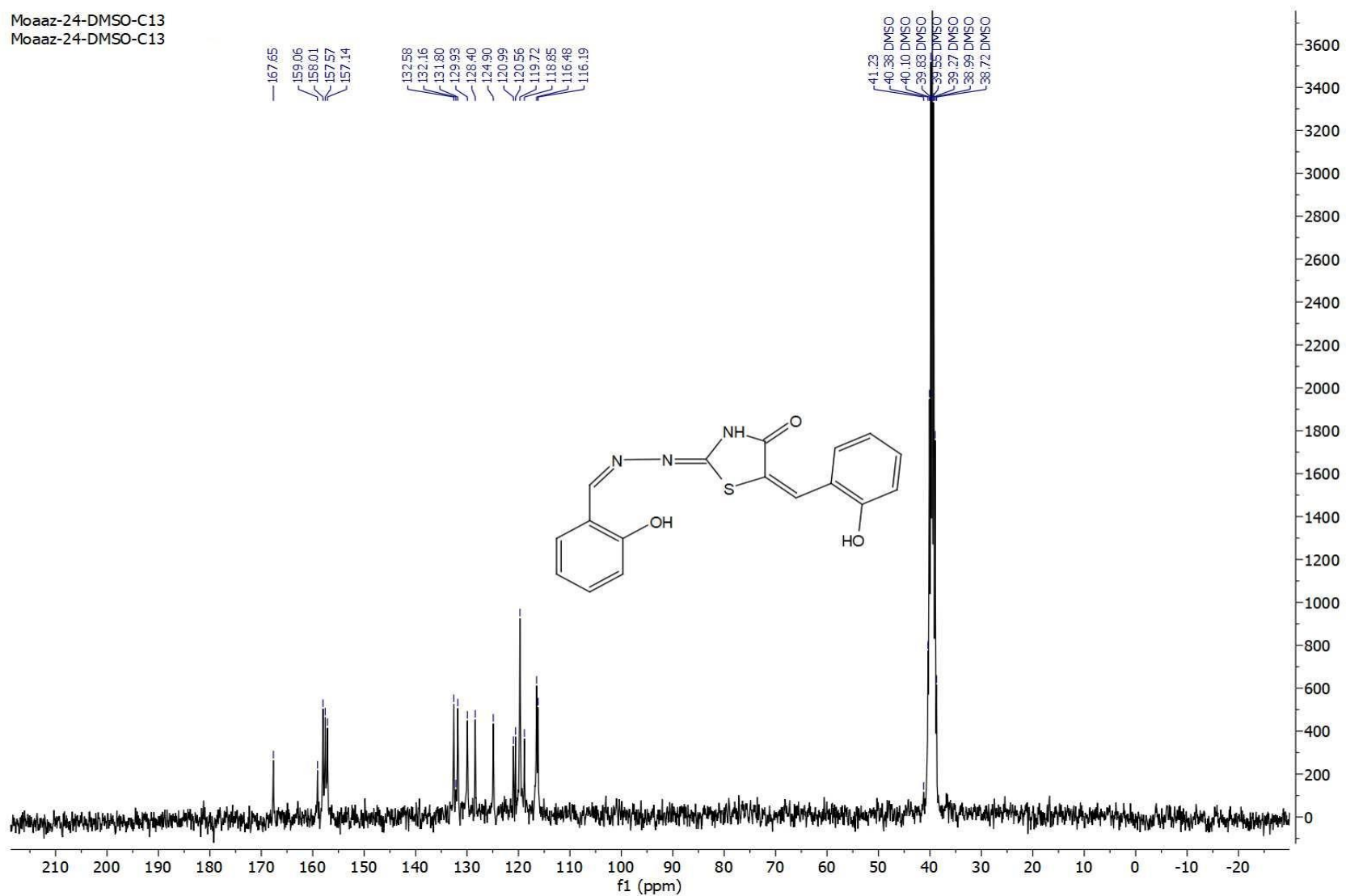
Figure. S3d C: ^{13}\text{C} -NMR spectrum of compound 3d .
