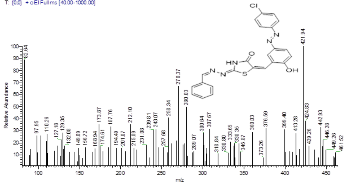
Figure. S5a D: Mass spectrum of compound 5a(dye 3).
