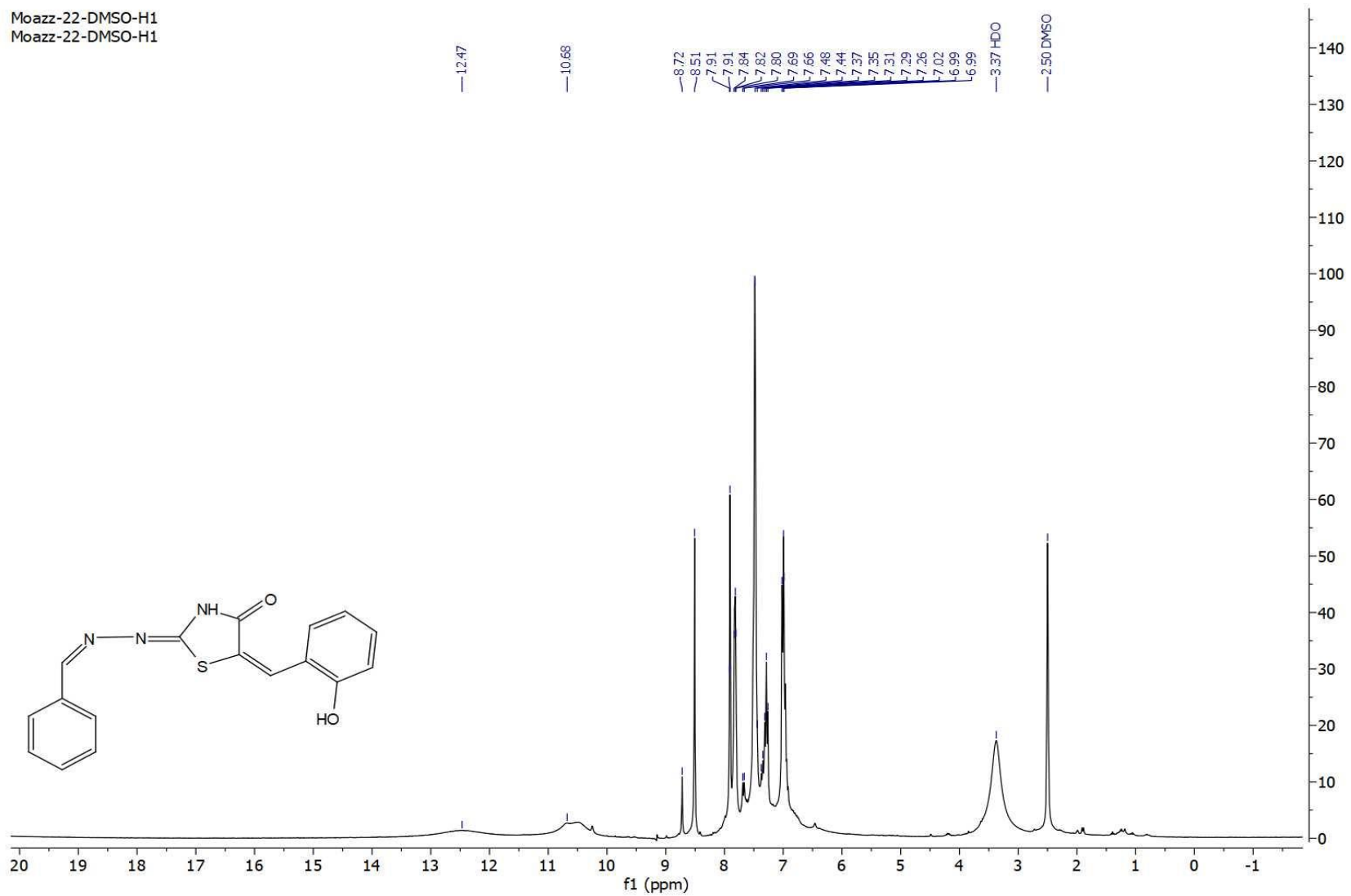
Figure. S3b B: 1 H-NMR spectrum of compound 3b
