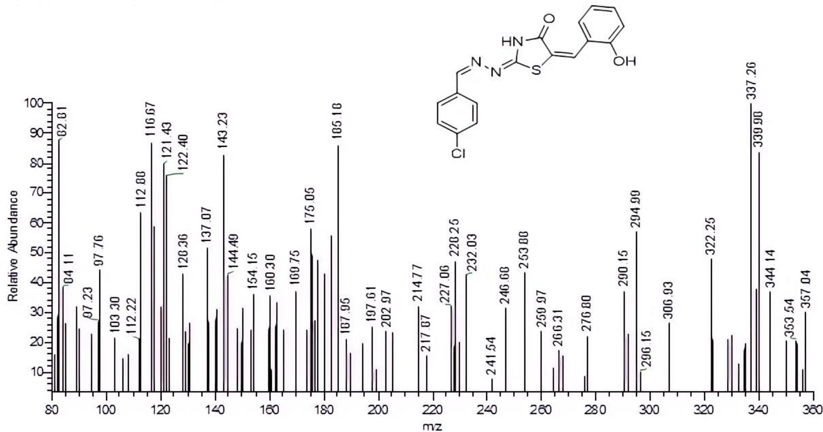
Figure. S3a D: Mass spectrum of compound 3a.
