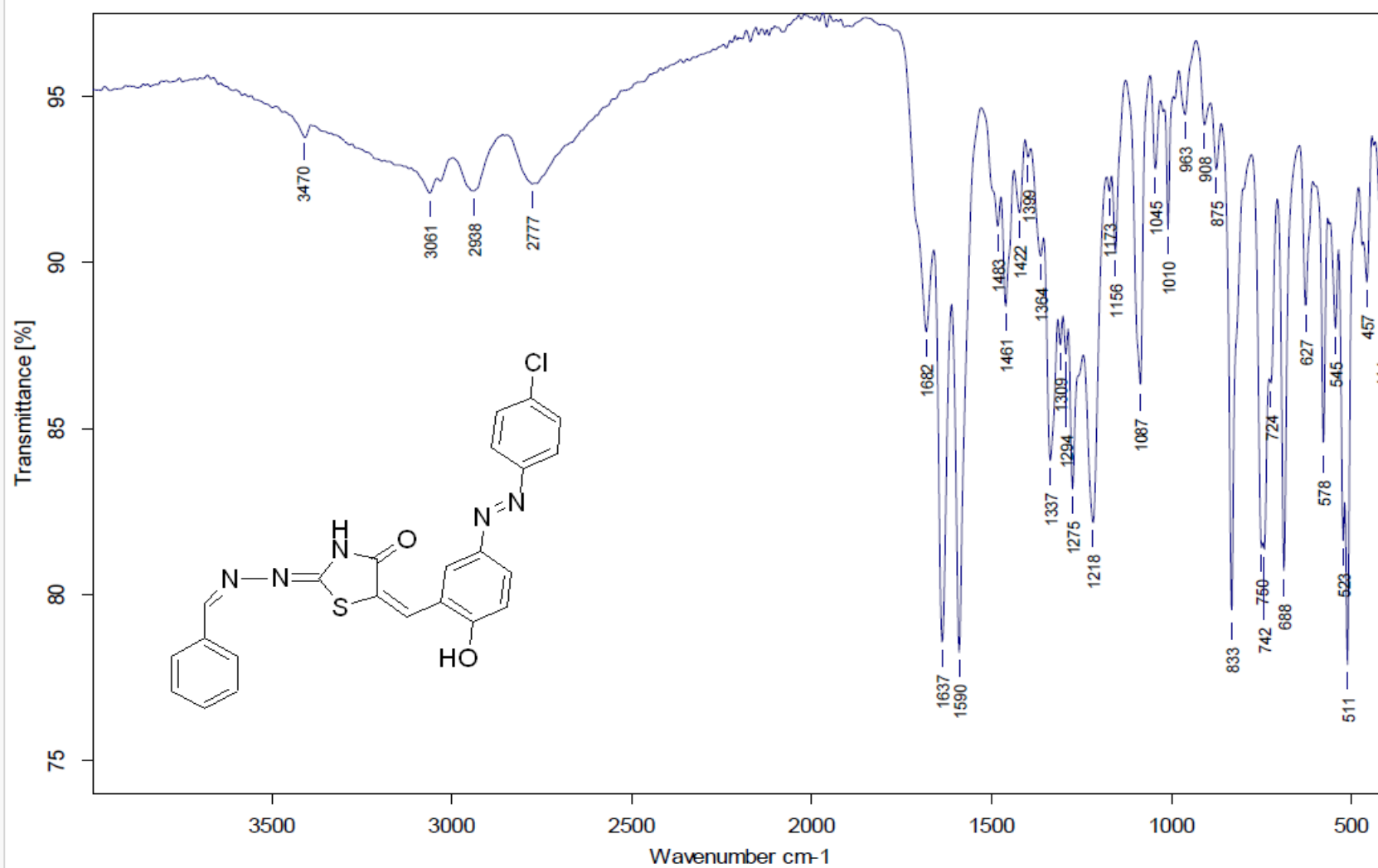
Figure. S5a A: IR spectrum of compound 5a(dye 3).
