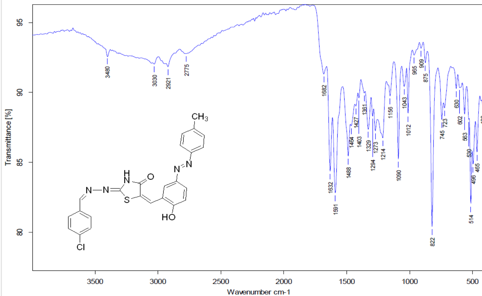
Figure. S4b A: IR spectrum of compound 4b(dye 2) .
