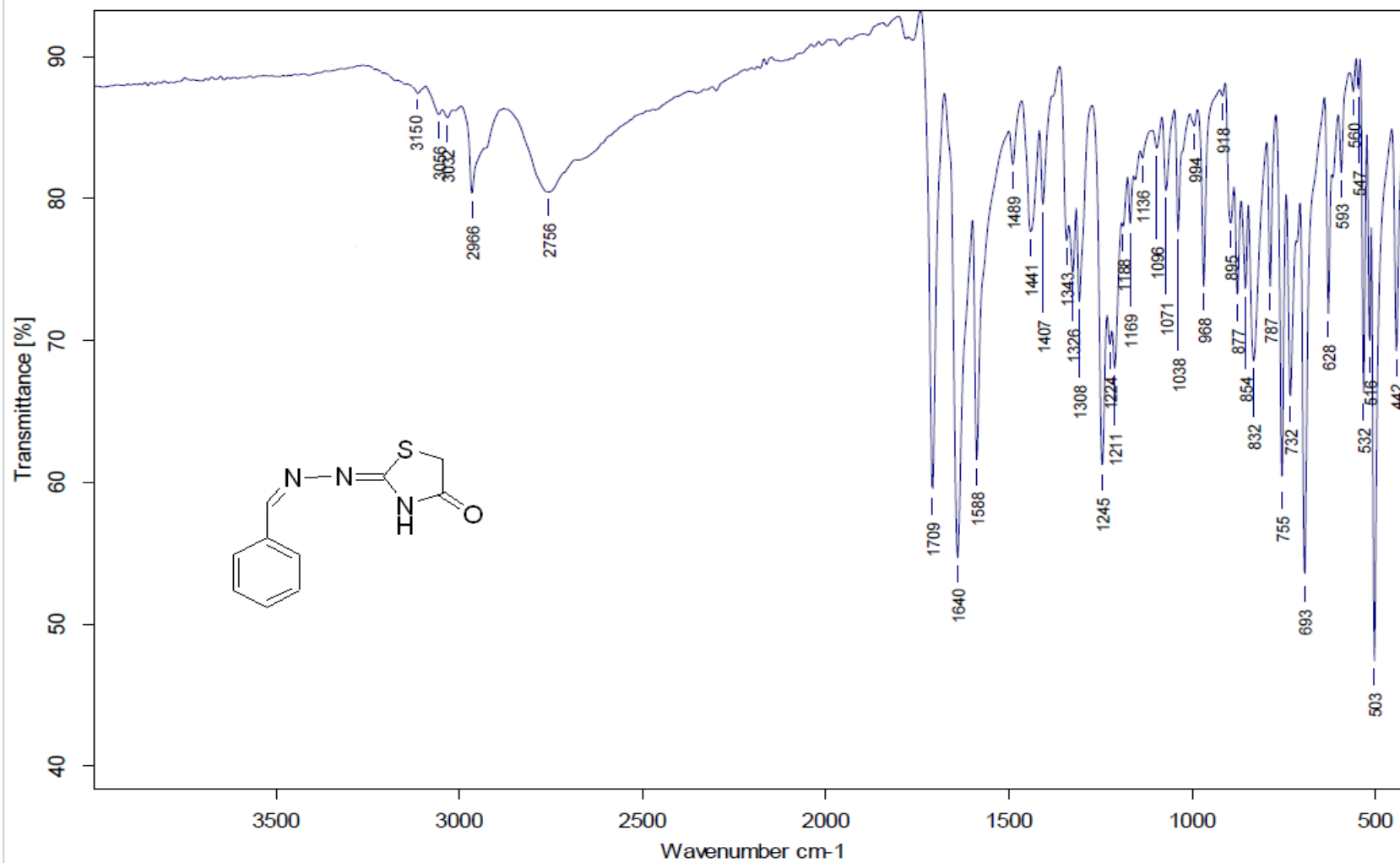
Figure. S2b A: IR spectrum of compound 2b
