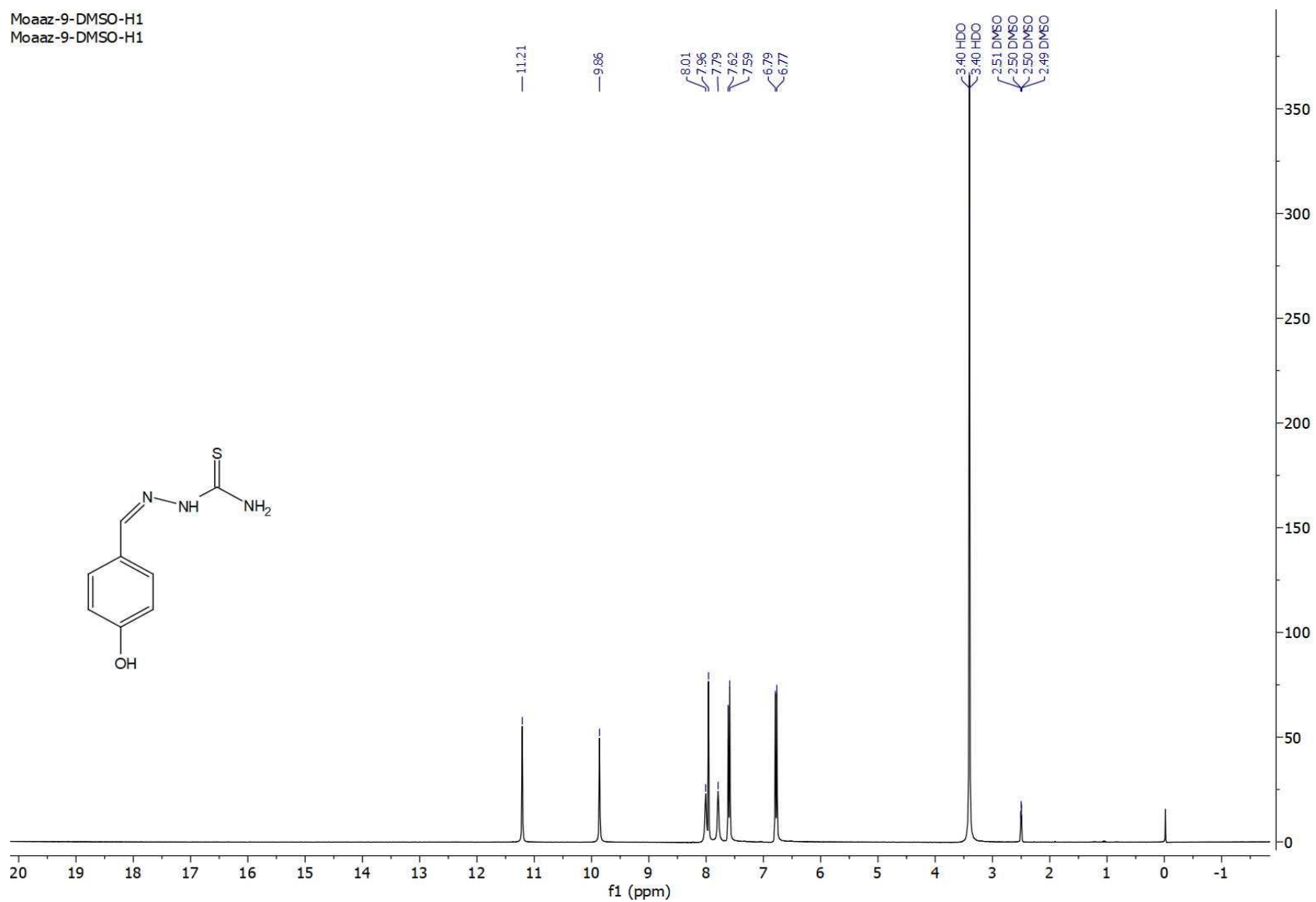
Figure. S1e B: 1 H-NMR spectrum of compound 1e
