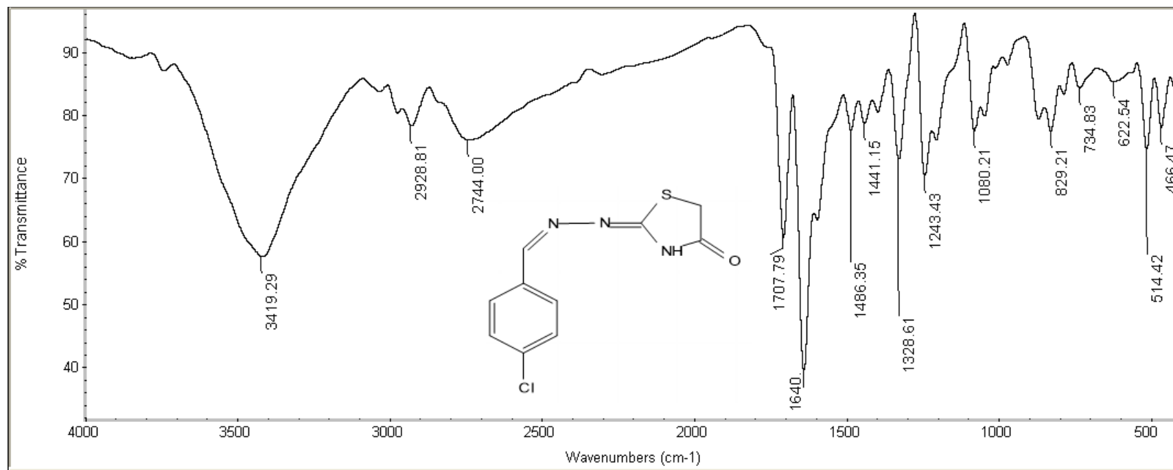
Figure. S2a A: IR spectrum of compound 2a
