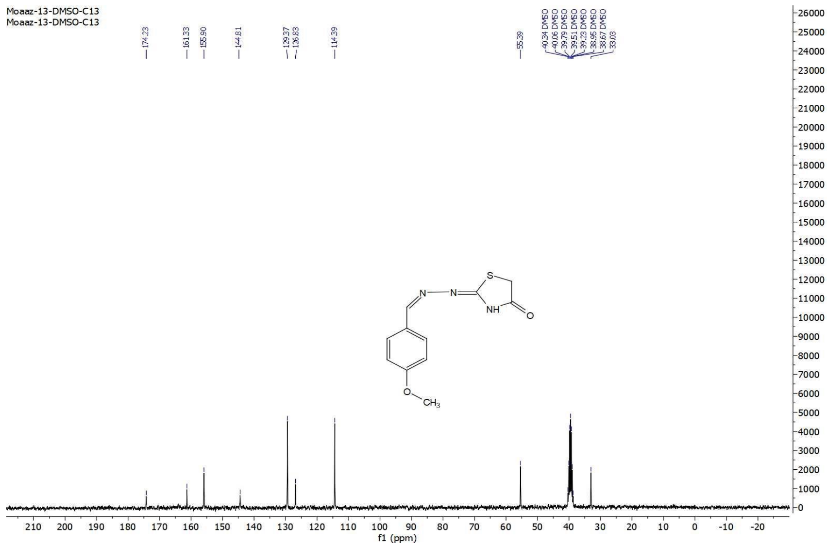
Figure. S2c C: ^{13}\text{C} -NMR spectrum of compound 2c
