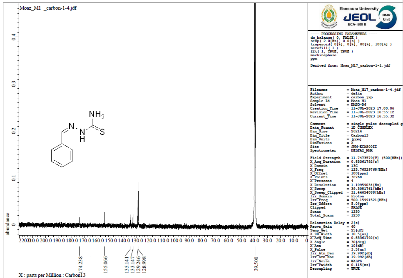
Figure. S1b C: ^{13}\text{C} -NMR spectrum of compound 1b
