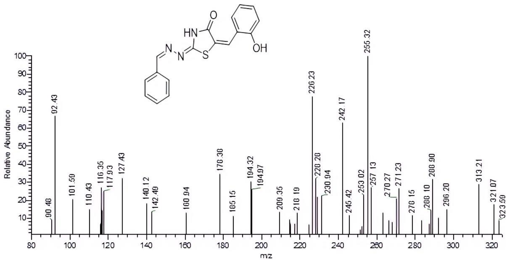
Figure. S3b D: Mass spectrum of compound 3b .
