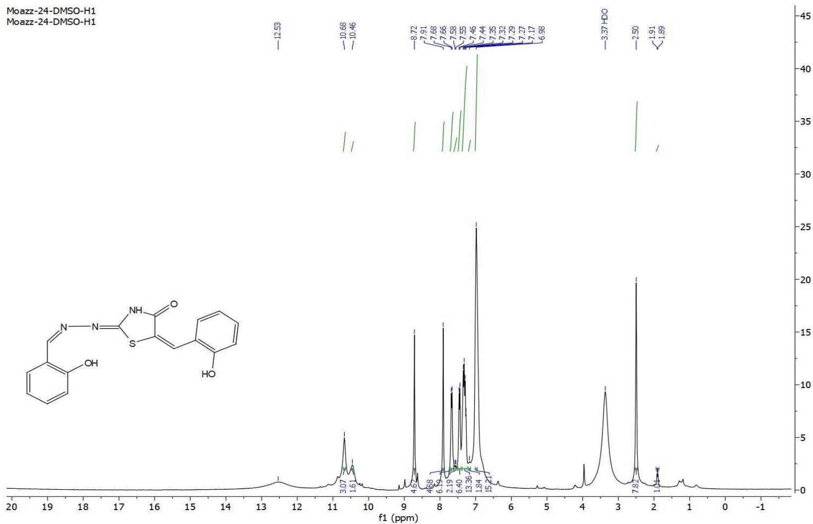
Figure. S3d B: 1 H-NMR spectrum of compound 3d
