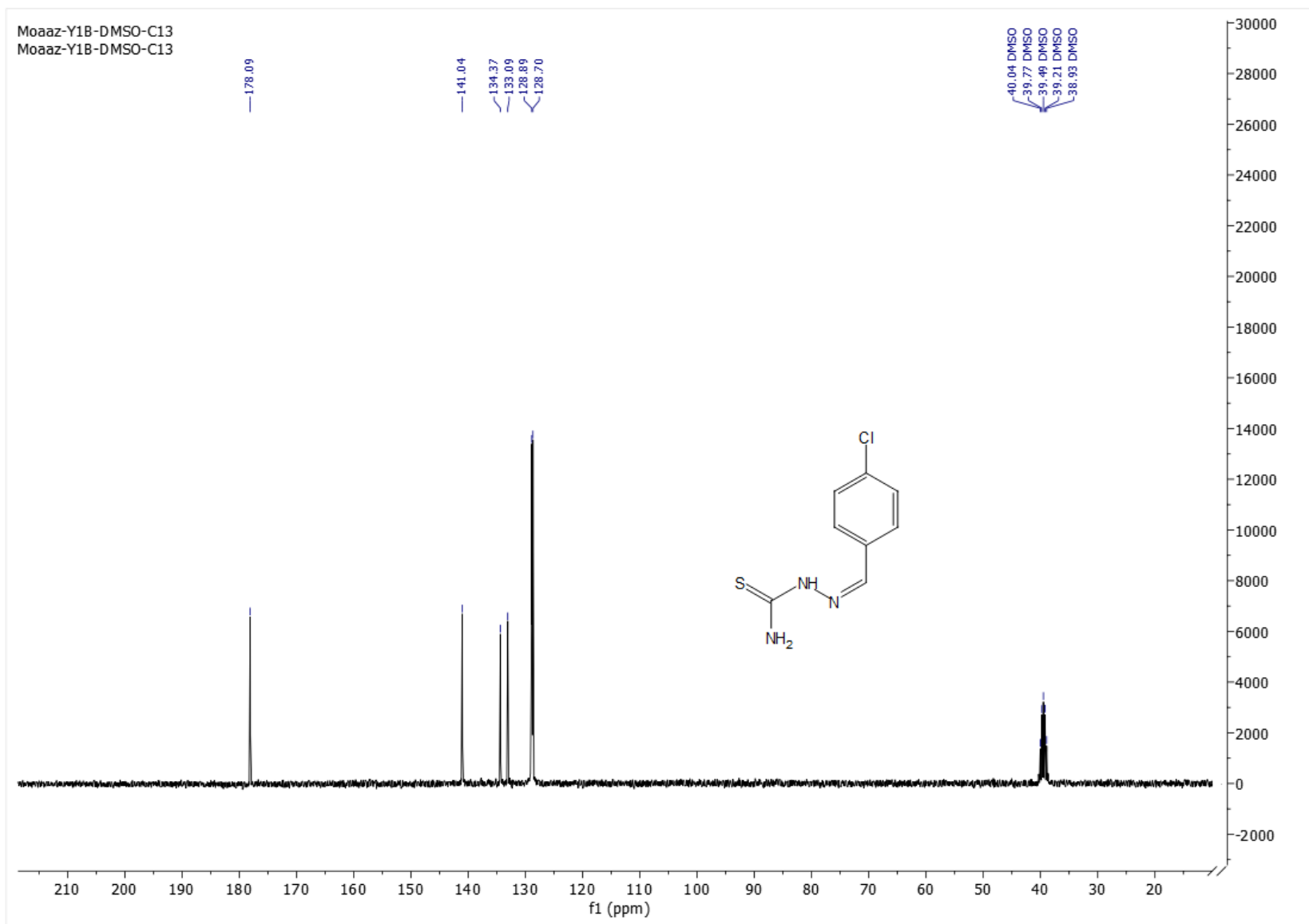
Figure. S1a C: ^{13}\text{C} -NMR spectrum of compound 1a
