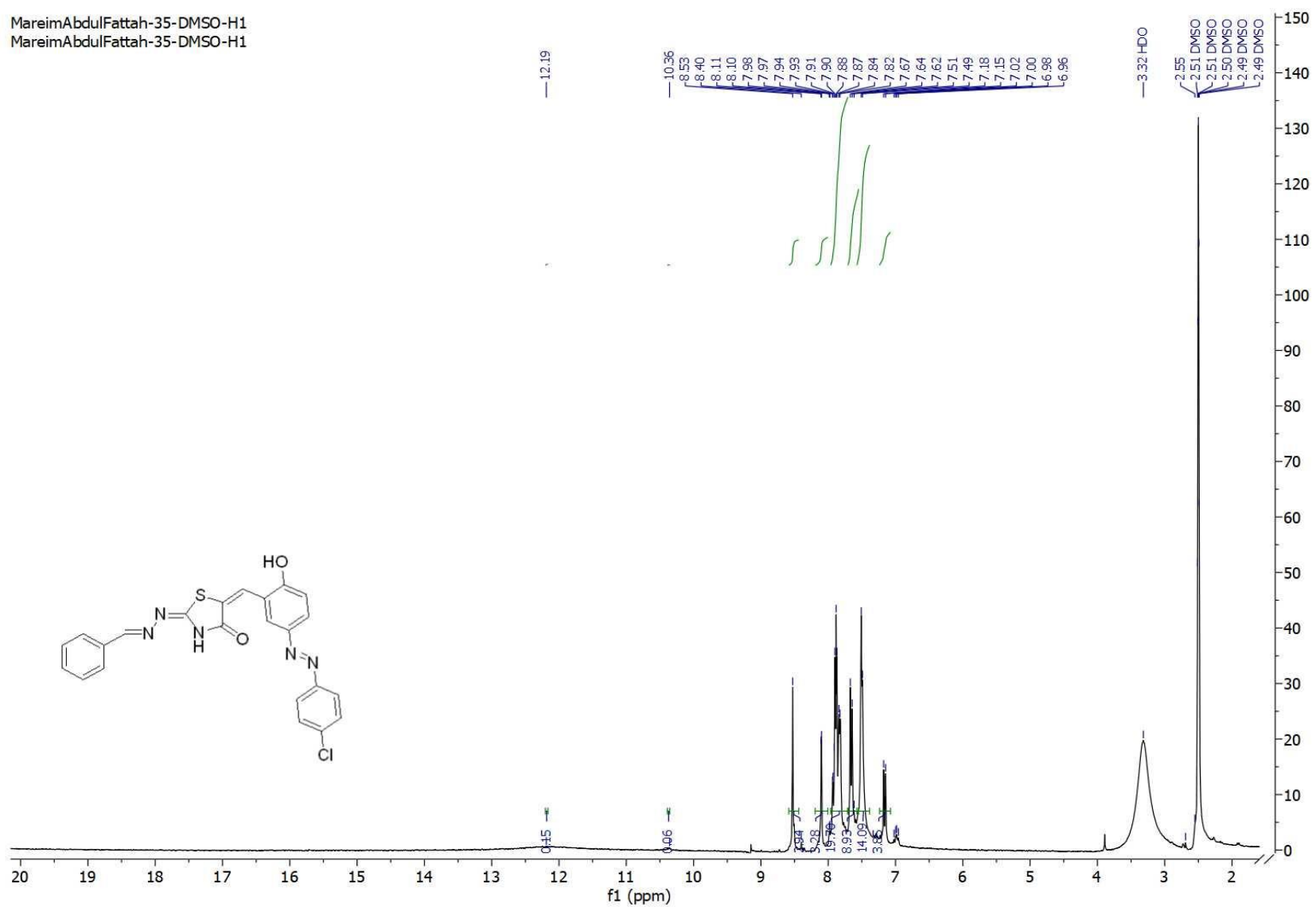
Figure. S5a B: 1 H-NMR spectrum of compound 5a (dye 3).
