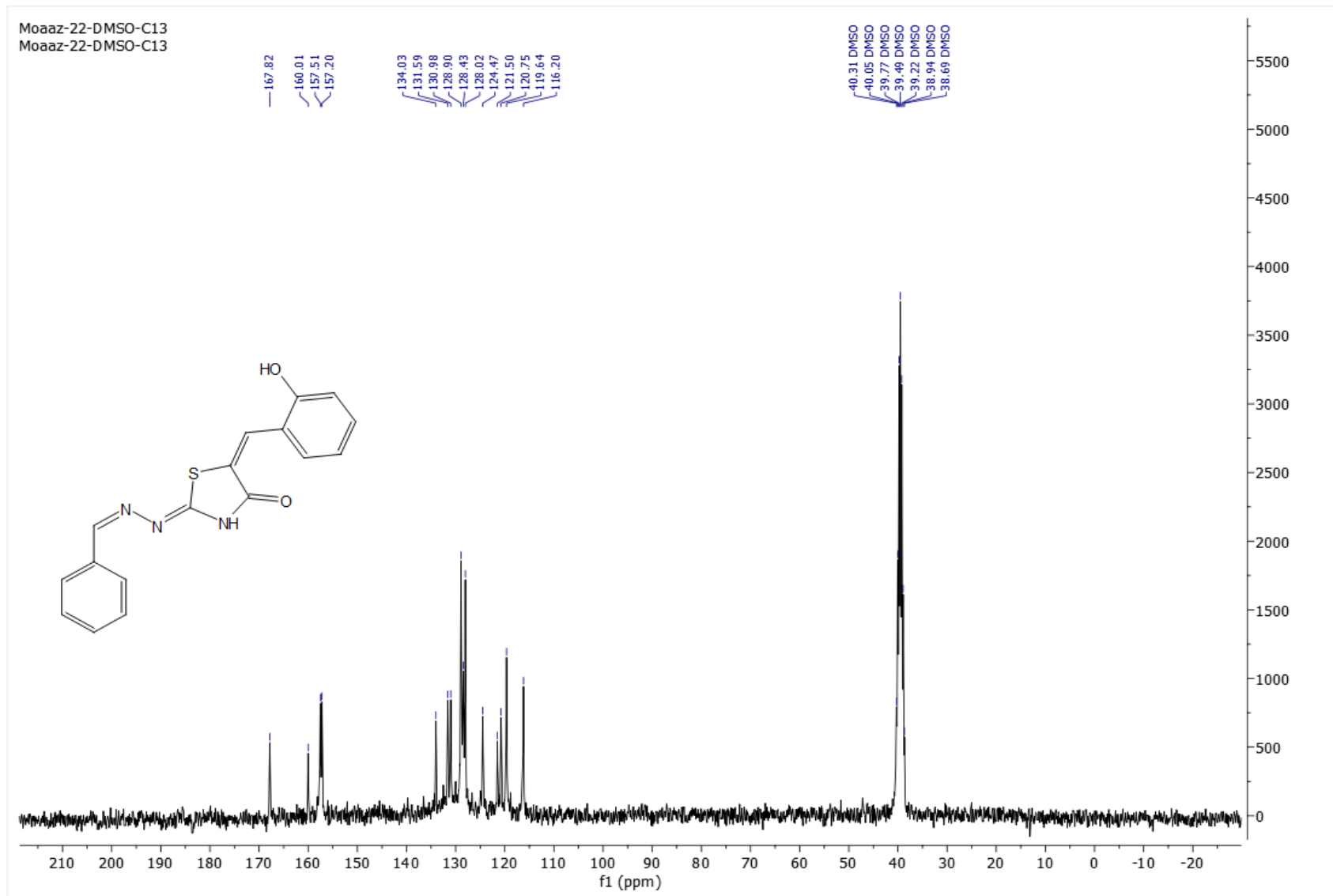
Figure. S3b C: 13 C-NMR spectrum of compound 3b .
