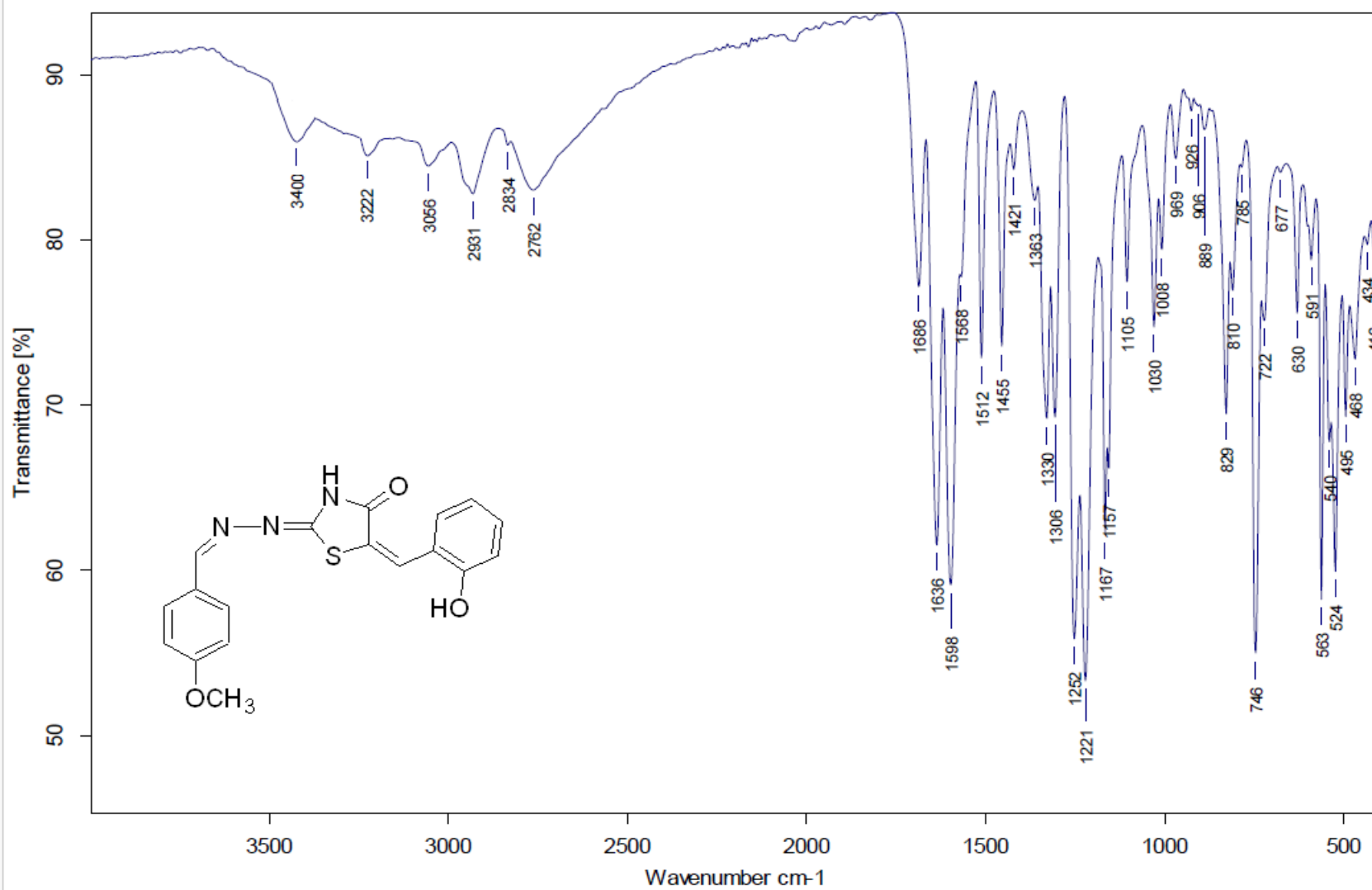
Figure. S3c A: IR spectrum of compound 3c
