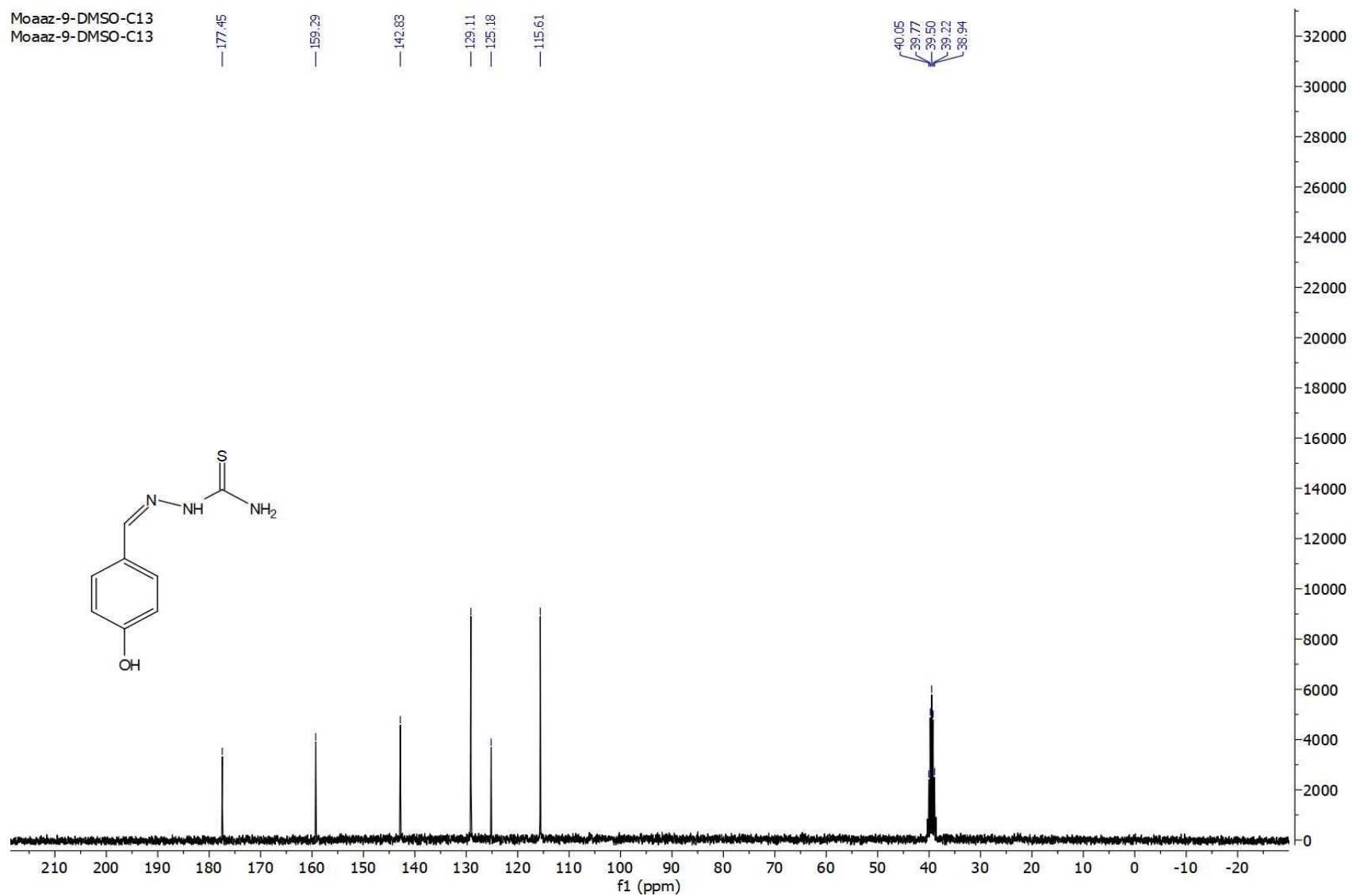
Figure. S1e C: ^{13}\text{C} -NMR spectrum of compound 1e
