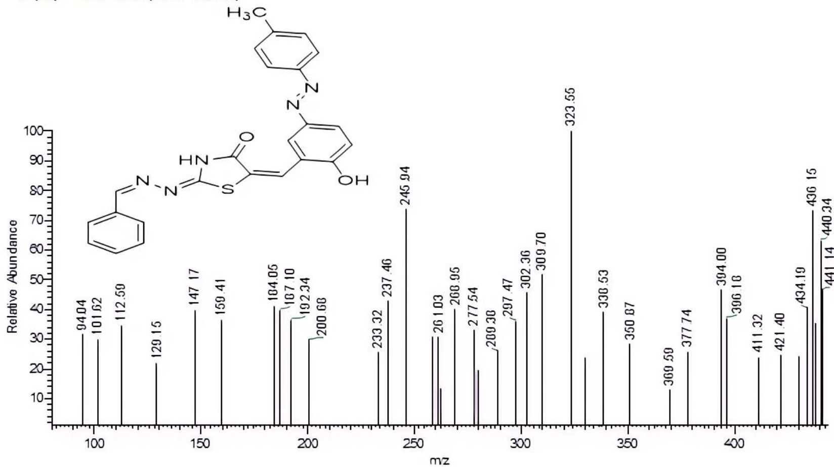
Figure. S5b D: Mass spectrum of compound 5b(dye 4).
