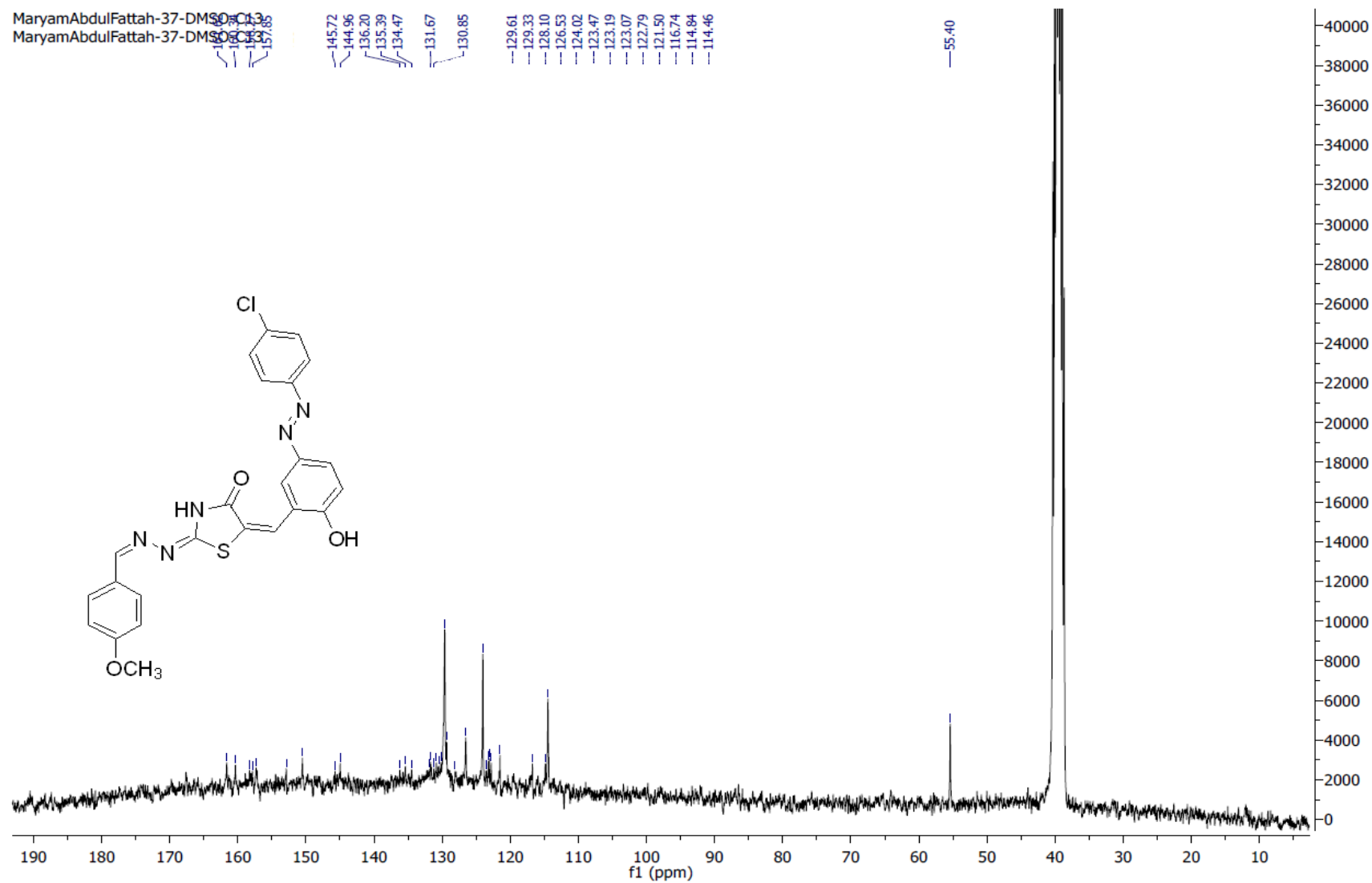
Figure. S6a C: 13 C-NMR spectrum of compound 6a (dye 5 ).
