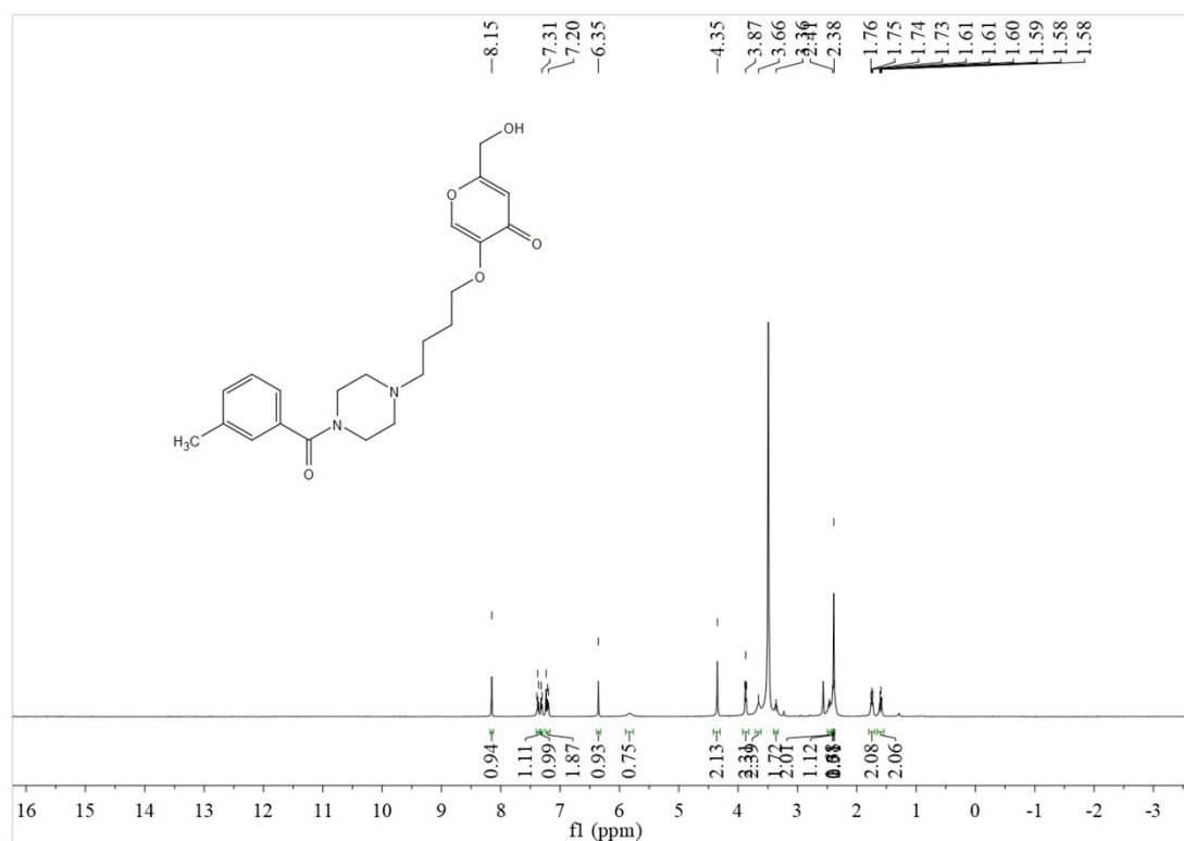
1 H NMR of 2-(hydroxymethyl)-5-(4-(4-(3-methylbenzoyl)piperazin-1-yl)butoxy)-4H-pyran-4-one (3b)
