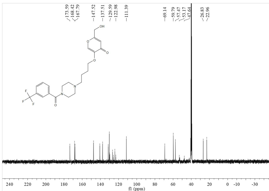
13 C NMR of 2-(hydroxymethyl)-5-(4-(4-(3-(trifluoromethyl)benzoyl)piperazin-1-yl)butoxy)-4H-pyran-4-one (3q)
