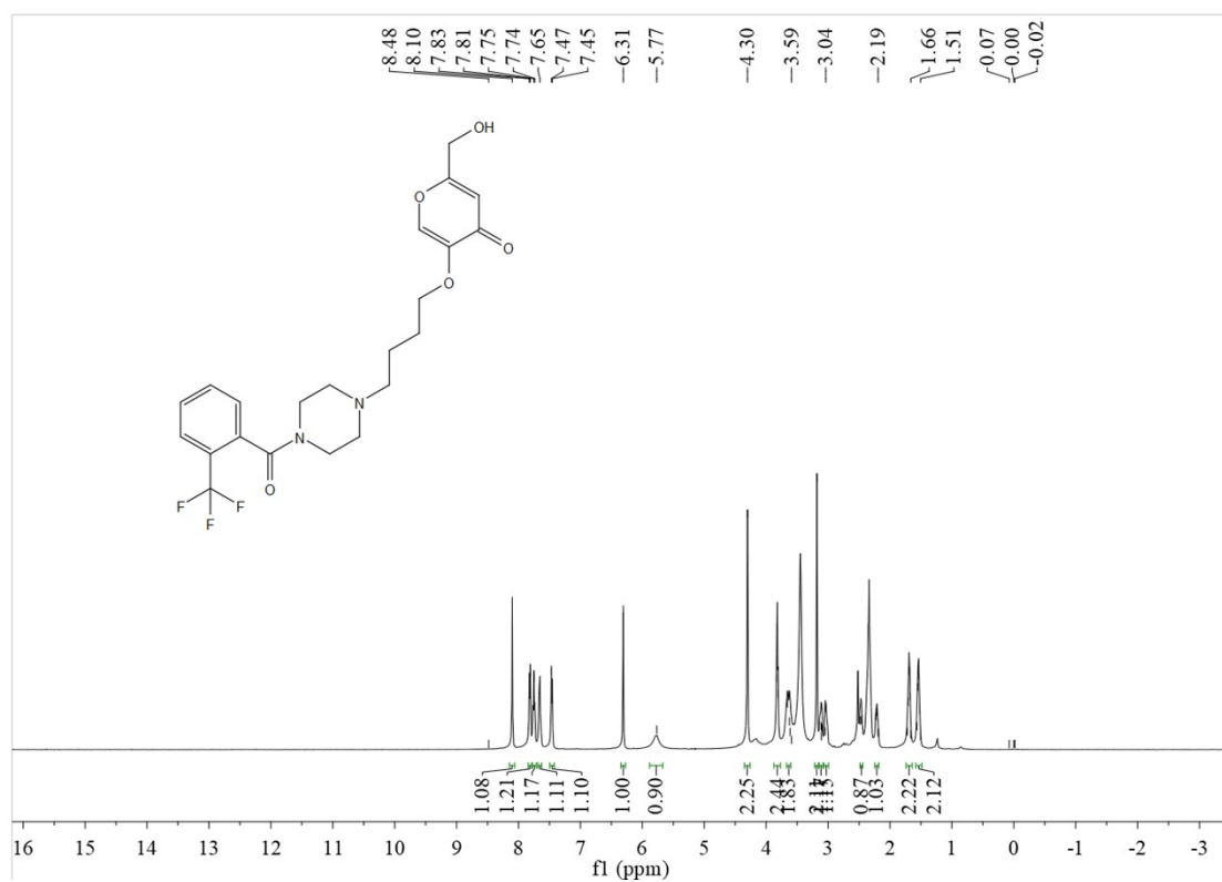
1 H NMR of 2-(hydroxymethyl)-5-(4-(4-(2-(trifluoromethyl)benzoyl)piperazin-1-yl)butoxy)-4H-pyran-4-one (3p)
