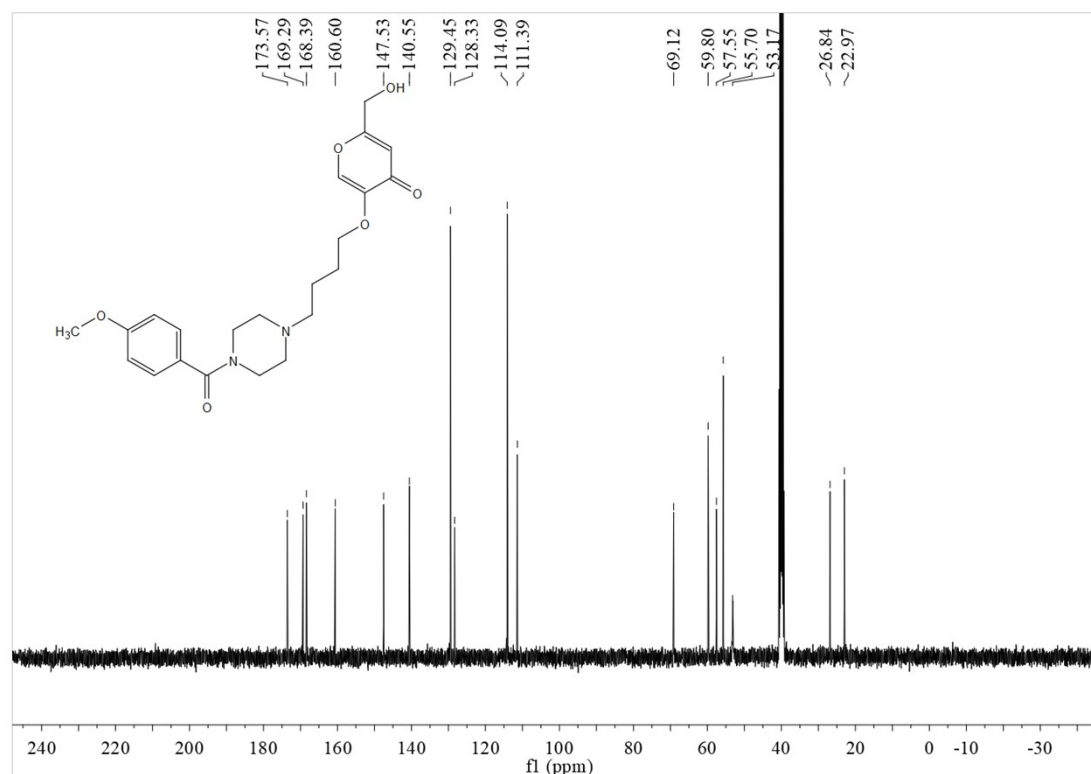
13 C NMR of 2-(hydroxymethyl)-5-(4-(4-(4-methoxybenzoyl)piperazin-1-yl)butoxy)-4H-pyran-4-one (3f)
