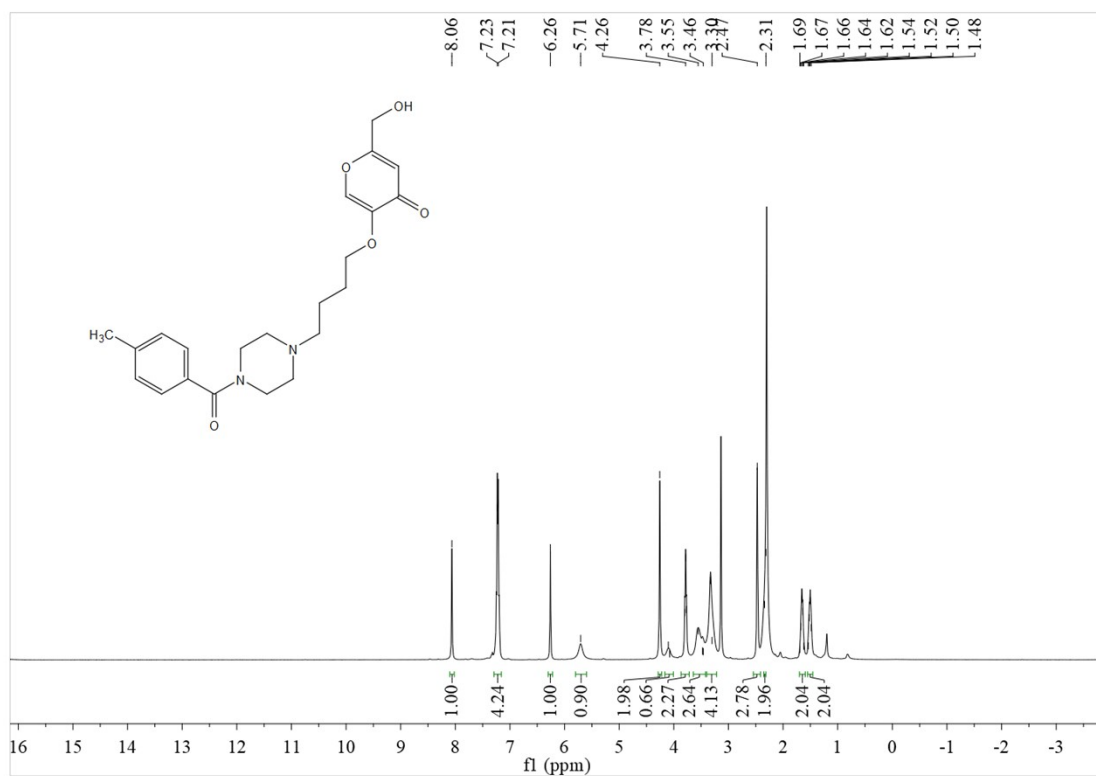
1 H NMR of 2-(hydroxymethyl)-5-(4-(4-(4-methylbenzoyl)piperazin-1-yl)butoxy)-4H-pyran-4-one (3c)
