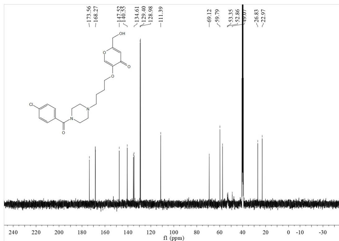
13 C NMR of 5-(4-(4-(4-chlorobenzoyl)piperazin-1-yl)butoxy)-2-(hydroxymethyl)-4H-pyran-4-one (31)
