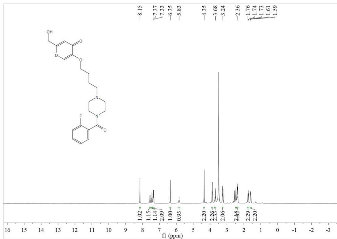
1 H NMR of 5-(4-(4-(2-fluorobenzoyl)piperazin-1-yl)butoxy)-2-(hydroxymethyl)-4H-pyran-4-one (3g)
