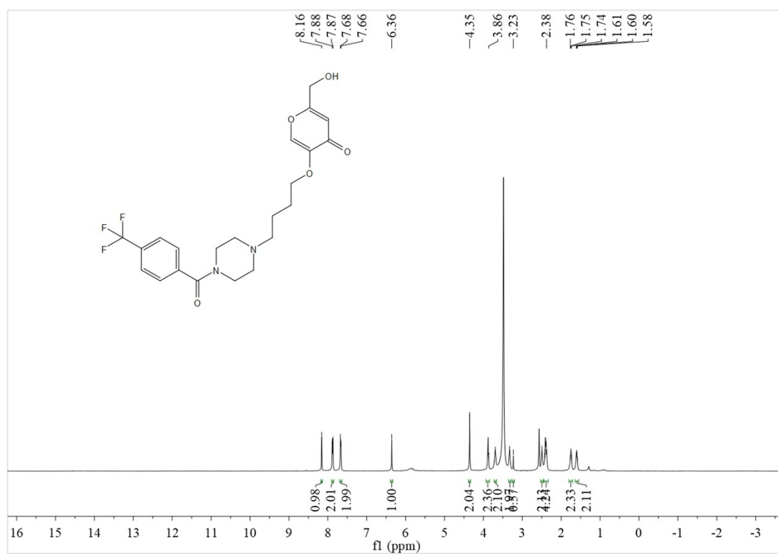
1 H NMR of 2-(hydroxymethyl)-5-(4-(4-(4-(trifluoromethyl)benzoyl)piperazin-1-yl)butoxy)-4H-pyran-4-one (3r)
