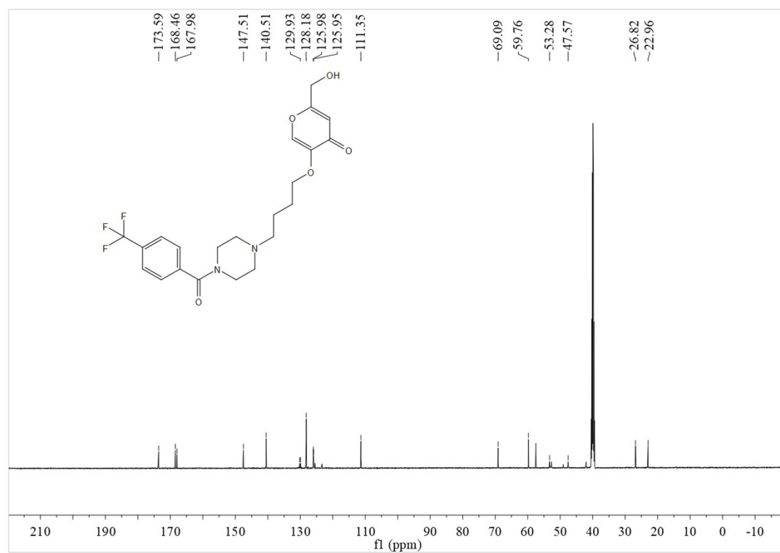
13 C NMR of 2-(hydroxymethyl)-5-(4-(4-(4-(trifluoromethyl)benzoyl)piperazin-1-yl)butoxy)-4H-pyran-4-one (3r)
