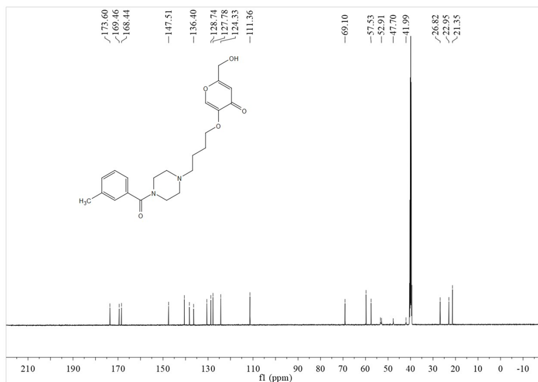
13 C NMR of 2-(hydroxymethyl)-5-(4-(4-(3-methylbenzoyl)piperazin-1-yl)butoxy)-4H-pyran-4-one (3b)
