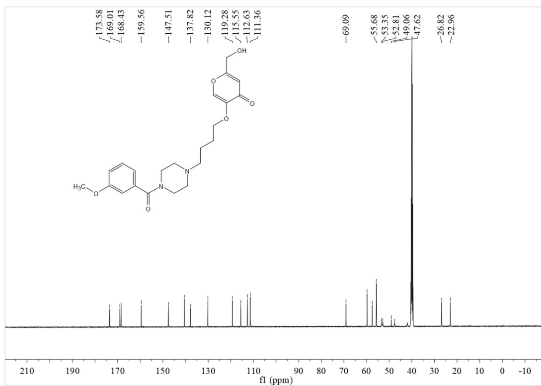
13 C NMR of 2-(hydroxymethyl)-5-(4-(4-(3-methoxybenzoyl)piperazin-1-yl)butoxy)-4H-pyran-4-one (3e)
