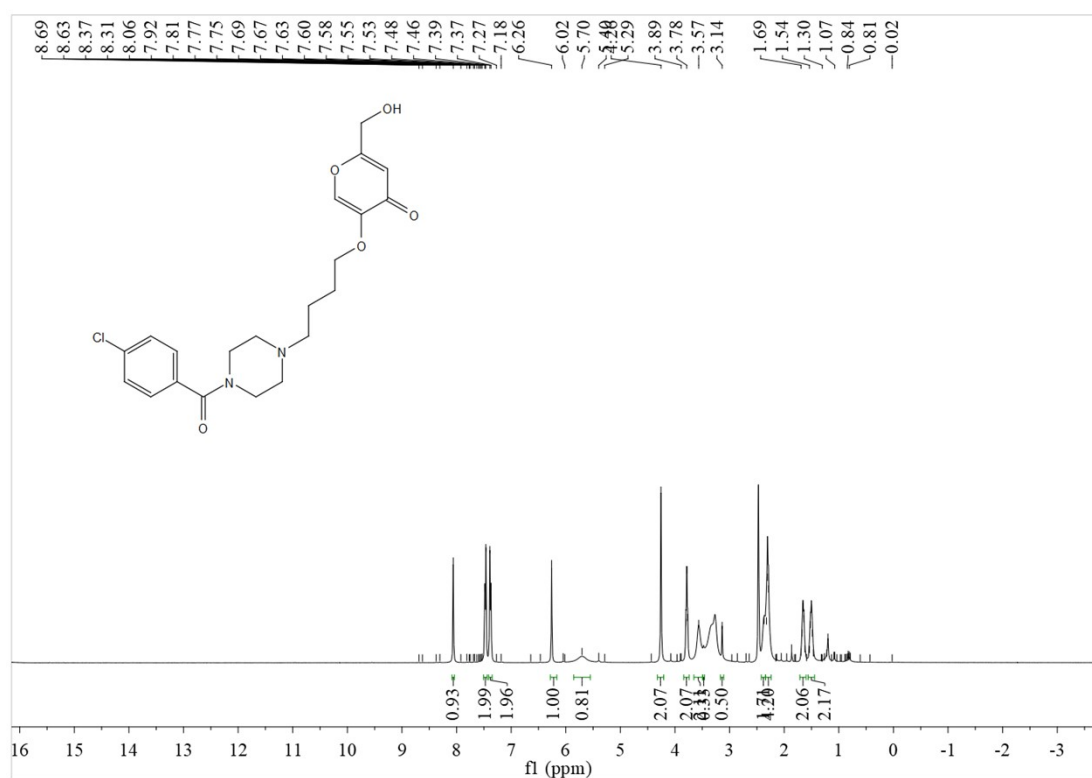
1 H NMR of 5-(4-(4-(4-chlorobenzoyl)piperazin-1-yl)butoxy)-2-(hydroxymethyl)-4H-pyran-4-one (31)
