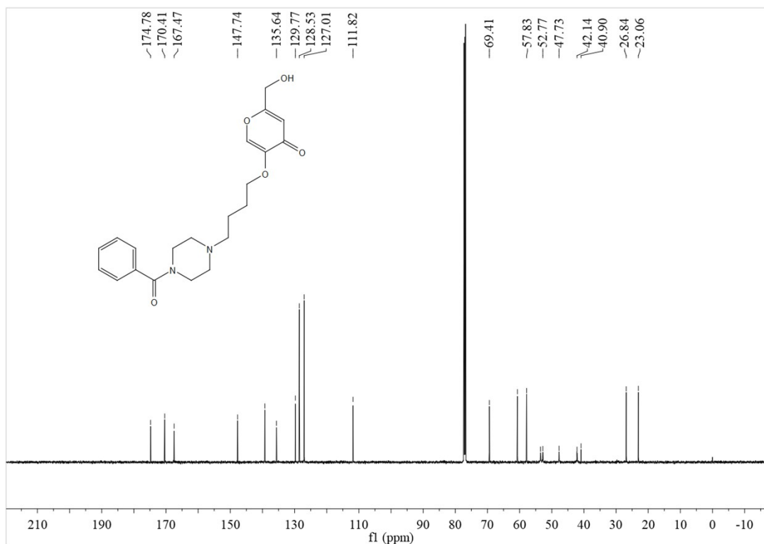
13 C NMR of 5-(4-(4-benzoylpiperazin-1-yl)butoxy)-2-(hydroxymethyl)-4H-pyran-4-one (3a)
