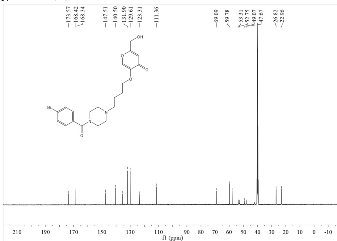
13 C NMR of 5-(4-(4-(4-bromobenzoyl)piperazin-1-yl)butoxy)-2-(hydroxymethyl)-4H-pyran-4-one (3o)
