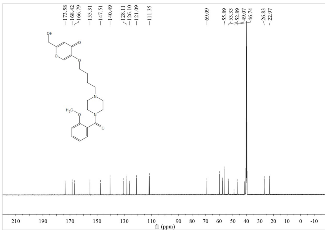
13 CNMR of 2-(hydroxymethyl)-5-(4-(4-(2-methoxybenzoyl)piperazin-1-yl)butoxy)-4H-pyran-4-one (3d)
