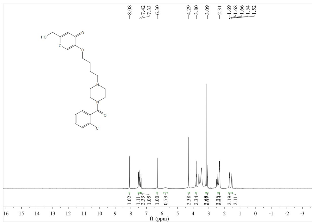
1 H NMR 5-(4-(4-(2-chlorobenzoyl)piperazin-1-yl)butoxy)-2-(hydroxymethyl)-4H-pyran-4-one (3j)
