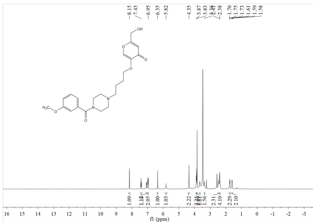
1 H NMR of 2-(hydroxymethyl)-5-(4-(4-(3-methoxybenzoyl)piperazin-1-yl)butoxy)-4H-pyran-4-one (3e)
