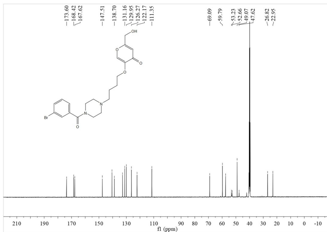
13 C NMR of 5-(4-(4-(3-bromobenzoyl)piperazin-1-yl)butoxy)-2-(hydroxymethyl)-4H-pyran-4-one (3n)
