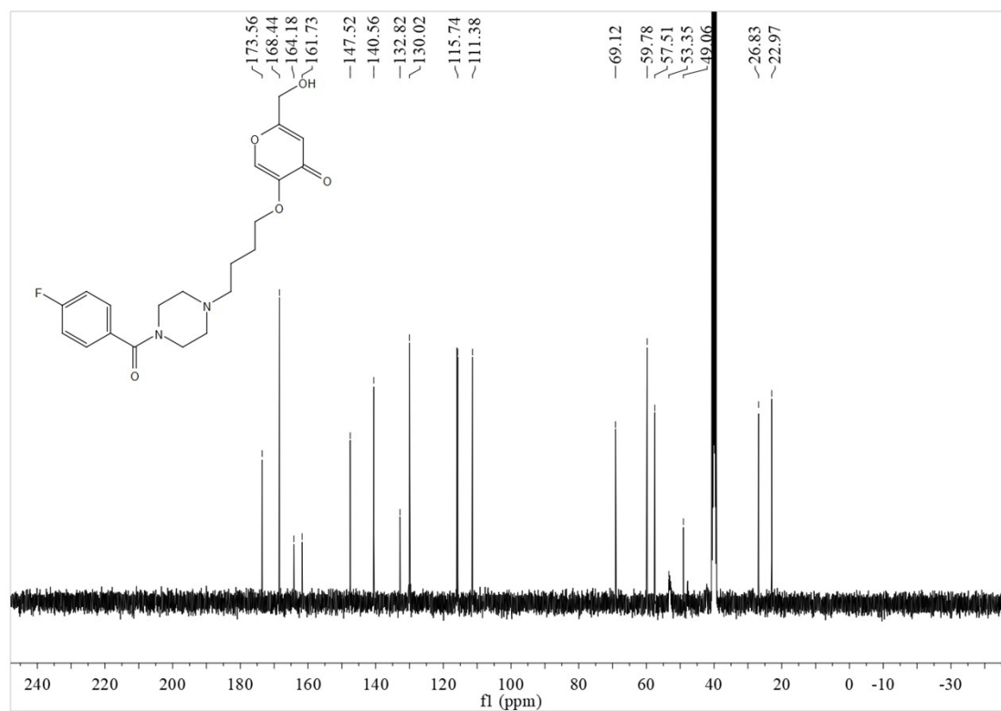
13 C NMR of 5-(4-(4-(4-fluorobenzoyl)piperazin-1-yl)butoxy)-2-(hydroxymethyl)-4H-pyran-4-one (3i)
