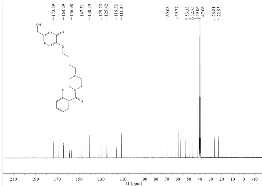
13 C NMR of 5-(4-(4-(2-fluorobenzoyl)piperazin-1-yl)butoxy)-2-(hydroxymethyl)-4H-pyran-4-one (3g)
