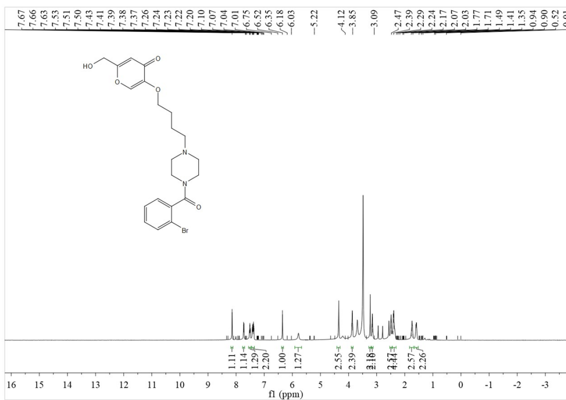
1 H NMR of 5-(4-(4-(2-bromobenzoyl)piperazin-1-yl)butoxy)-2-(hydroxymethyl)-4H-pyran-4-one (3m)
