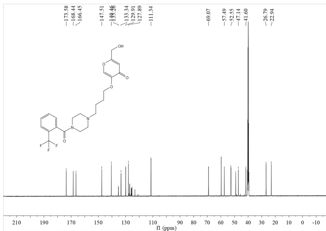
13 C NMR of 2-(hydroxymethyl)-5-(4-(4-(2-(trifluoromethyl)benzoyl)piperazin-1-yl)butoxy)-4H-pyran-4-one (3p)
