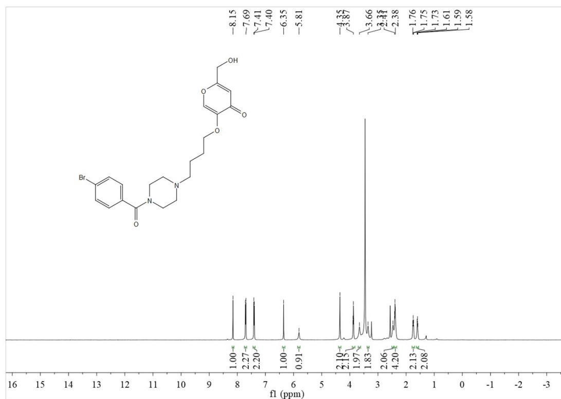
1 H NMR of 5-(4-(4-(4-bromobenzoyl)piperazin-1-yl)butoxy)-2-(hydroxymethyl)-4H-pyran-4-one (3o)
