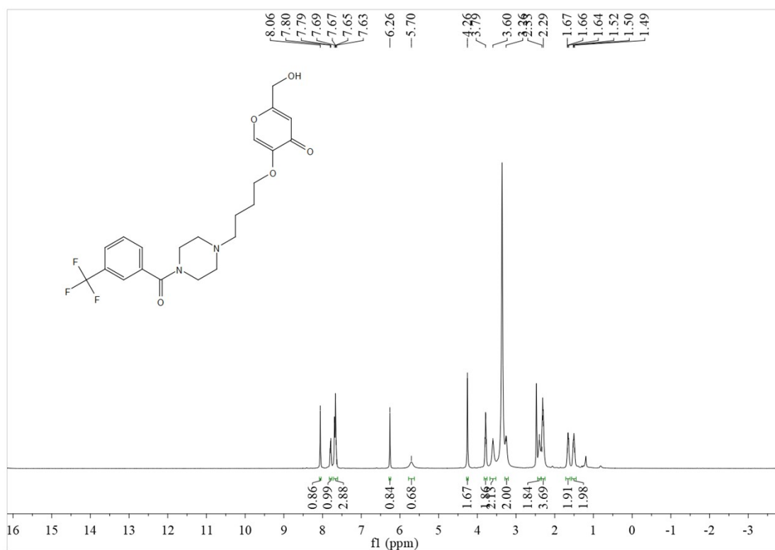
1 H NMR of 2-(hydroxymethyl)-5-(4-(4-(3-(trifluoromethyl)benzoyl)piperazin-1-yl)butoxy)-4H-pyran-4-one (3q)
