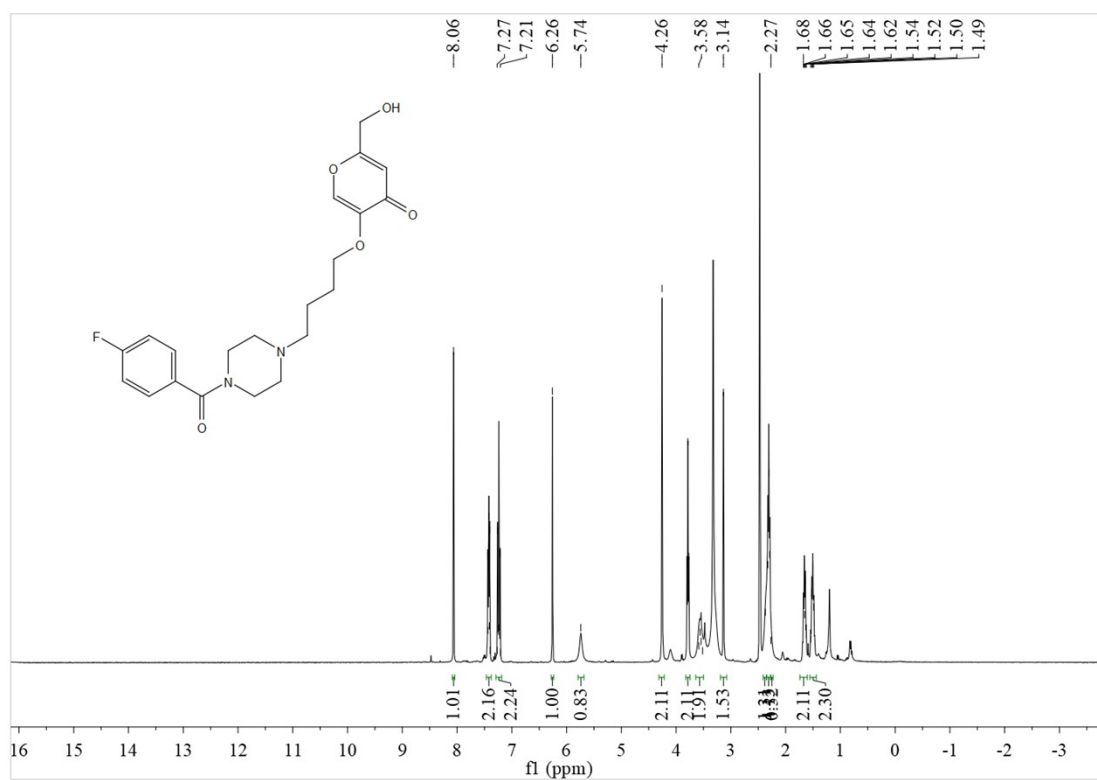
1 H NMR of 5-(4-(4-(4-fluorobenzoyl)piperazin-1-yl)butoxy)-2-(hydroxymethyl)-4H-pyran-4-one (3i)
