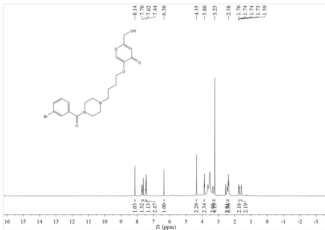
1 H NMR of 5-(4-(4-(3-bromobenzoyl)piperazin-1-yl)butoxy)-2-(hydroxymethyl)-4H-pyran-4-one (3n)
