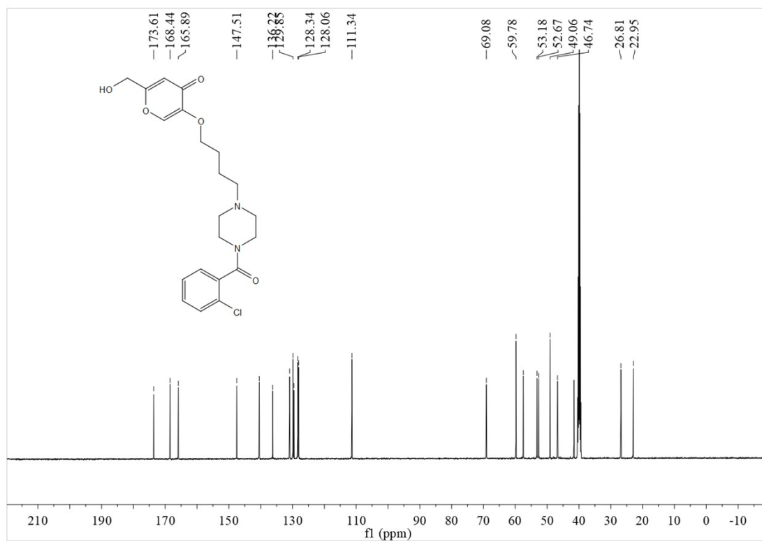
13 C NMR of 5-(4-(4-(2-chlorobenzoyl)piperazin-1-yl)butoxy)-2-(hydroxymethyl)-4H-pyran-4-one (3j)
