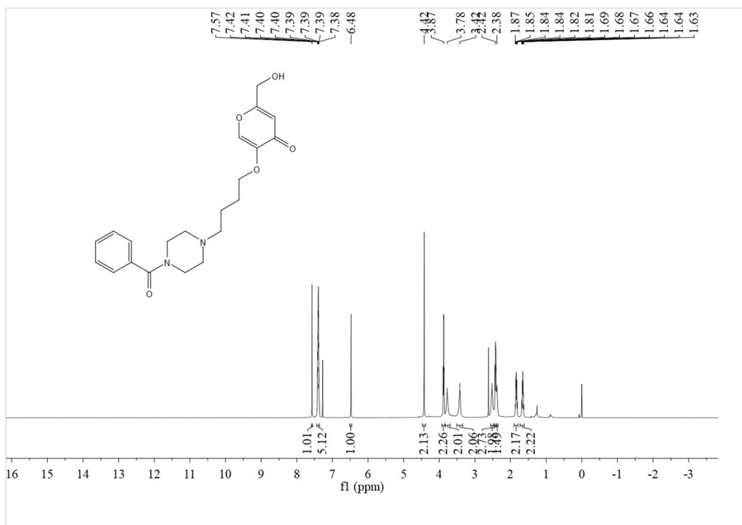
1 H NMR of 5-(4-(4-benzoylpiperazin-1-yl)butoxy)-2-(hydroxymethyl)-4H-pyran-4-one (3a)
