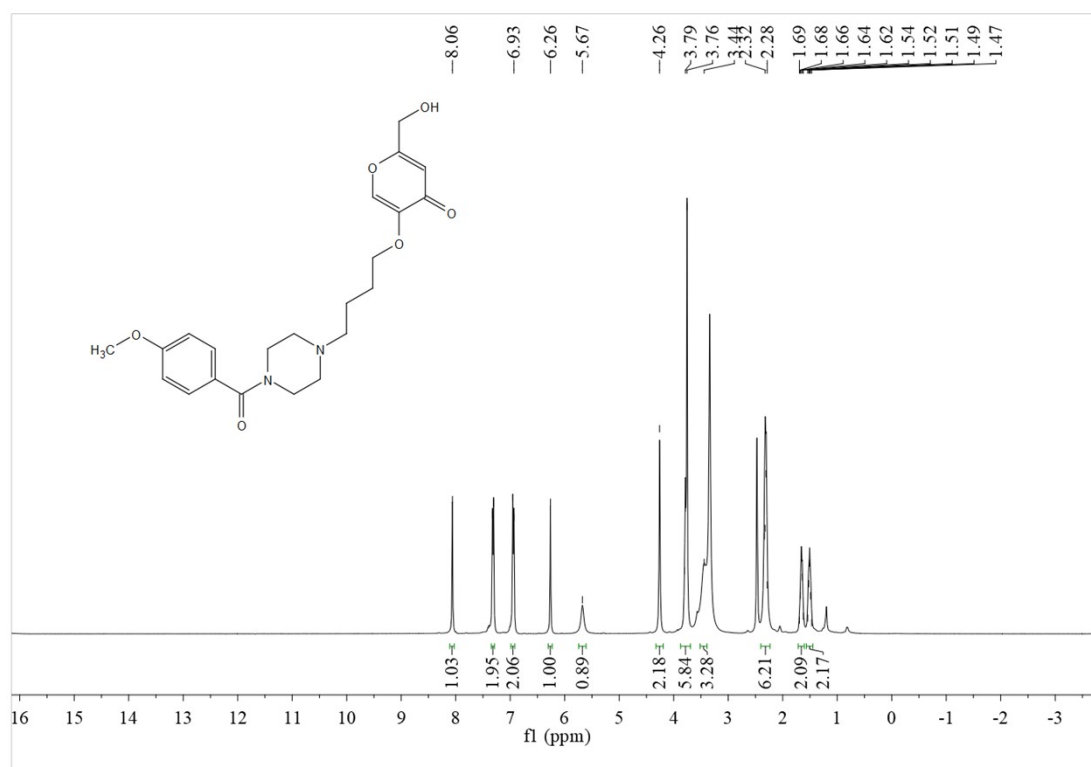
1 H NMR of 2-(hydroxymethyl)-5-(4-(4-(4-methoxybenzoyl)piperazin-1-yl)butoxy)-4H-pyran-4-one (3f)
