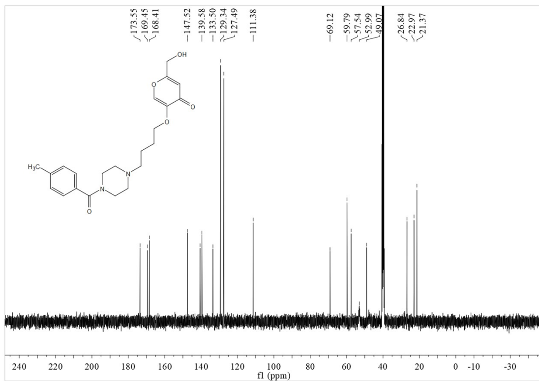
13 C NMR of 2-(hydroxymethyl)-5-(4-(4-(4-methylbenzoyl)piperazin-1-yl)butoxy)-4H-pyran-4-one (3c)
