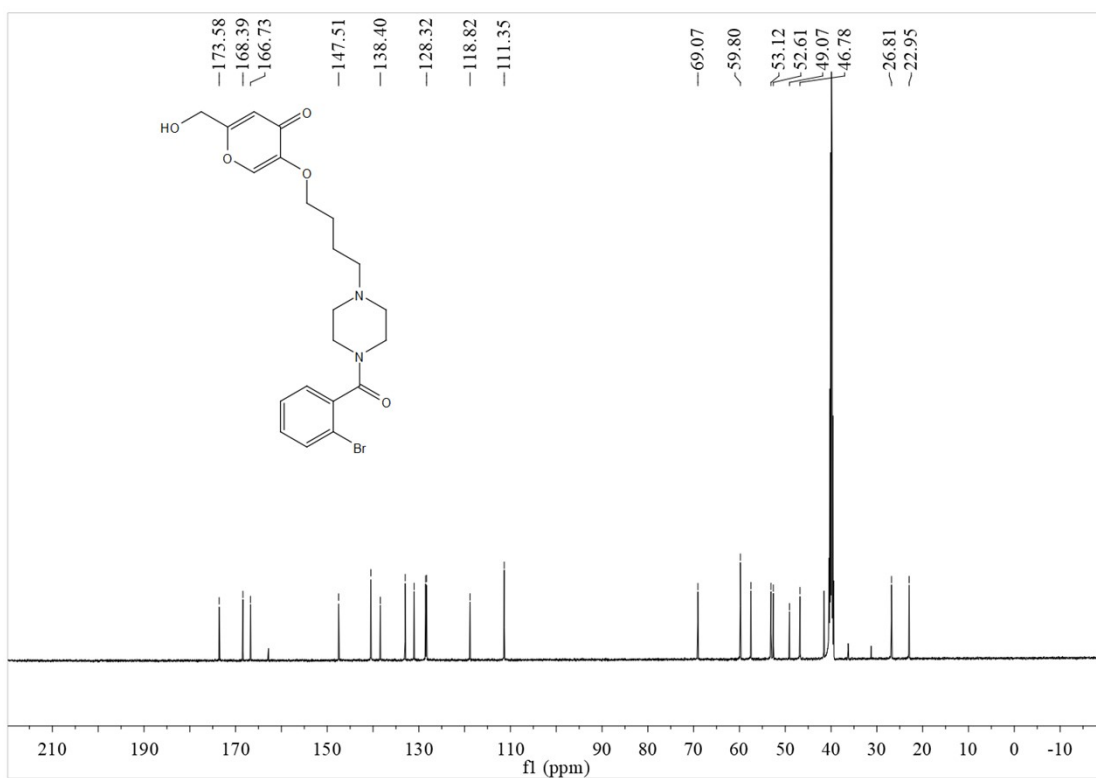
13 C NMR of 5-(4-(4-(2-bromobenzoyl)piperazin-1-yl)butoxy)-2-(hydroxymethyl)-4H-pyran-4-one (3m)
