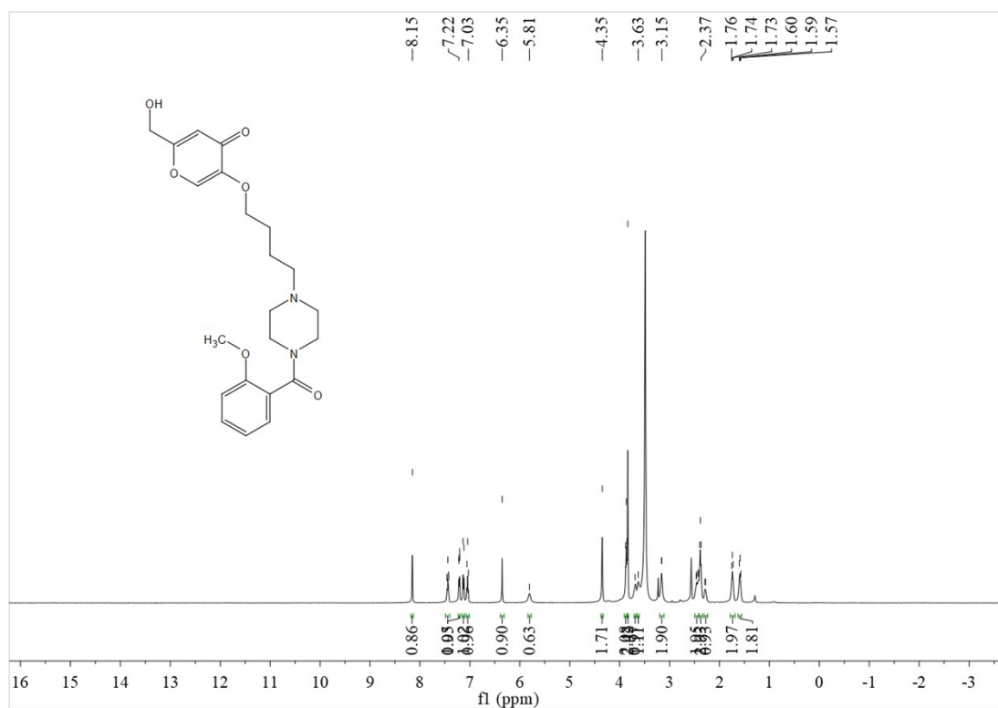
1 H NMR of 2-(hydroxymethyl)-5-(4-(4-(2-methoxybenzoyl)piperazin-1-yl)butoxy)-4H-pyran-4-one (3d)
