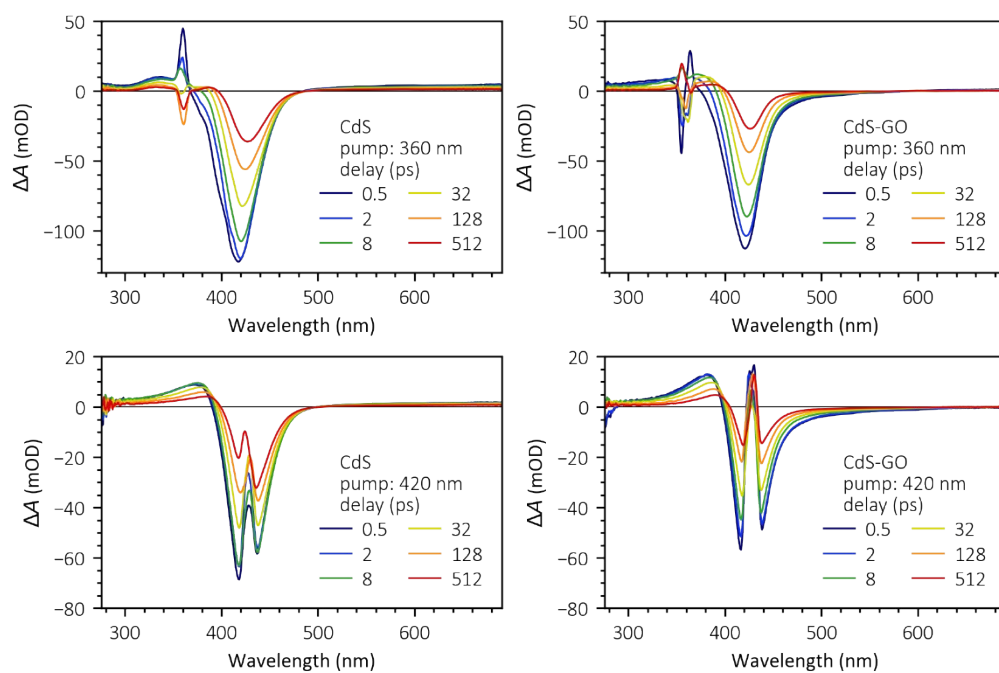
Figure S1: Comparison of TA data: excitation wavelengths (top row) 360 nm and (bottom row) 420 nm, for samples (left) CdS (right) CdS GO.
