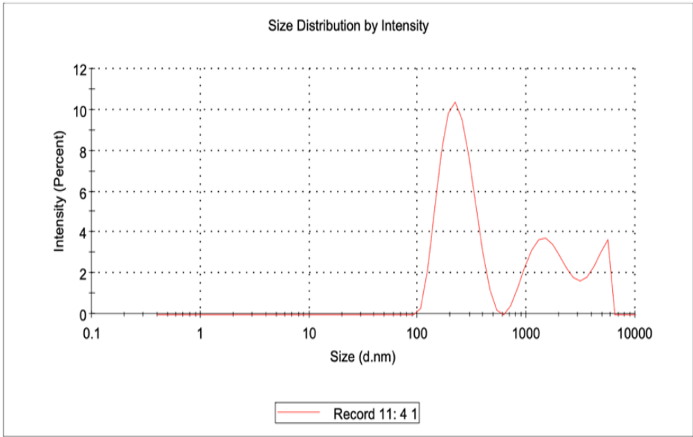
Fig. S4 Zeta size to of composite coded AA4.
