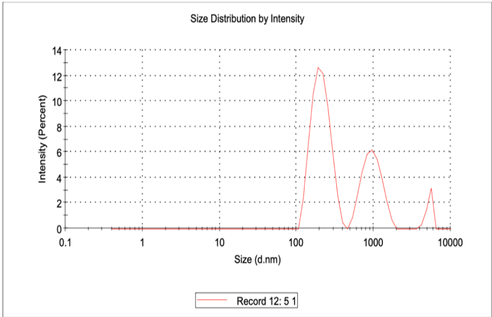
Fig. S5 Zeta size to of composite coded AA5.
