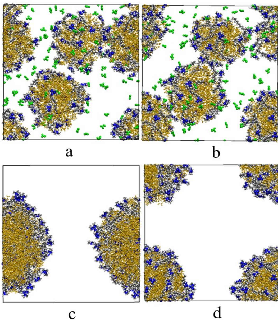
Figure S1. Final configurations of the DTMGH and DTMG systems in the emulsion model, where a, b are the front view and top view of the DTMGH system, respectively, and c, d are the front view and top view of the DTMG system, respectively. Yellow represents the oil phase, green represents the carbonate ion, and the carbon, nitrogen, and hydrogen atoms in the surfactant are grey, blue, and white, respectively. Water molecules are hidden.
