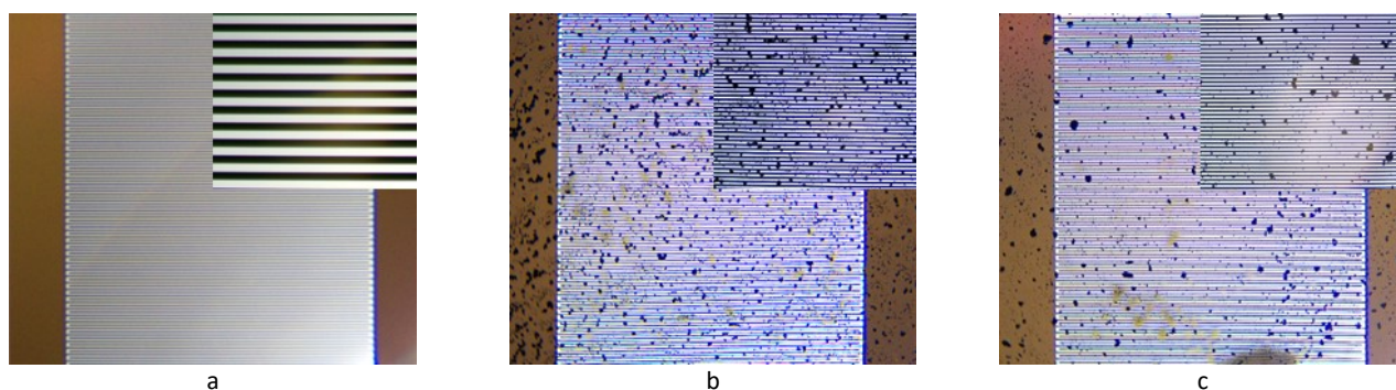
Figure S1. Optical micrographs of the samples before and after deposition of the sensing layer: (a) pristine IDE; (b) IDE coated with PANi; (c) IDE coated with PANi/GO.
