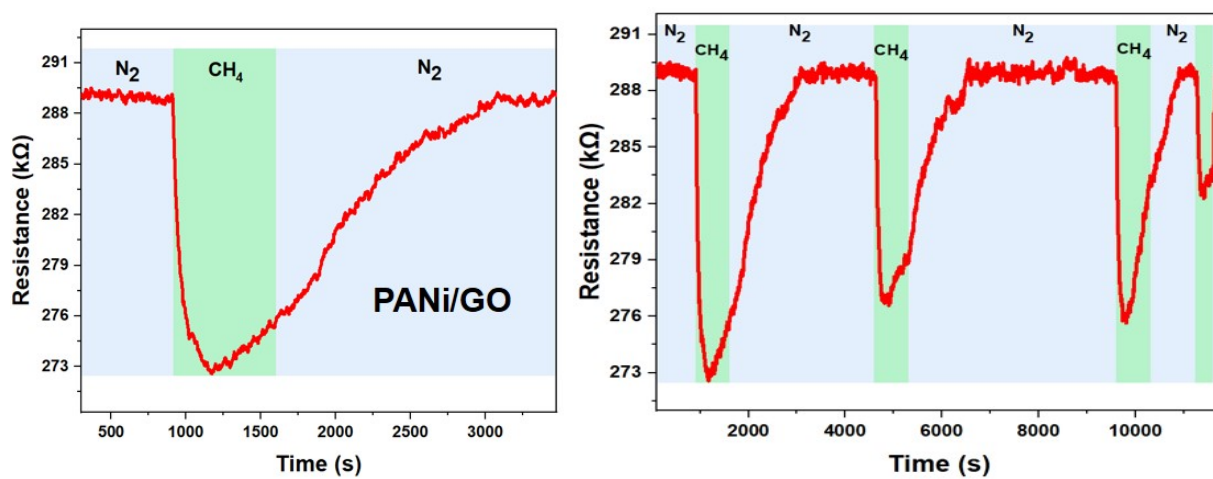
Figure S2. Gas-sensing performance of the PANi/GO composite toward CH 4 at room temperature
