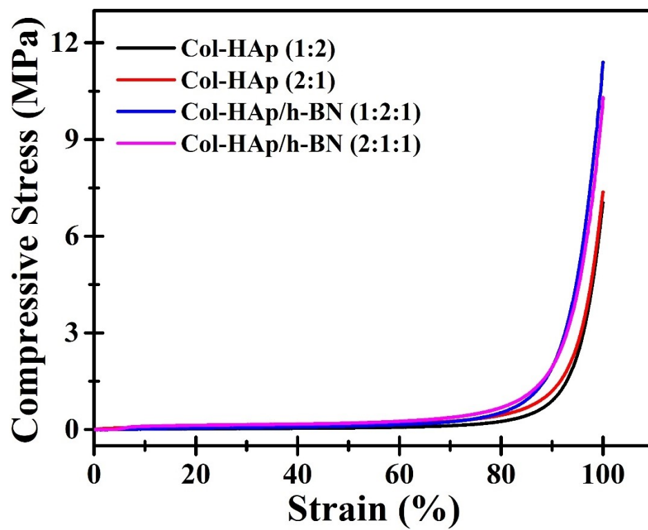
Figure S2: Compressive stress vs strain curve of different fabricated scaffold
