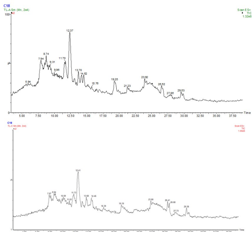
Fig.3. Chromatograms before and after the addition of nano-Fe 2 O 3
