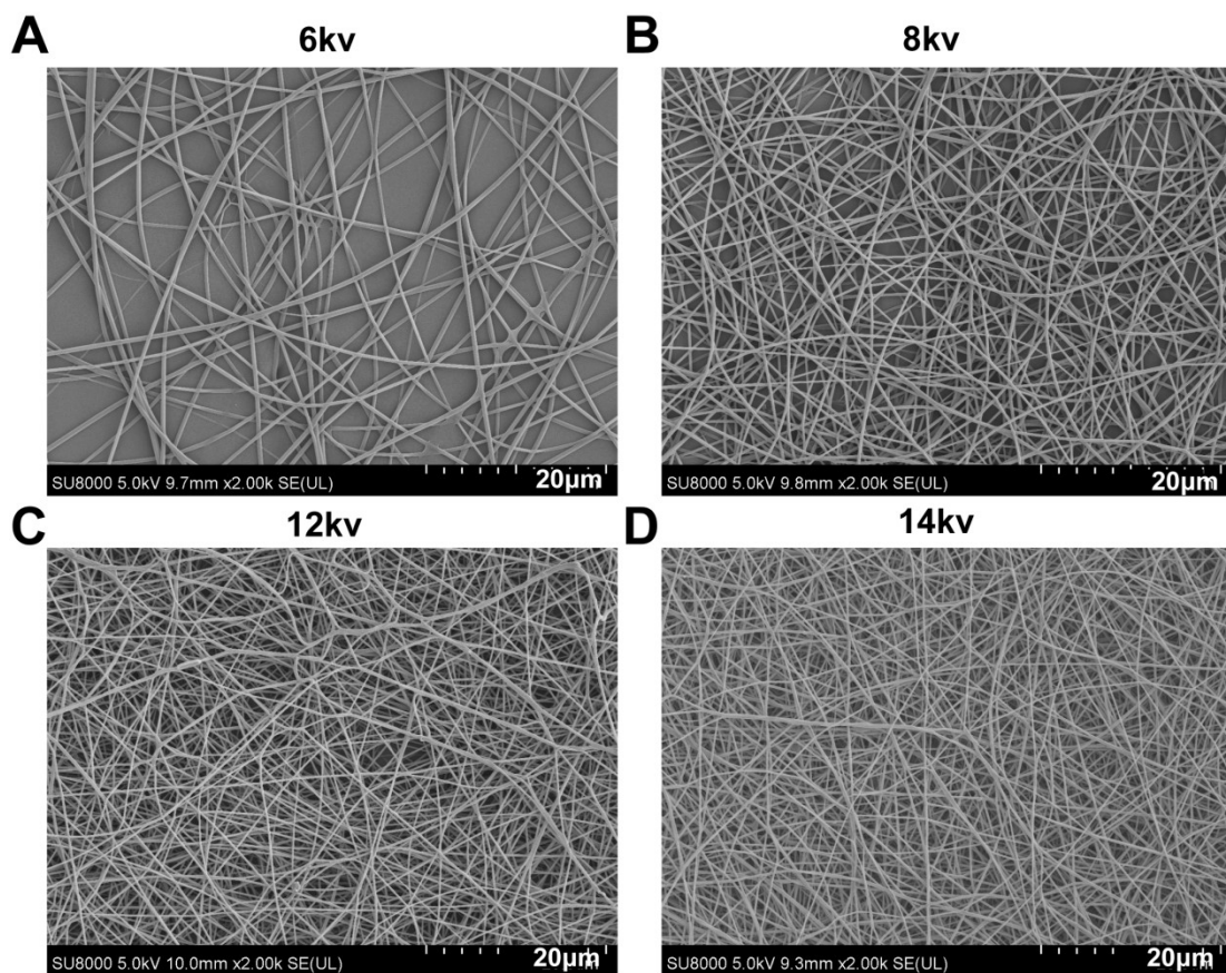
Fig. S1 SEM observation of the effect of spinning voltage on fiber formation at (A) 6 kV (B) 8 kV, (C) 12 kV, and (D) 14 kV.
