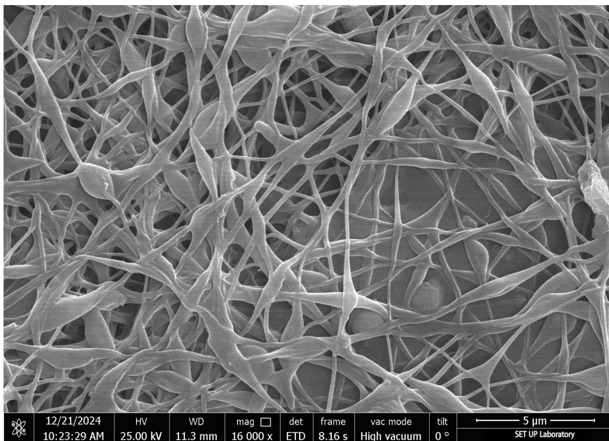
Figure S1. The FE-SEM image of PVA.
