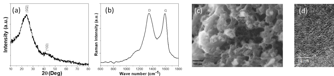
Fig. S1: (a) Powder XRD, (b) Raman spectrum, (c) SEM image and (d) TEM of carbon derived from custard apple seed.
