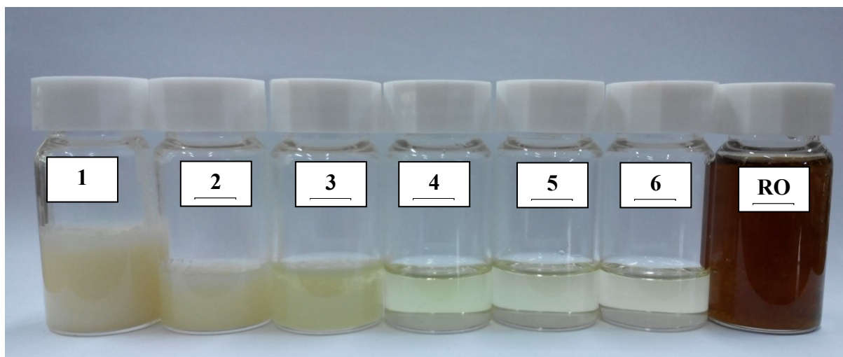
S2. The appearance of the product collected from reactor. Number 1 until 6 are products collected from reactor at 30, 60, 90, 120, 150, and 180 minutes of reaction, respectively. RO is the remaining oil that collected from the bottom of the reactor after the reaction finished.
