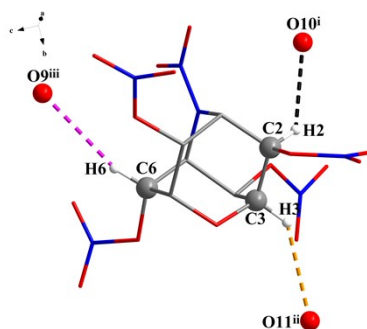
Fig.S5 Hydrogen bond diagram of compound 4
