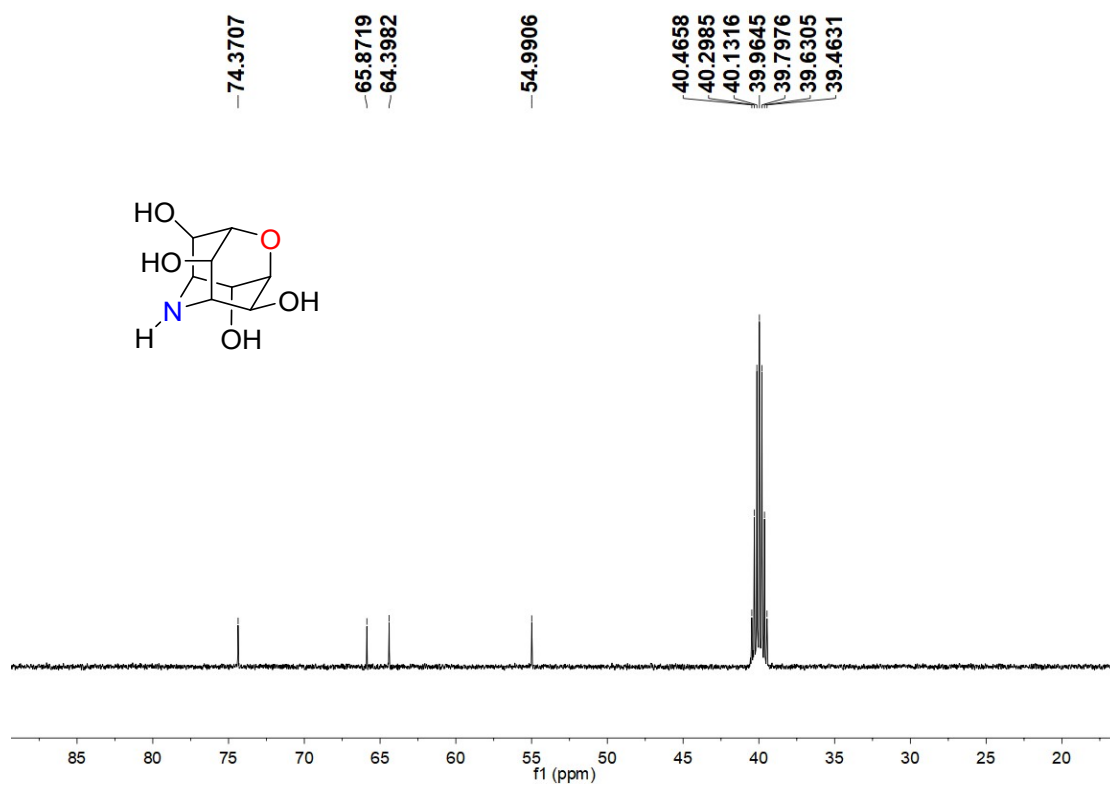
Fig.S15 ^{13}\text{C} NMR spectrum of compound 11 (DMSO- d_6 , 126 MHz)
