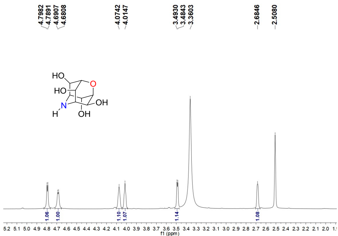
Fig.S14 ^1\text{H} NMR spectrum of compound 3 ^ (DMSO- d_6 , 500 MHz)
