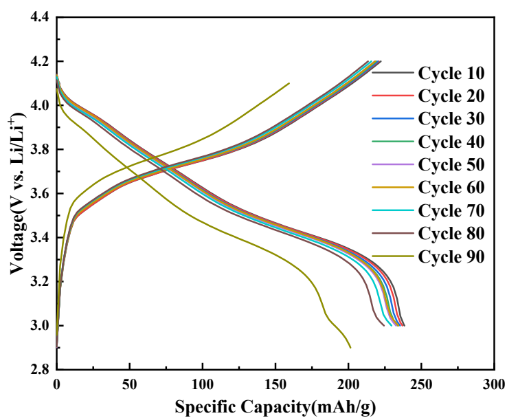
Fig.S1 Specific capacity–voltage profiles for the SSSLBs aged under CCCV–CCCV strategy at Cycle 10 to Cycle 90
