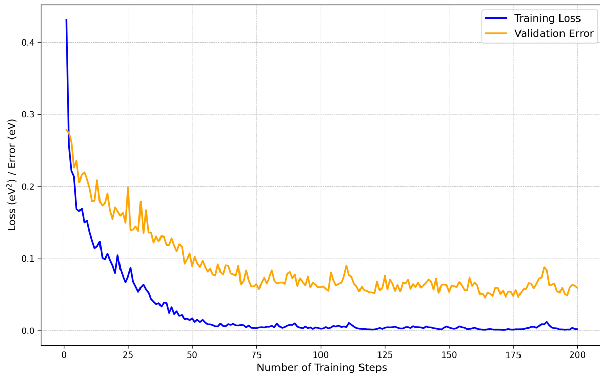
Figure S1: Training and validation loss curves for the MGT model over the training epochs. This plot demonstrates model convergence and the absence of significant overfitting.
