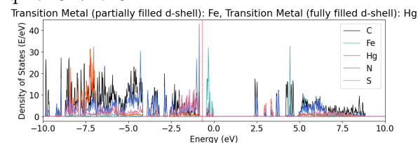
Figure S8: pDOS plots for all structure containing multiple metals in their metal centres
