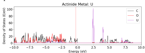
Figure S7: pDOS plots for all structure containing an Actinide metal
