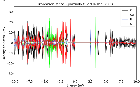
qmof-ea963b6:
