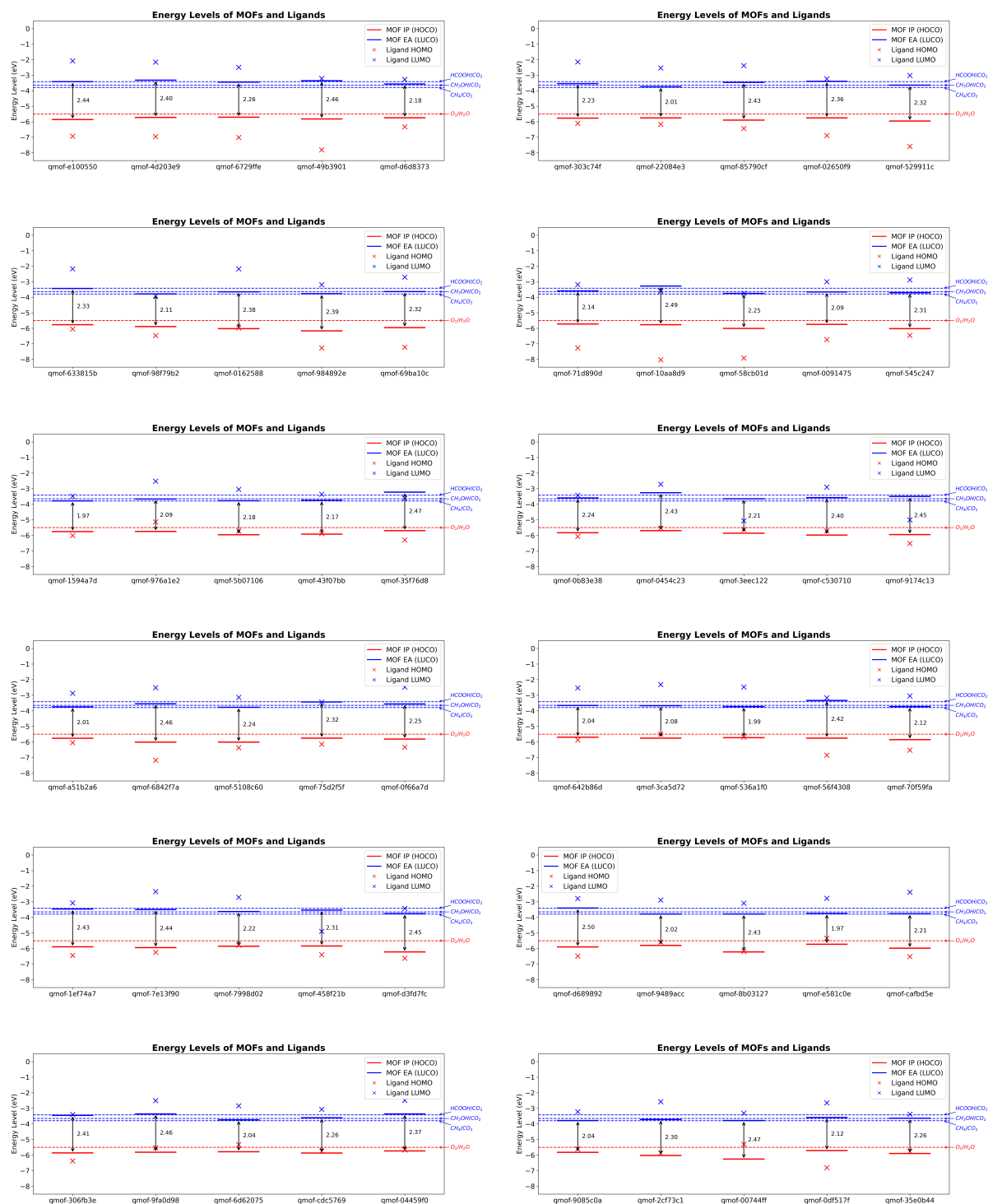
Figure S9: Energy diagrams comparing the Highest Occupied Crystal Orbital (HOCO) and Lowest Unoccupied Crystal Orbital (LUCO) of each MOF with the Highest Occupied Molecular Orbital (HOMO) and Lowest Unoccupied Molecular Orbital (LUMO) defined by the ligands of the MOF. For MOFs with multiple ligand types the HOMO and LUMO are taken as the highest HOMO and lowest LUMO between all of the ligands
