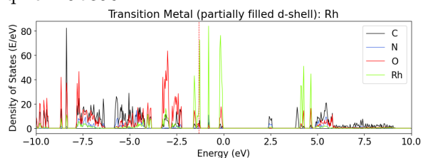
qmof-49b3901:
