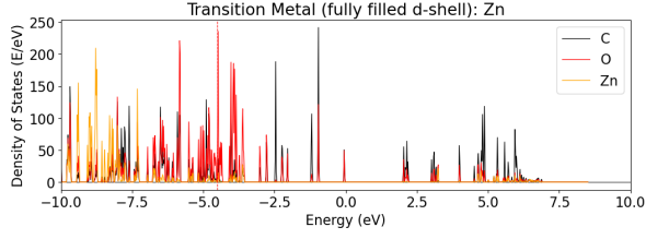
qmof-c4714cc:
