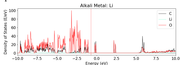
Figure S2: pDOS plots for all structure containing an Alkali metal
