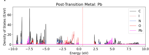
Figure S5: pDOS plots for all structure containing a Post-Transition metal
