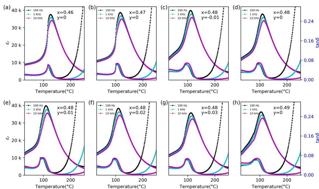
Figure S1: The temperature dependence of \epsilon_r and \tan\delta of PNN-PMcN-PT ceramics at 0.1-10 kHz with x=0.46-0.49 and y=-0.01-0.03
