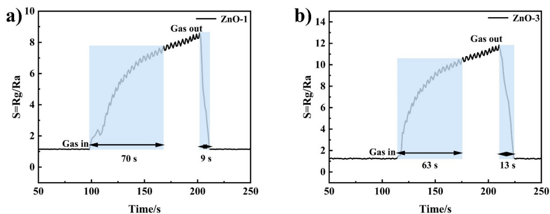
Fig. S1 (a) Instantaneous response-recovery curve of ZnO-1;(b) Instantaneous response-recovery curve of ZnO-3.
