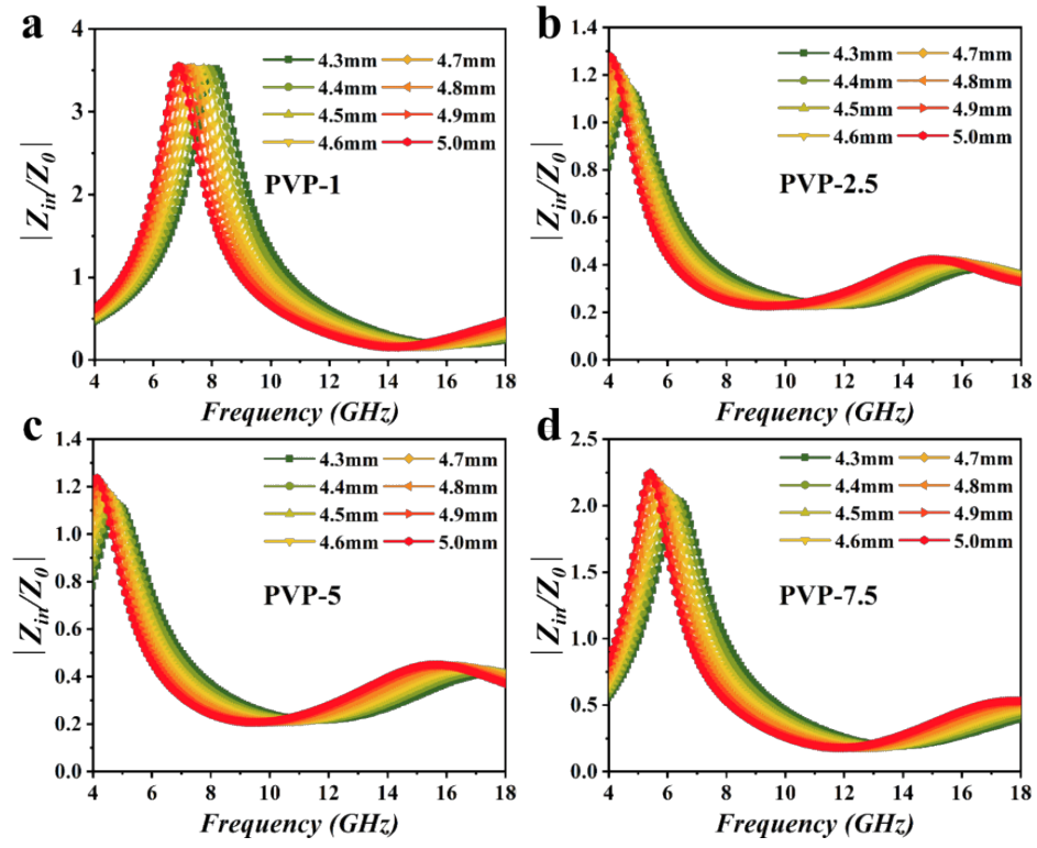
Fig. S3. Impedance matching for the products.
