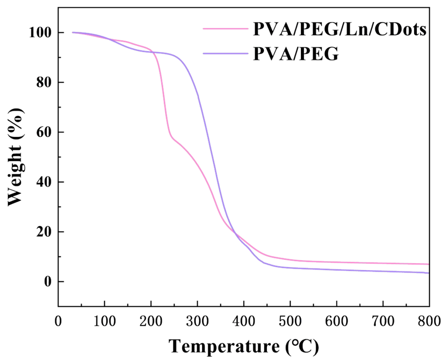
Fig. S2 Thermogravimetric analysis of PVA/PEG/Ln/CDots and PVA/PEG hydrogel
