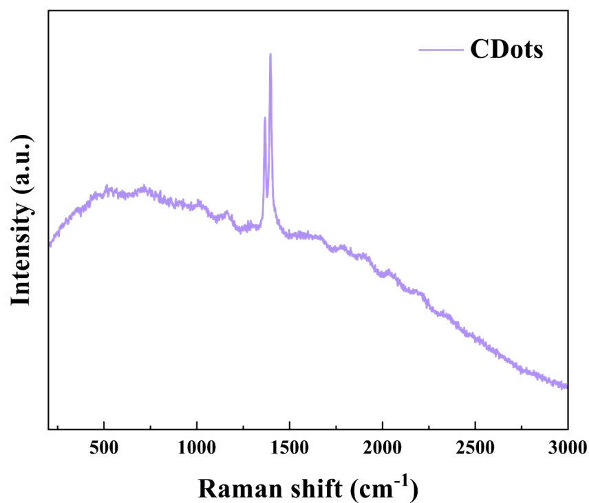
Fig. S1 Raman spectrum of CDots (excitation wavelength is 633nm)
