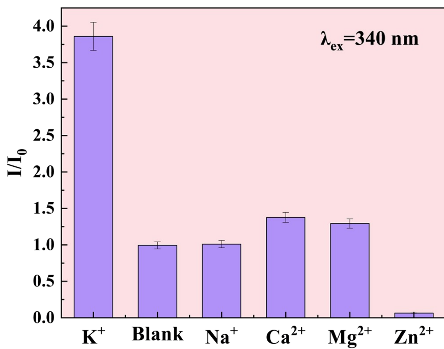
Fig. S3 Selectivity of PVA/PEG/Ln/CDots composite hydrogel for detection of various ions
