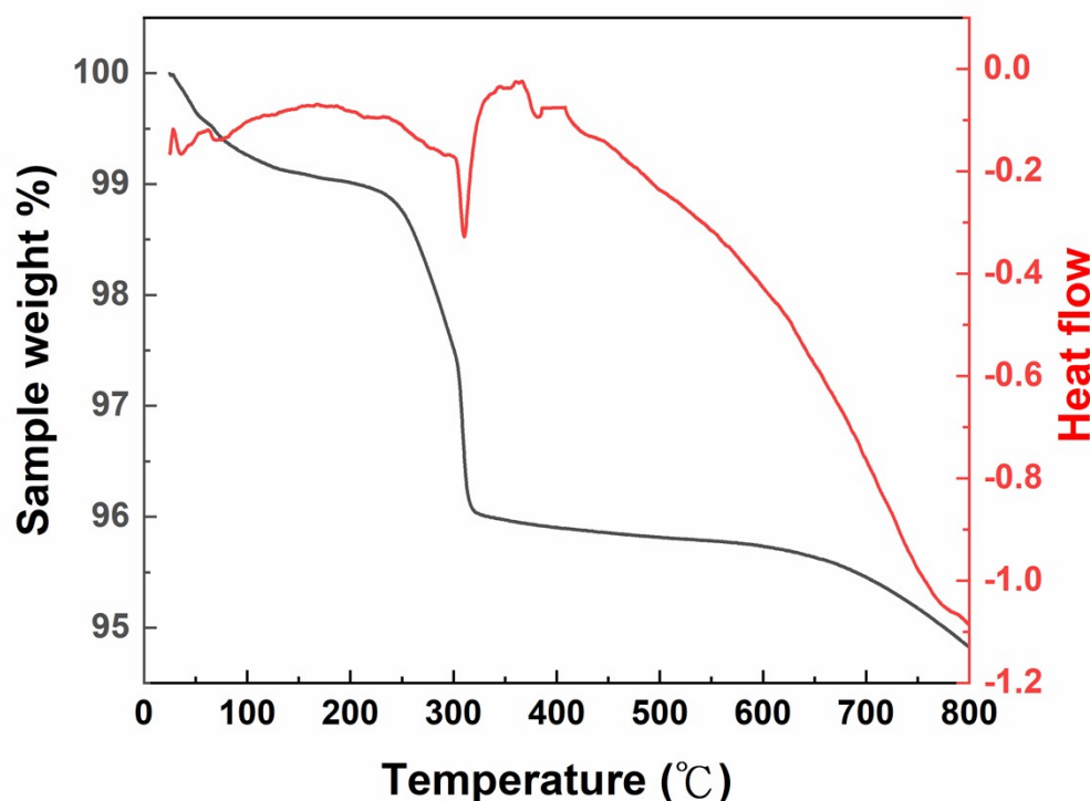
Figure S1. TGA/DSC profile recorded from TGS DES sample shows an endothermic peak at 300-320°C, corresponding to decomposition of ChCl and carbide formation.
