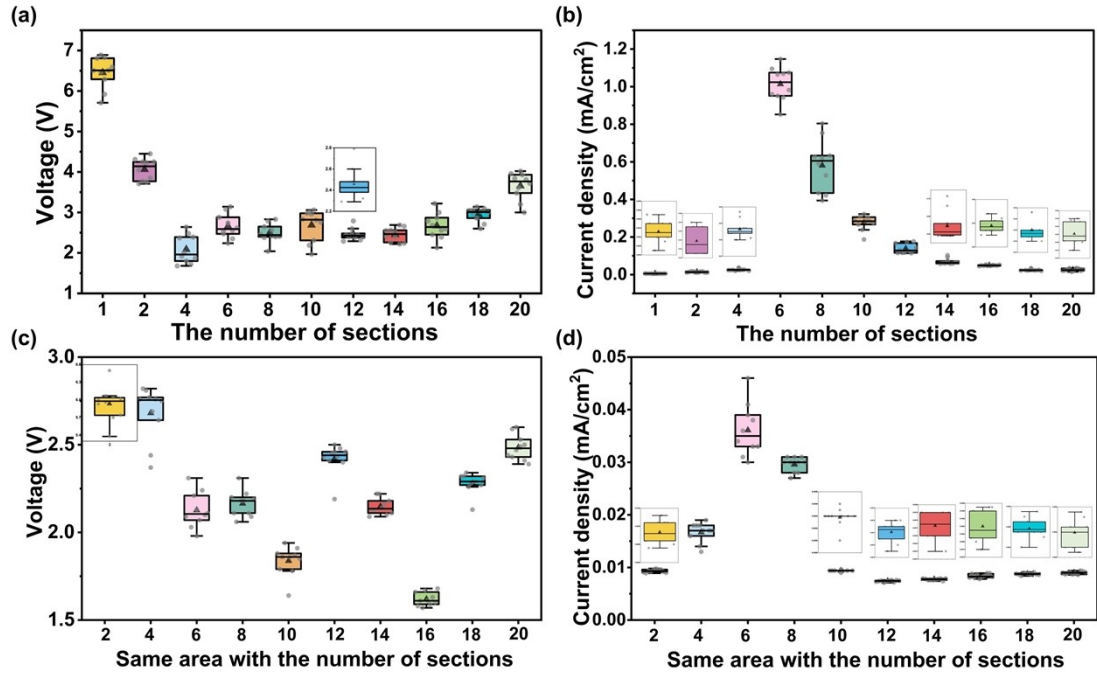
Fig. S2 (a) Boxing plot of the open circuit voltage of the devices with different sections; (b) boxing plot of the current density of the devices with different sections; (c) the boxing plot of the open circuit voltage for single circuit with the same areas as the different sections; (d) the boxing plot of the current density for single circuit with the same areas as the different sections.
