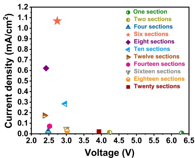
Fig. S1 The photovoltaic performance of the devices with different sections.
