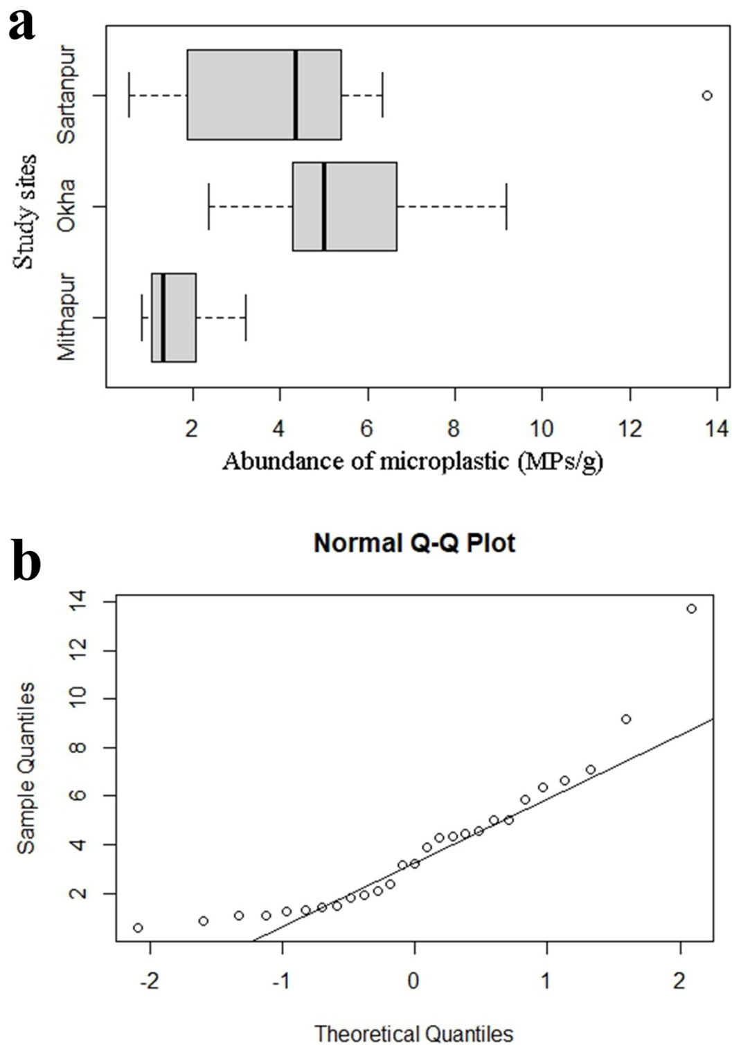
Fig. 1S: Abundance of microplastic contamination in the ginger prawn Metapenaeus kutchensis collected from three sampling locations of Gujarat coast, India, showing not a normal distribution (Shapiro-Wilk test, W = 0.86 , p < 0.05 ).
