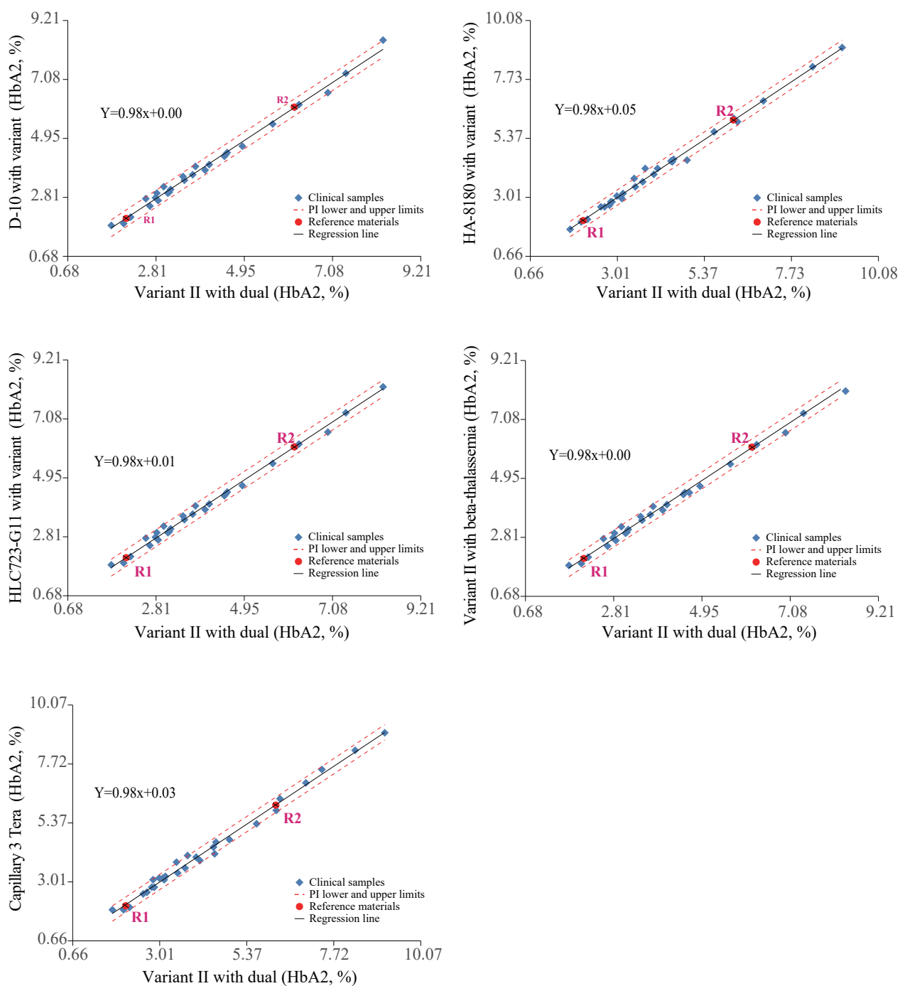
Fig. S5. The commutability of HbA2 reference materials was evaluated between certified value method and routine analyzers via Ordinary least squares regression when the uncertainty was taken into account. (A) Bio-Rad, D10, (B) ARKRAY, HA-8180, (C) TOSOH, HLC723-G11, (D) Bio-Rad, Variant II with beta-thalassemia, (E) Sebia, Capillary 3 Tera.
