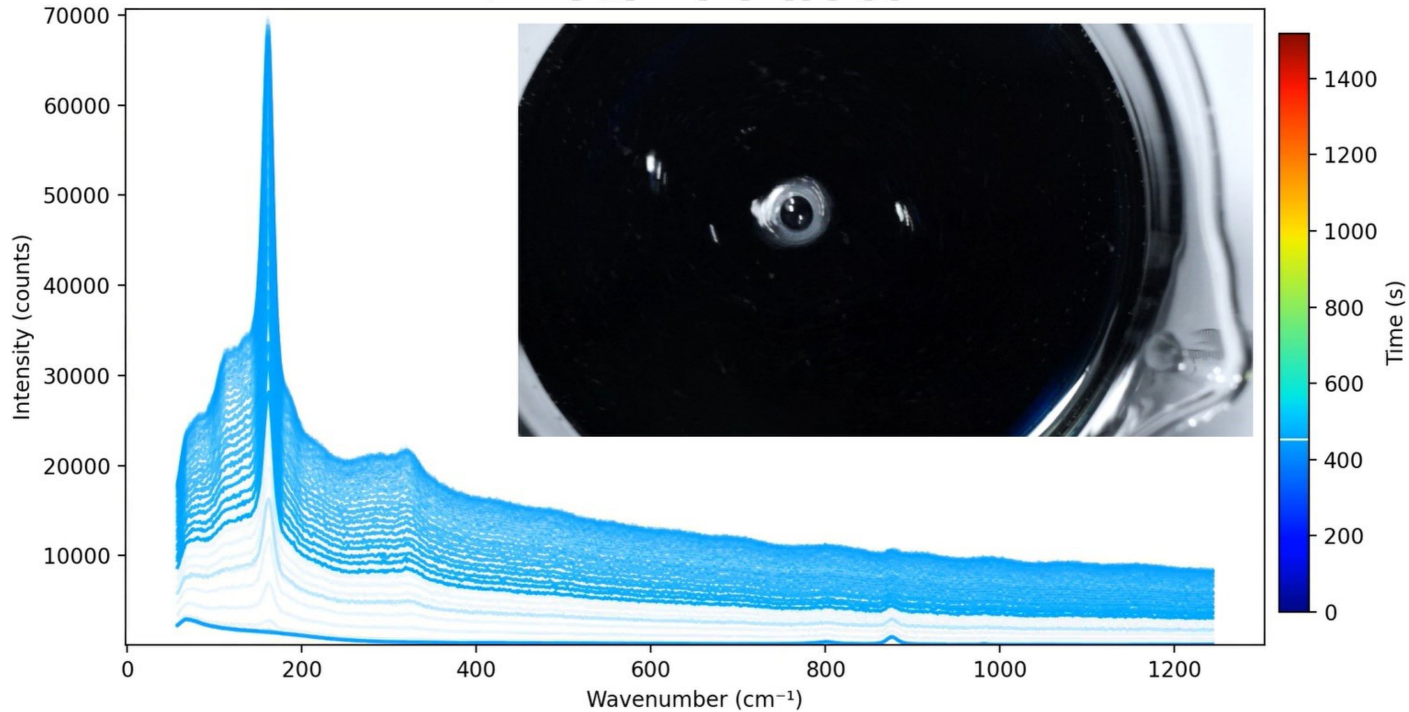
Spectral Plot_briggs_rauscher_run2_700c_0_5e_86p_1a_0i
