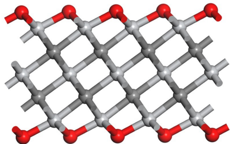
\text{Ti}_3\text{C}_2\text{O}_2
