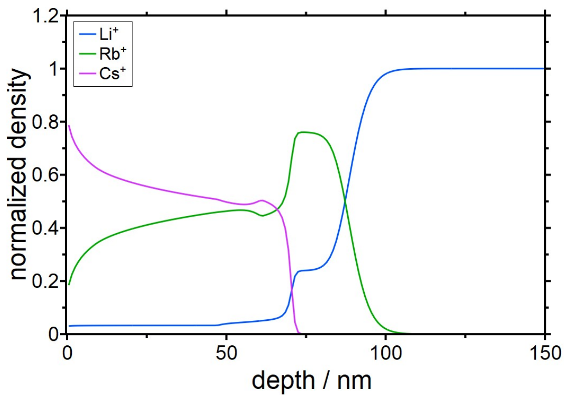
Figure S4 Snap shot of the time evolution leading to Figure 5 (main text) at 220h.
