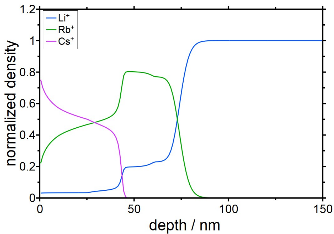
Figure S3 Snap shot of the time evolution leading to Figure 5 (main text) at 160h.
