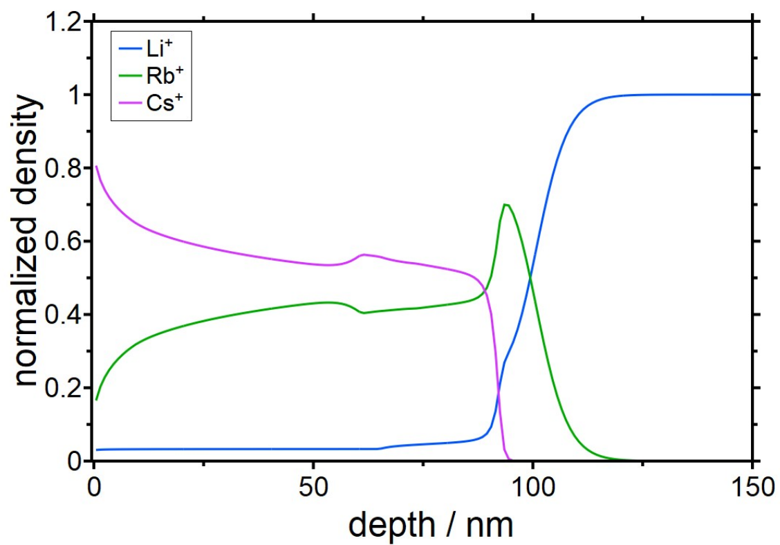
Figure S5 Snap shot of the time evolution leading to Figure 5 (main text) at 280h.
