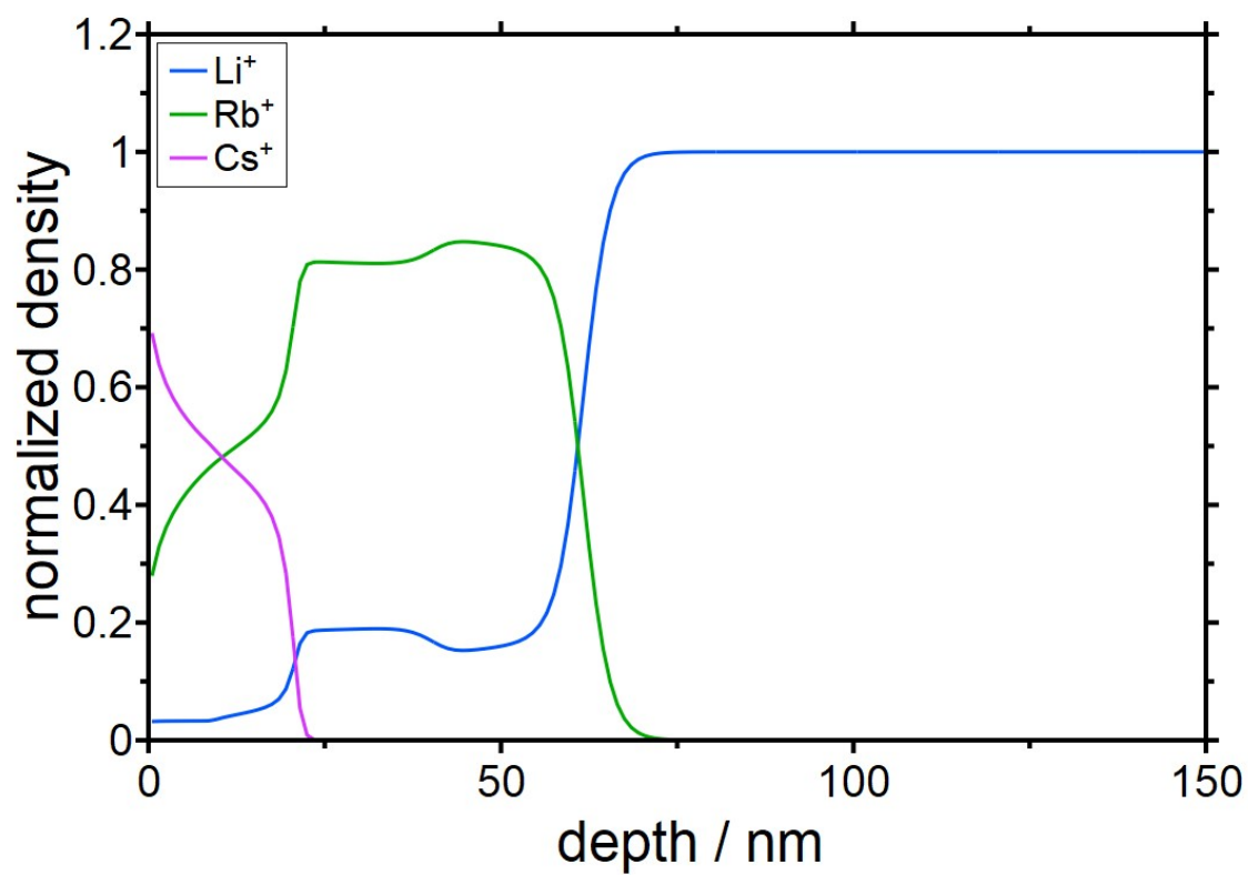
Figure S2 Snap shot of the time evolution leading to Figure 5 (main text) at 120h.
