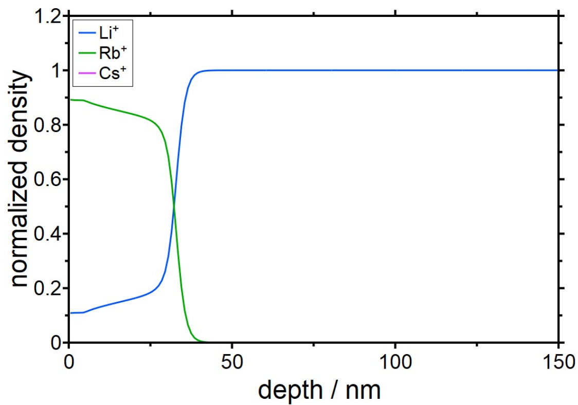
Figure S1 Snap shot of the time evolution leading to Figure 5 (main text) at 60h.
