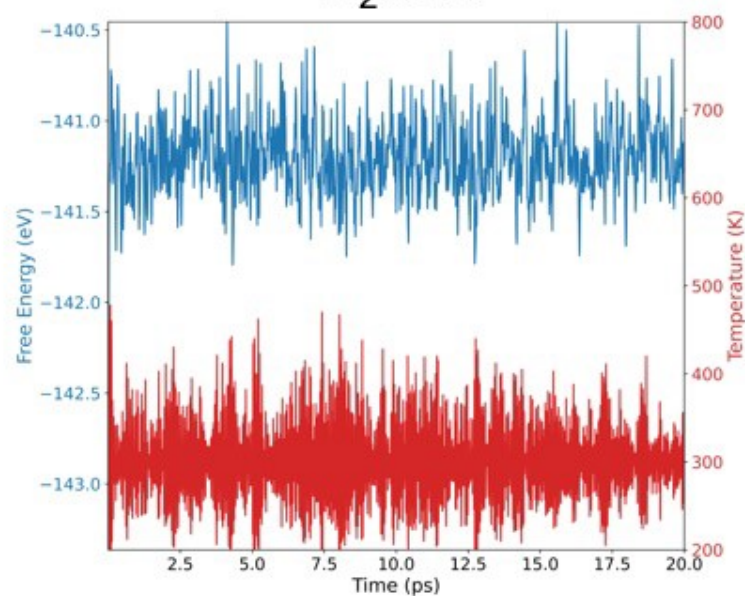
\text{Al}_2\text{TeSe}
