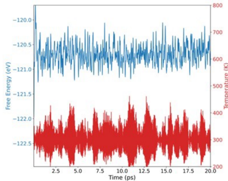
\text{InGaTeSe}
