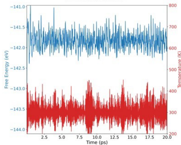
\text{AlGaSe}_2
