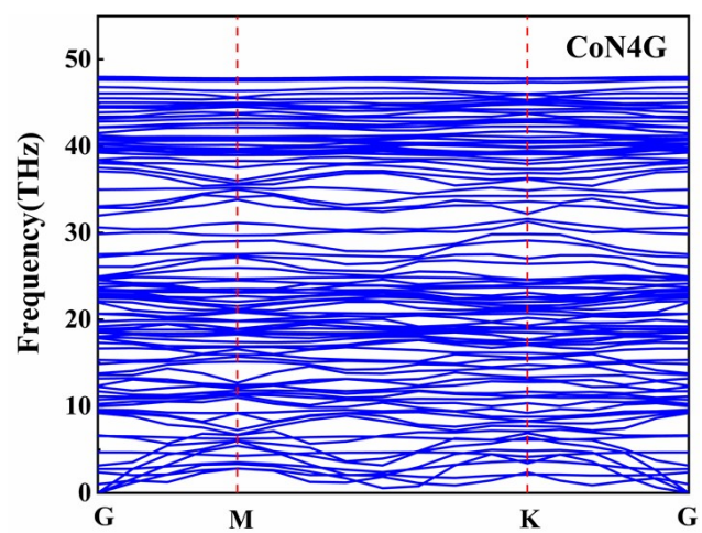
Figure S5. Phonon spectrum of \text{CoN}_4\text{G}
