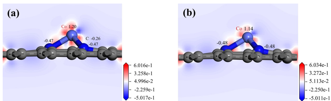
Figure S6. Charge difference density and Mulliken diagrams; (a) \text{CoN}_2\text{G} , (b) \text{CoN}_3\text{G}
