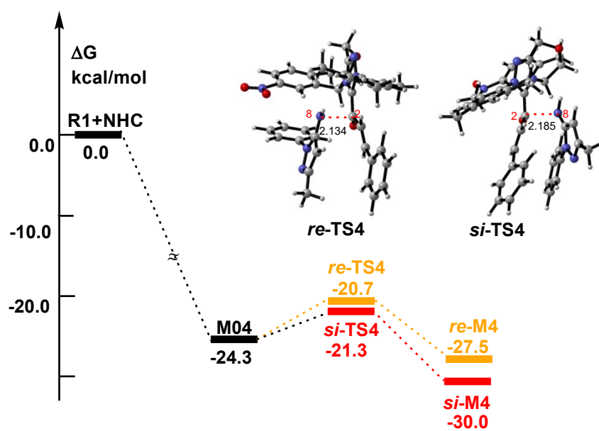
Fig. S5 Free energy profile for 1,2-addition mechanism. Energies and bond distances are in kcal/mol and Å, respectively.
