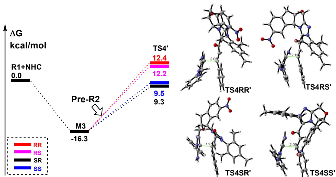
Fig. S8 Free energy profile for the reaction of M3 and Pre-R2 . Energies and bond distances are in kcal/mol and Å, respectively.
