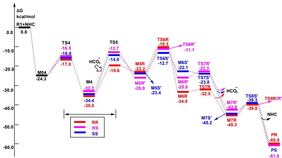
Fig. S6 Free energy profiles of RR/RS/SS-configurational pathways. Energies are in kcal/mol.
