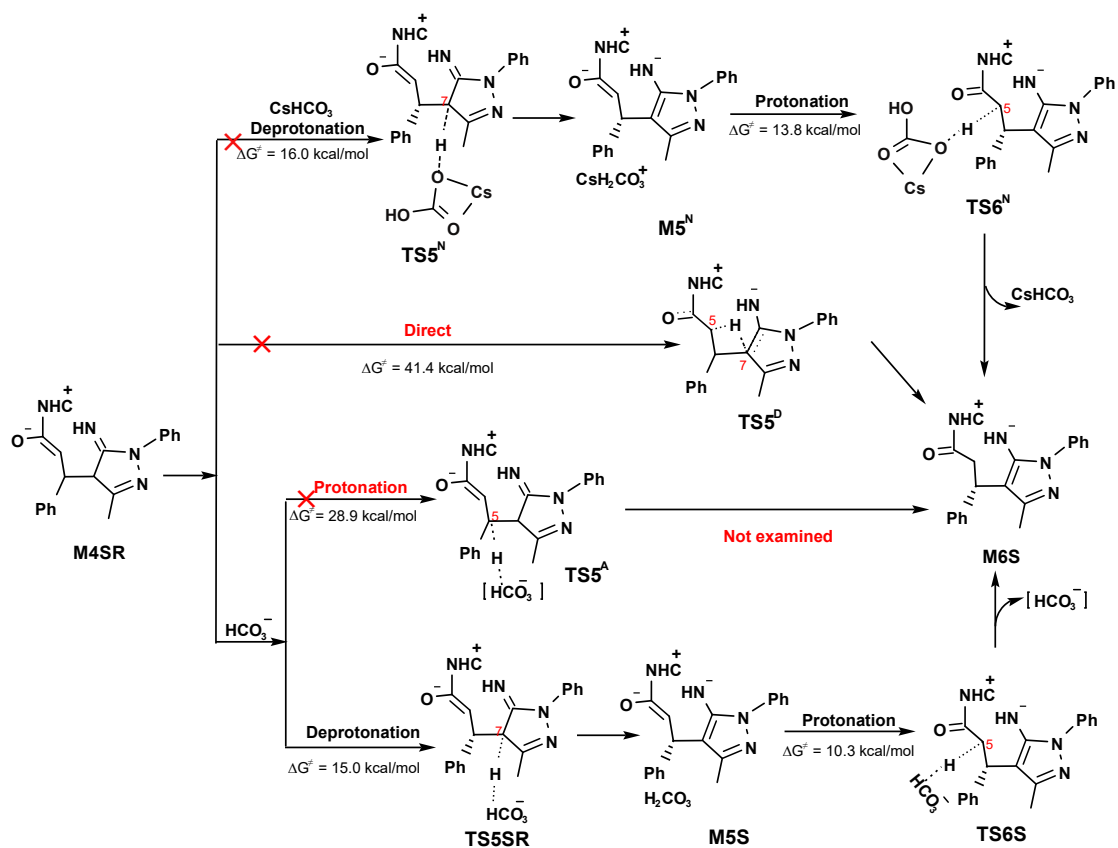
Scheme S3. Proposed pathways for the transformation of M4SR to M6S.
