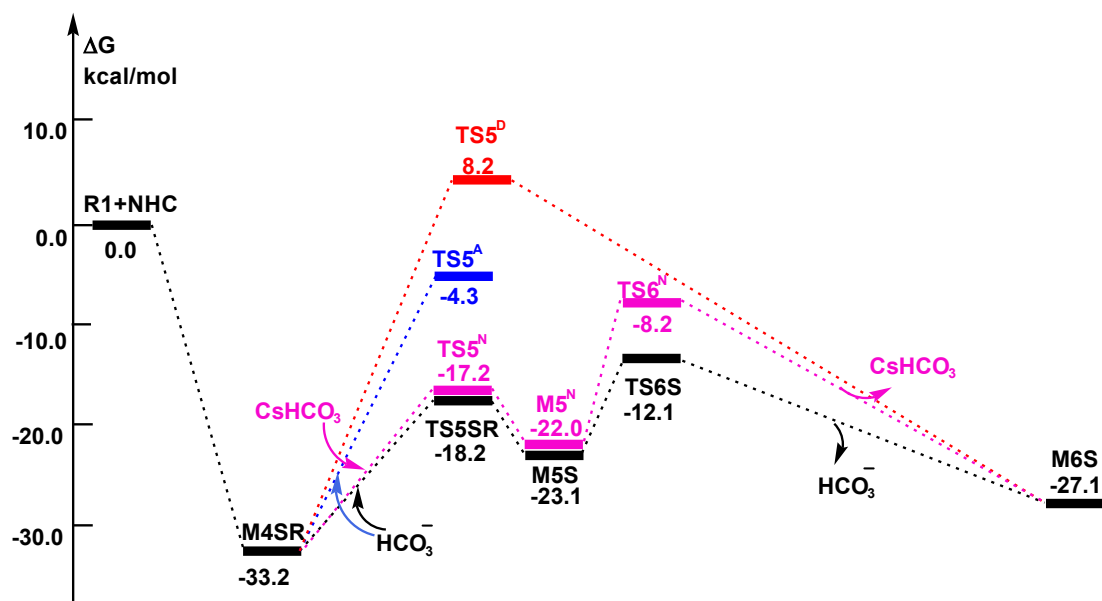
Fig. S9 Free energy (kcal/mol) profile for the transformation of M4SR → M6S . Energies are in kcal/mol.
