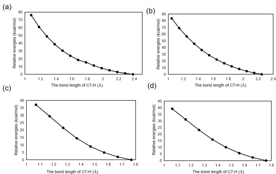
Fig. S7 (a) and (b) Energy change along proton transfer in re -M4 and si -M4, (c) and (d) Energy change along proton transfer in re -M4 and si -M4 in the presence of \text{HCO}_3^- .
