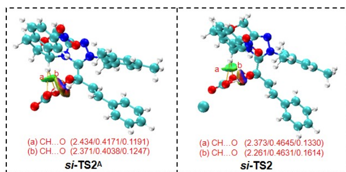
Fig. S4 (b) NCI and AIM analyses for si-TS2 A and si-TS2 . The values in parentheses are distances, Laplacian of electron densities ( \nabla^2\rho ) and electron densities ( \rho_{\text{bcp}} ), which are given in Å, 10^{-1} a.u. and 10^{-1} a.u., respectively.
