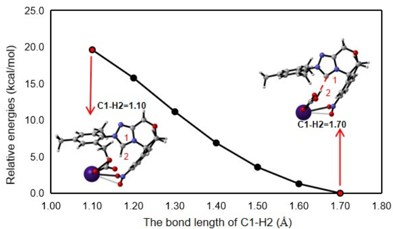
Fig. S1 The deprotonation of NHC precursor by base \text{CsCO}_3^- . Bond distances are in Å.
