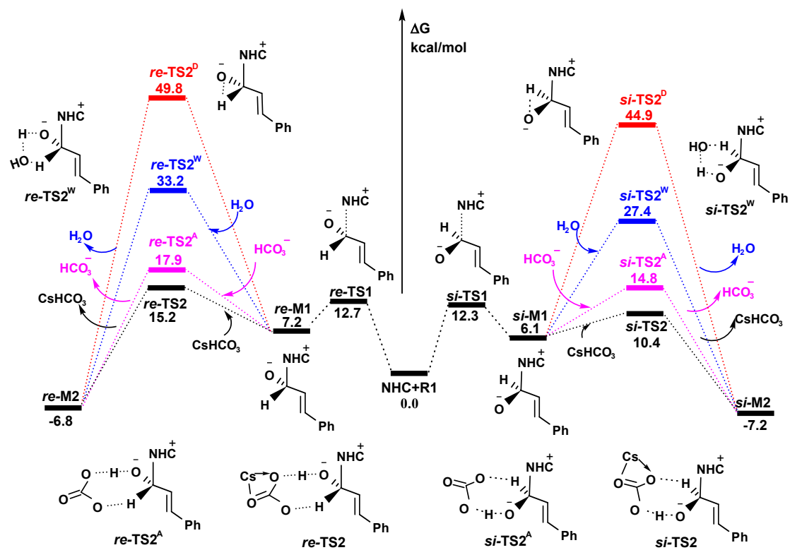
Fig. S3 Free energy (kcal/mol) profile of steps 1 and 2. Energies are in kcal/mol.
