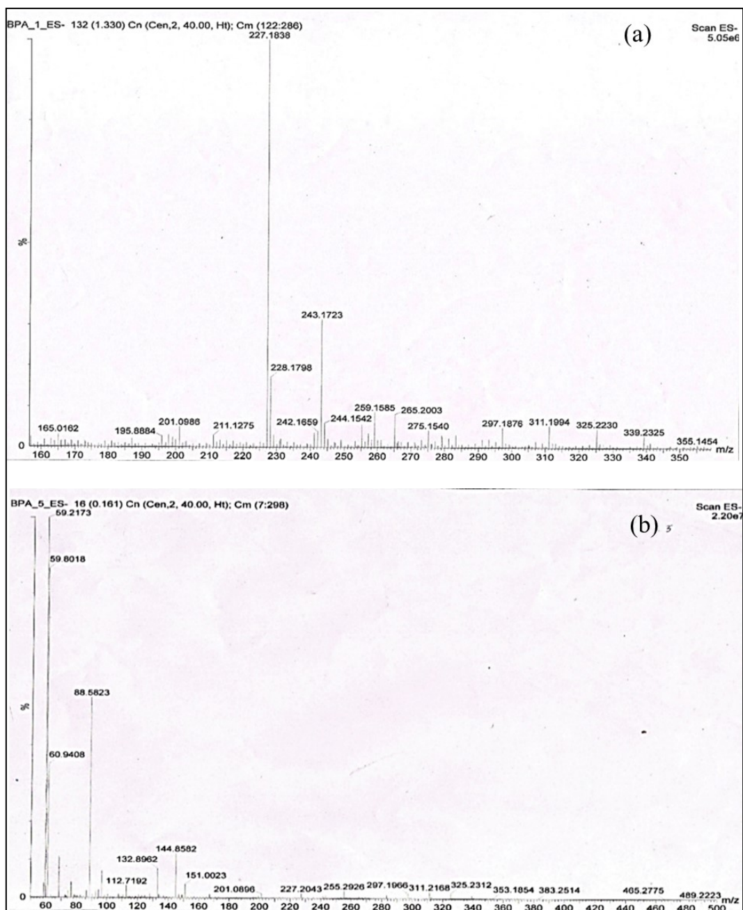
Fig. S2. Mass analysis (a) Mass spectrum of pure BPA solution (b) Mass spectrum of solution after 60 min reaction with \text{MnO}_2 nanosheets.
