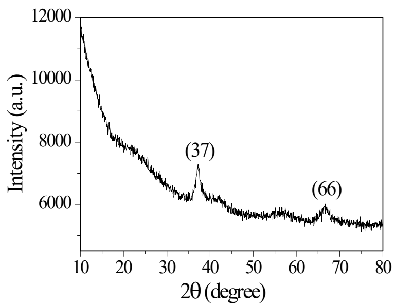
Fig.S1. XRD pattern of the as-prepared nano MnO 2 29
