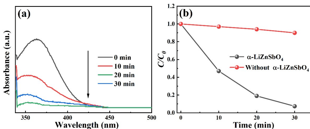
Fig. S2 UV-vis spectral changes of TC solutions, (b) degradation curves of photocatalytic degradation of TC.
