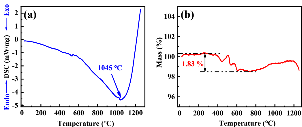
Fig. S1 DSC (a) and TG (b) curves of \text{LiZnSbO}_4 mixture powders.
