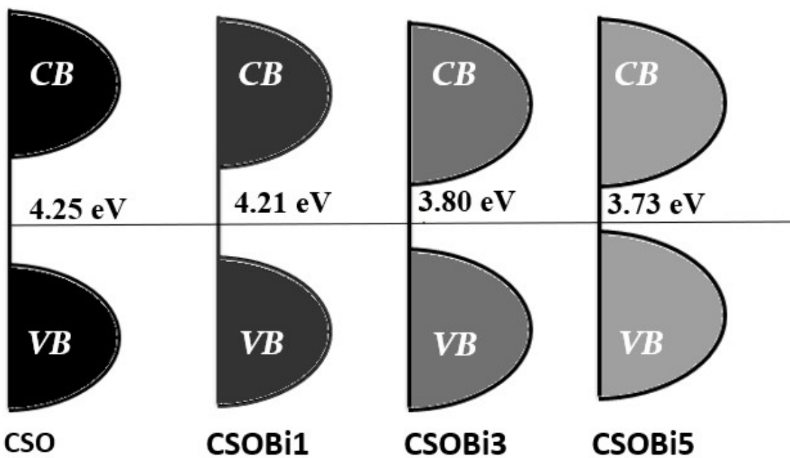
Figure S3: Schematic representation of variation in band gap values of CSO and Bi doped CSO Compounds
