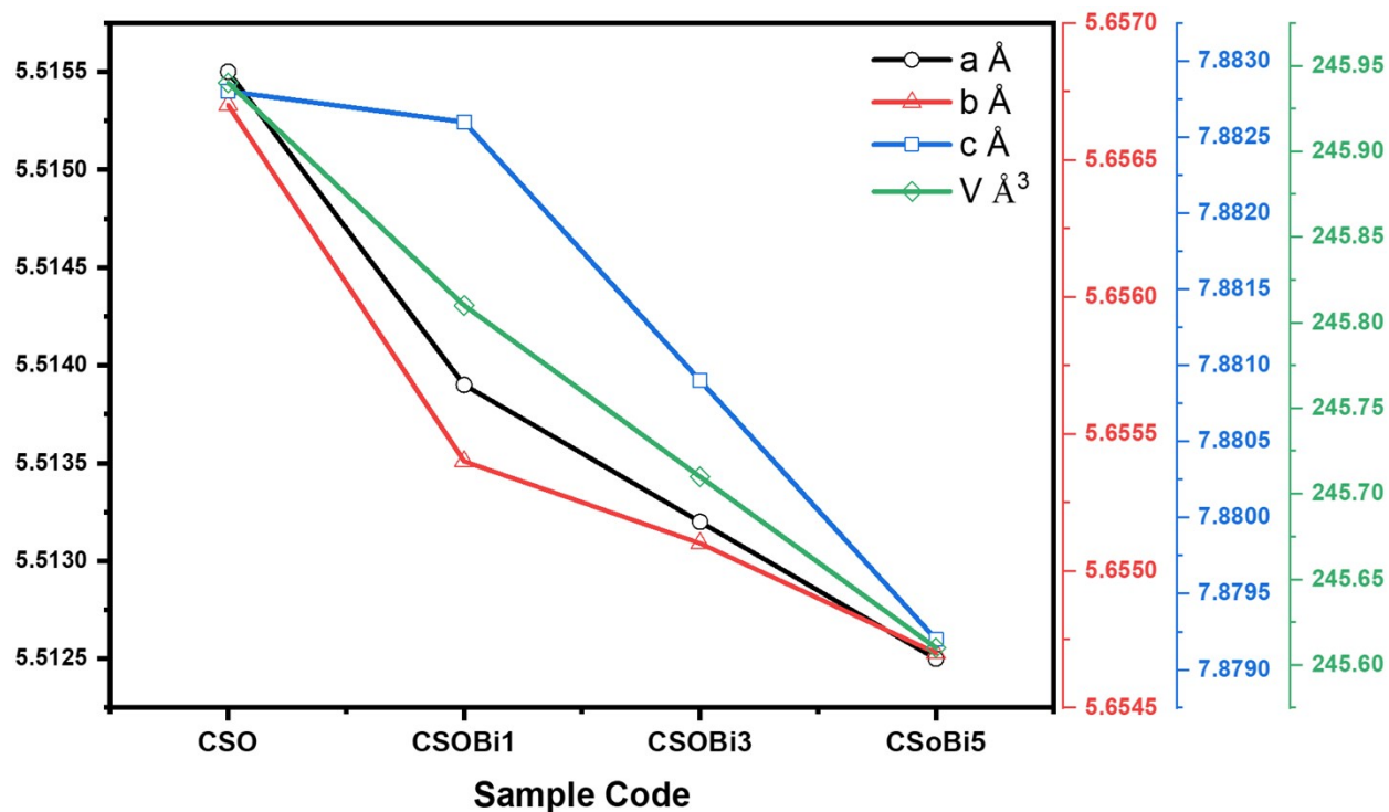
Figure S1: Lattice parameter and unit cell volume of CSO and Bi doped CSO compounds
