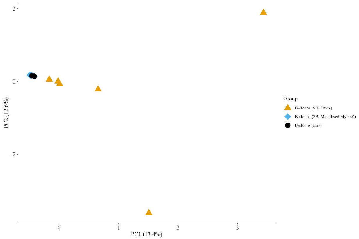
Figure S1: PCA scores plot for environmental balloon samples vs store-bought balloon samples.
