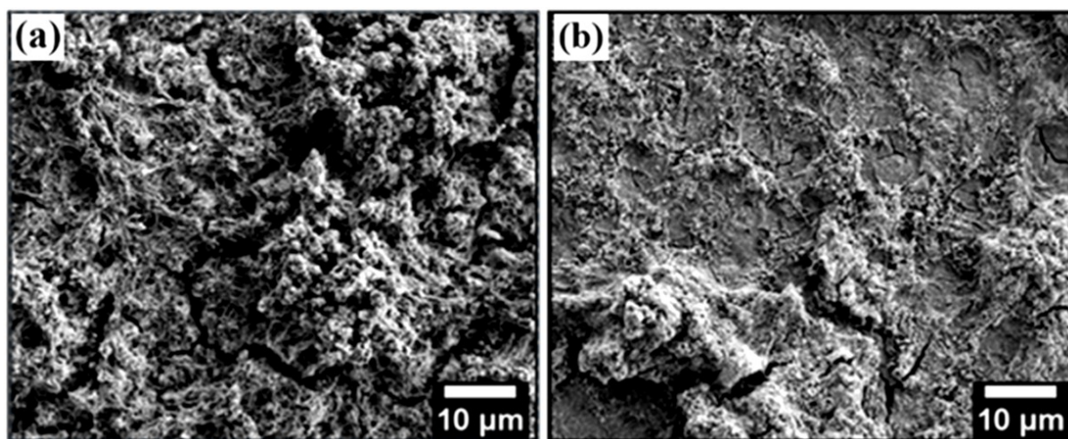
Figure S1. Low magnification SEM micrographs of steel samples after 28 days of immersion in biotic media (a) MB-Lc and (b) MB+Lc media inoculated with SRB.
