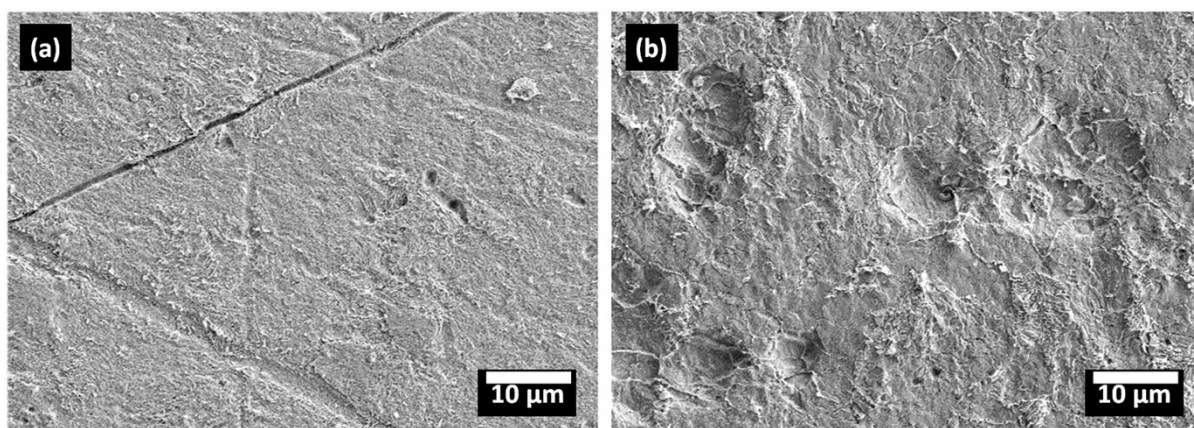
Figure S2. SEM micrographs of cleaned steel sample surfaces outside pit regions after 28-day immersion in biotic media (a) MB-Lc and (b) MB+Lc inoculated with SRB.
