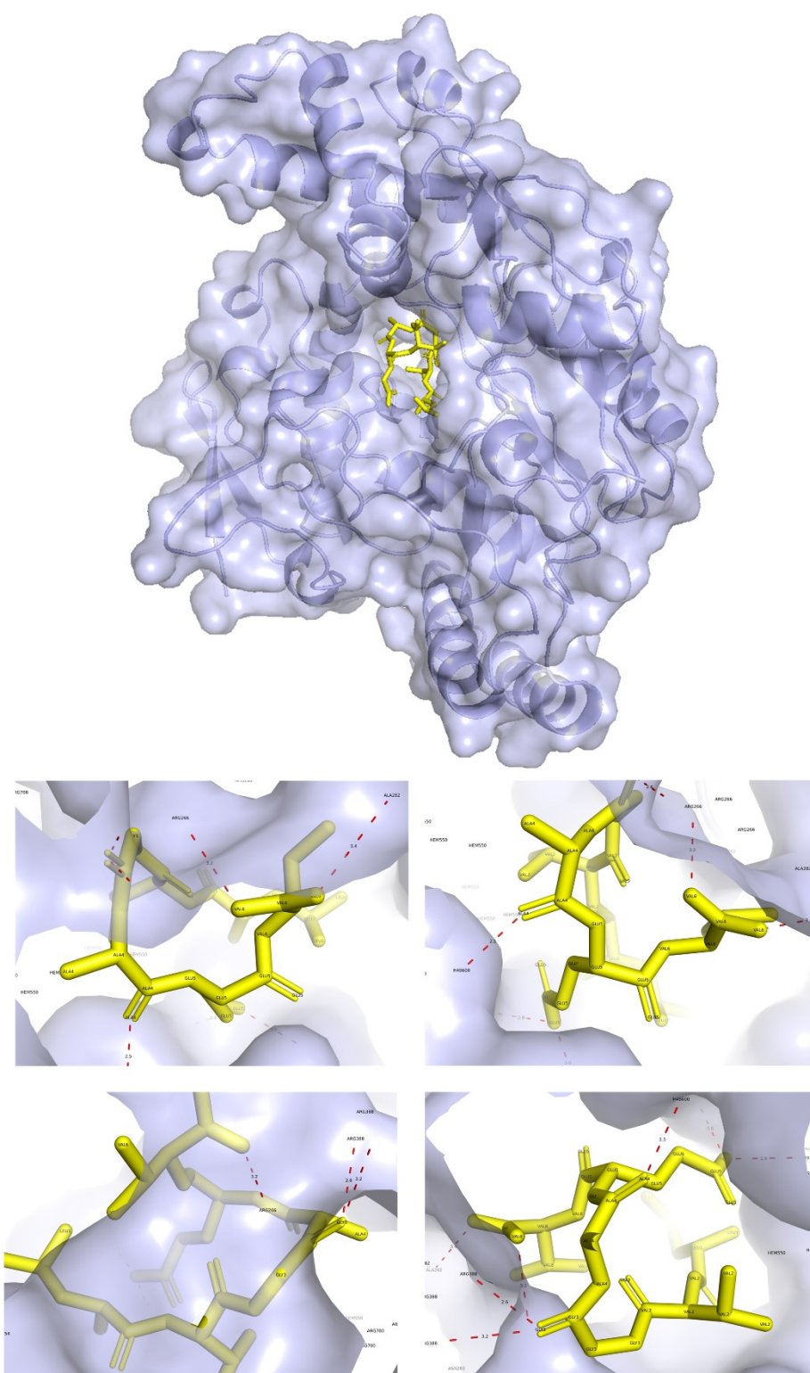
Supplementary Figure S1. Molecular docking analysis of the interaction between 1NSI and the LVGAEV peptide. Interactions and hydrogen bonds between amino acids in LVGAEV and 1NSI are illustrated.
