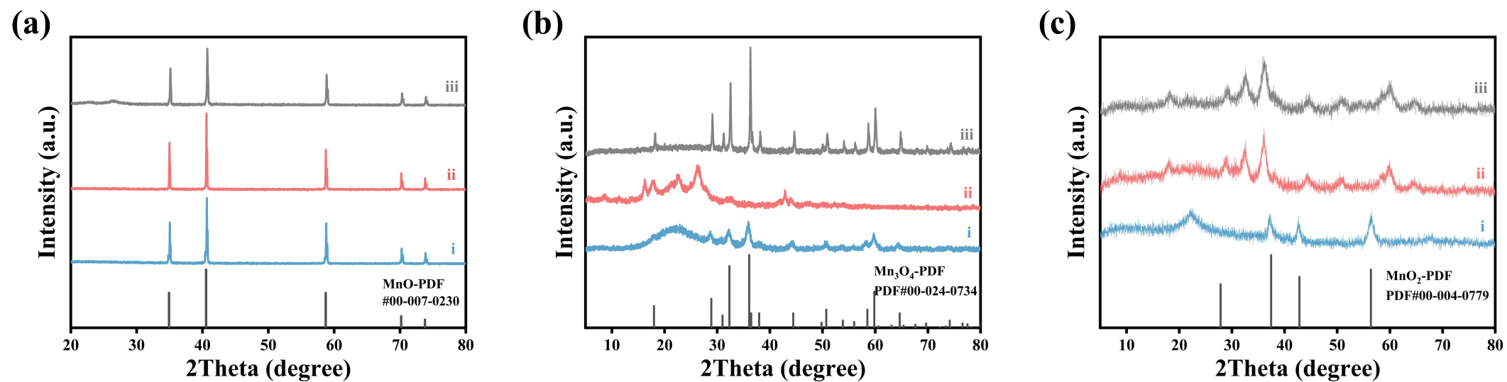
Figure. S17. XRD patterns of (a) MnO (b) Mn 3 O 4 (c) MnO 2 before and after reaction.
