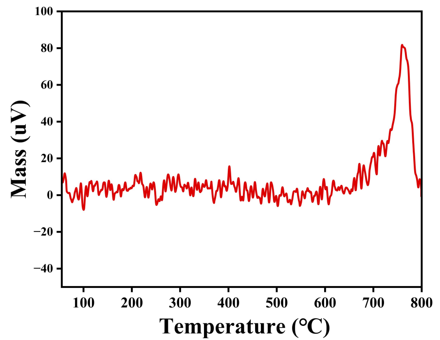
Figure. S19. CO 2 -TPD spectra of Mn 2 O 3 .
