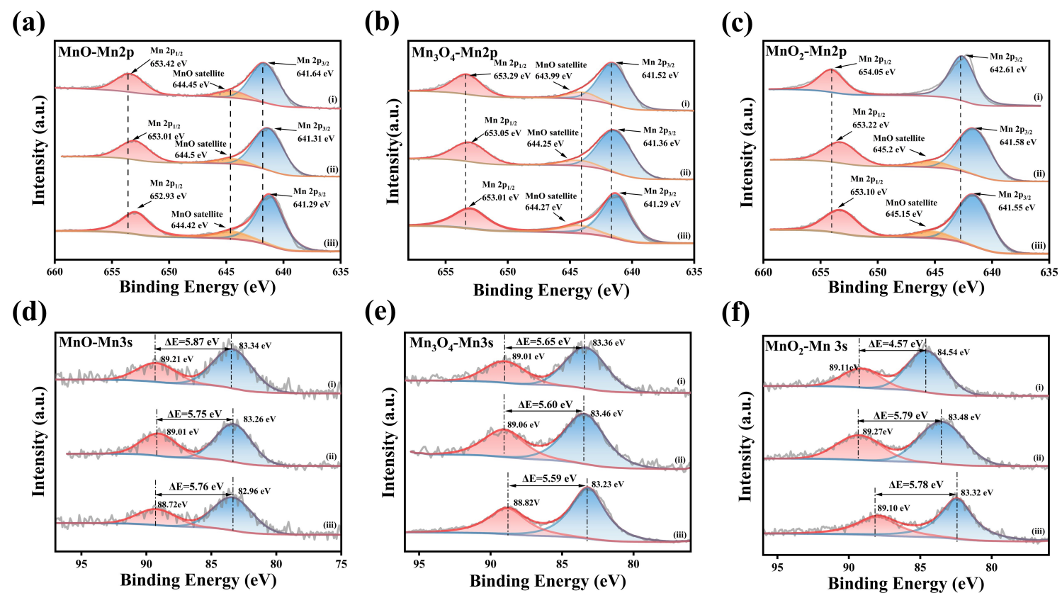
Figure. S21. XPS curves of Mn 2p: (a) MnO (b) Mn 3 O 4 (c) MnO 2 , and Mn 3s: (d) MnO (e) Mn 3 O 4 (f) MnO 2 . ((i) before reaction, (ii) after heterogeneous reaction, (iii) after synergistic reaction).
